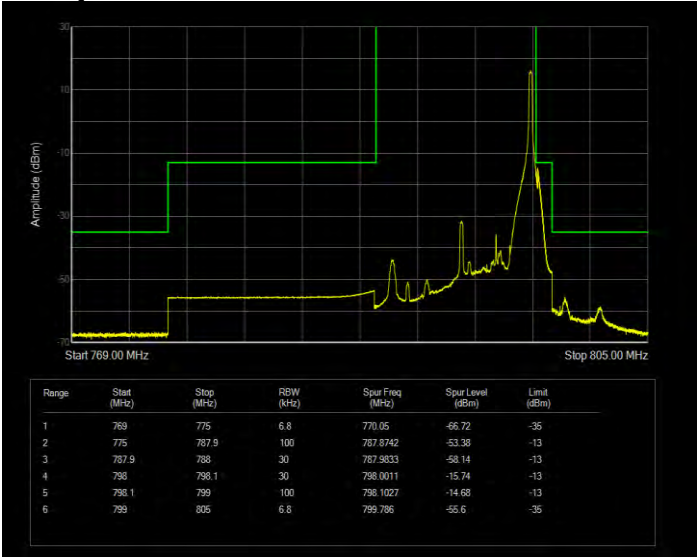
Band14 16QAM BW=5MHz Channel=23355 RB Size=25 Position=#0 Extended
