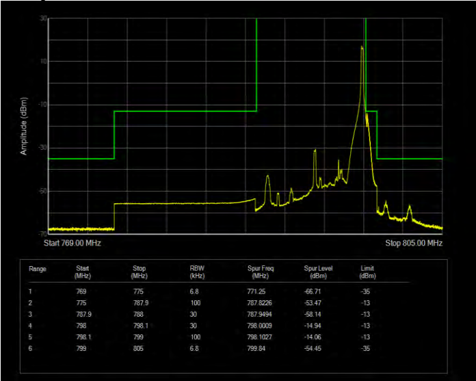
Band14 QPSK BW=5MHz Channel=23355 RB Size=25 Position=#0 Extended
