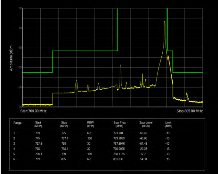
Band14 QPSK BW=10MHz Channel=23330 RB Size=50 Position=#0 Extended
