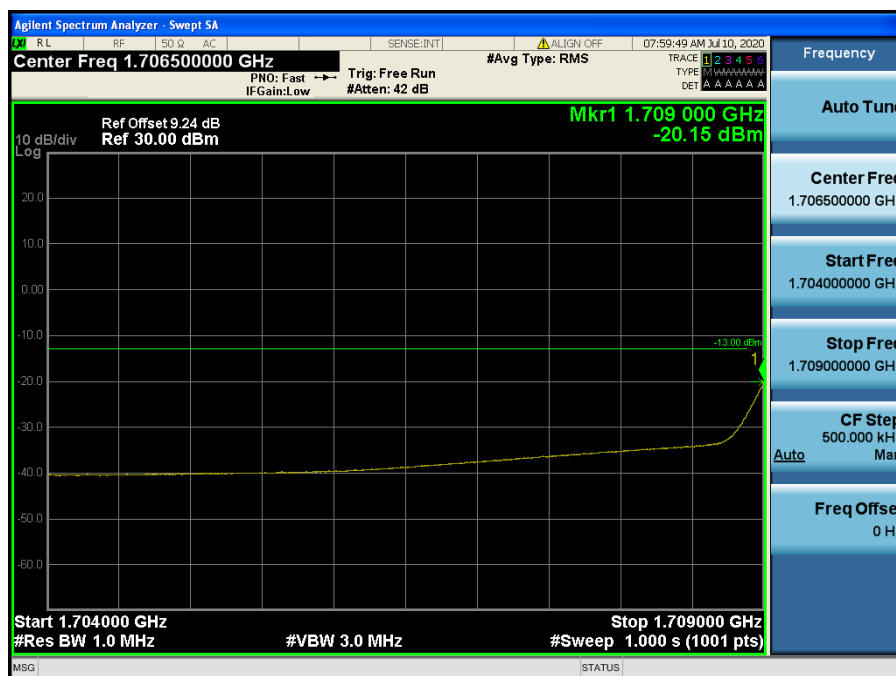
LTE Band 4 / 1.4 MHz / 16QAM - RB Size/Offset (1/2)
