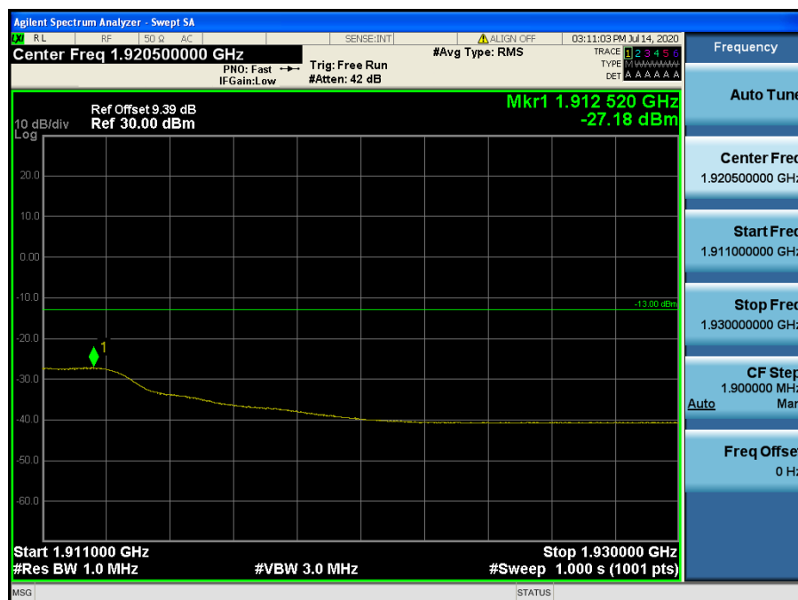
LTE Band 2 / 20 MHz / QPSK - RB Size/Offset (50/25)
