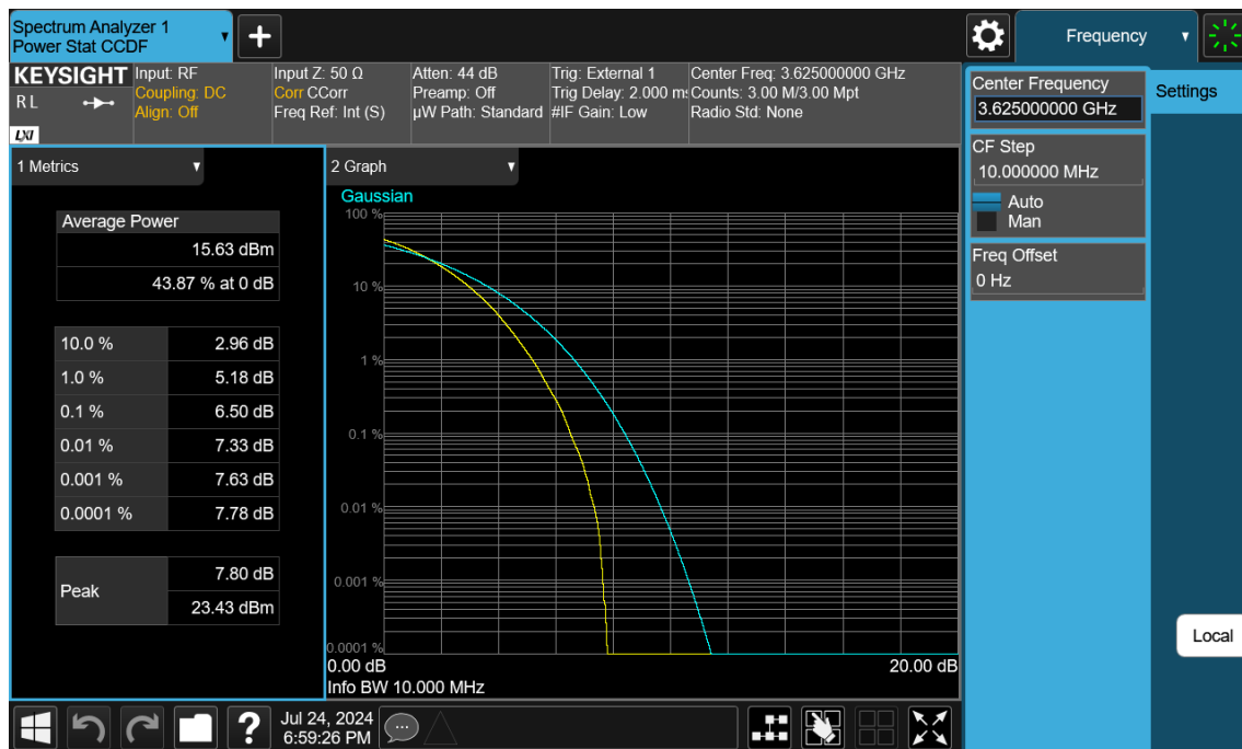
10 MHz / 256QAM / FULL RB Size
