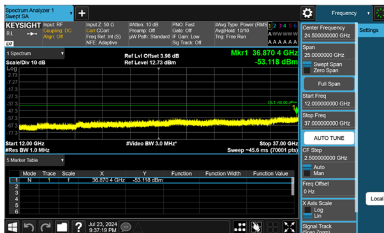
20 MHz / QPSK / RB Size/Offset (1/0) - Low Channel
