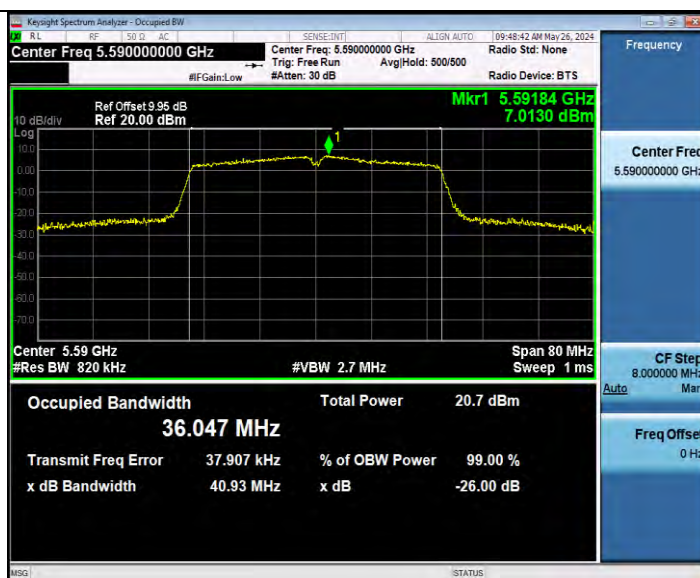
11N40MIMO Ant2 5590
