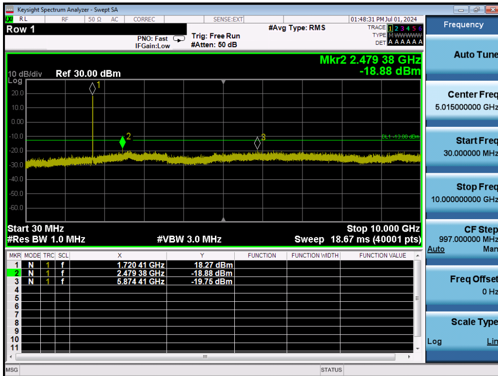
LTE Band 66 / 20MHz / 64QAM - RB Size/Offset (50/25) - Low Channel
