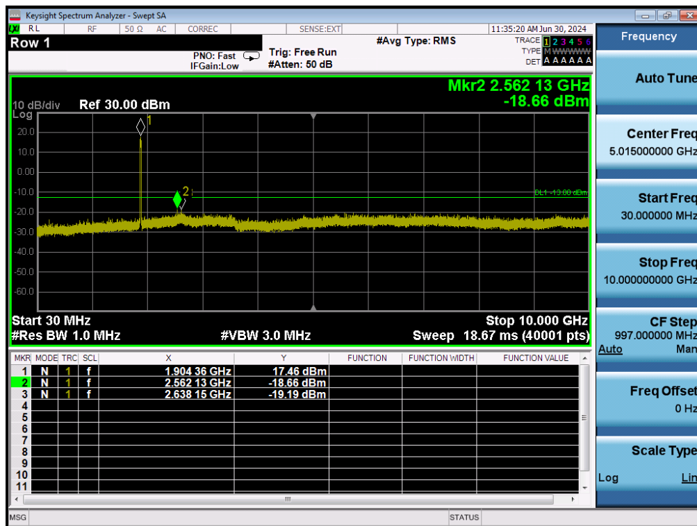
LTE Band 2 / 20MHz / 16QAM -- RB Size/Offset (100/0) - High Channel
