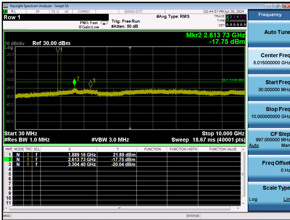
LTE Band 2 / 20MHz / 256QAM - RB Size/Offset (1/99) - Mid Channel
