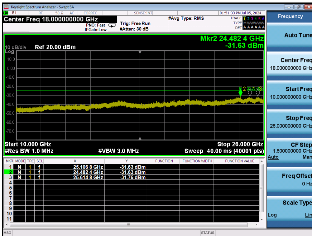
LTE Band 7 / 20MHz / 256QAM - RB Size/Offset (50/0) - Low Channel
