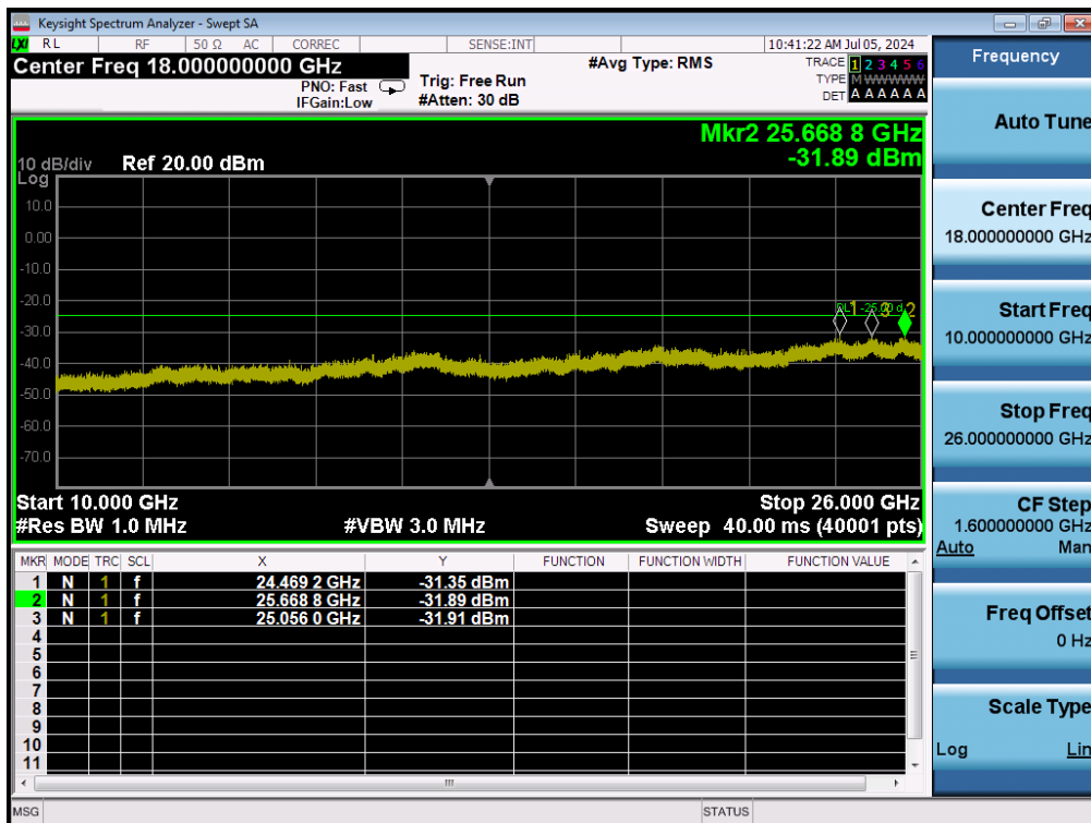
LTE Band 7 / 20MHz / QPSK -- RB Size/Offset (50/50) - High Channel
