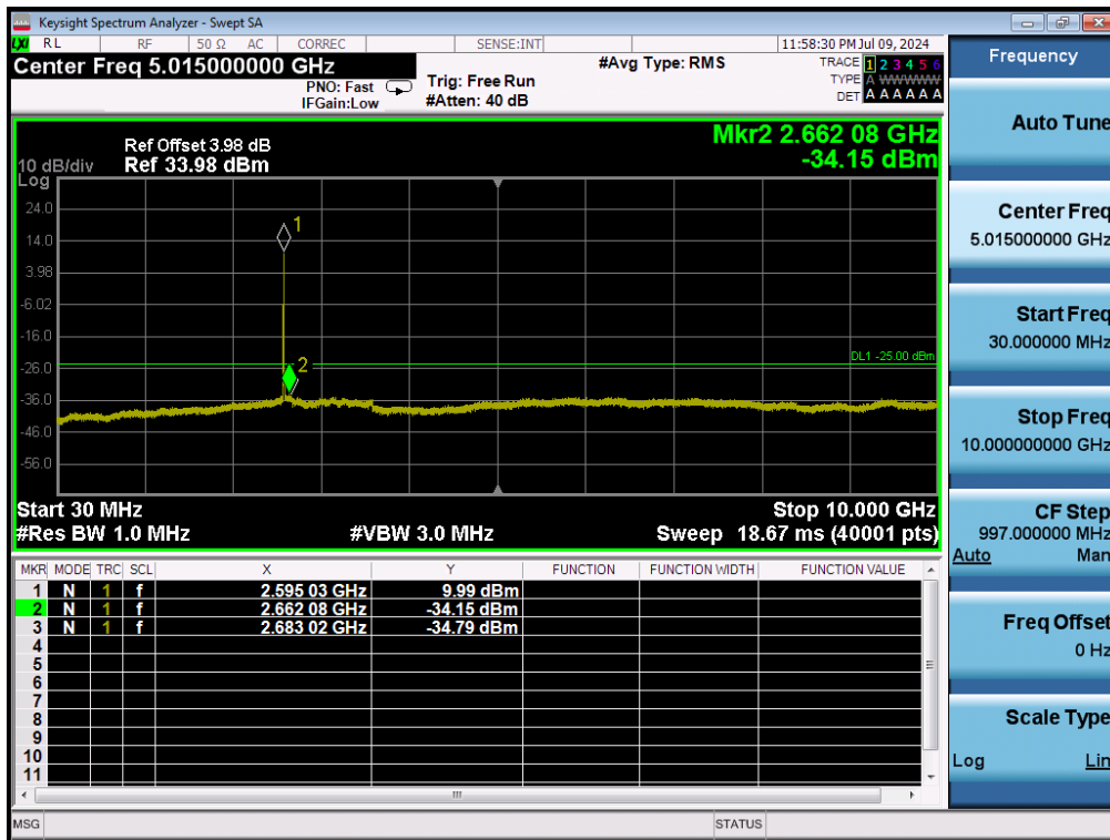
LTE Band 38 / 20MHz / 256QAM - RB Size/Offset (50/25) - Mid Channel
