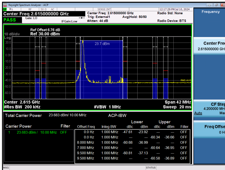
LTE Band 38 / 10MHz / QPSK - RB Size/Offset (1/0)
