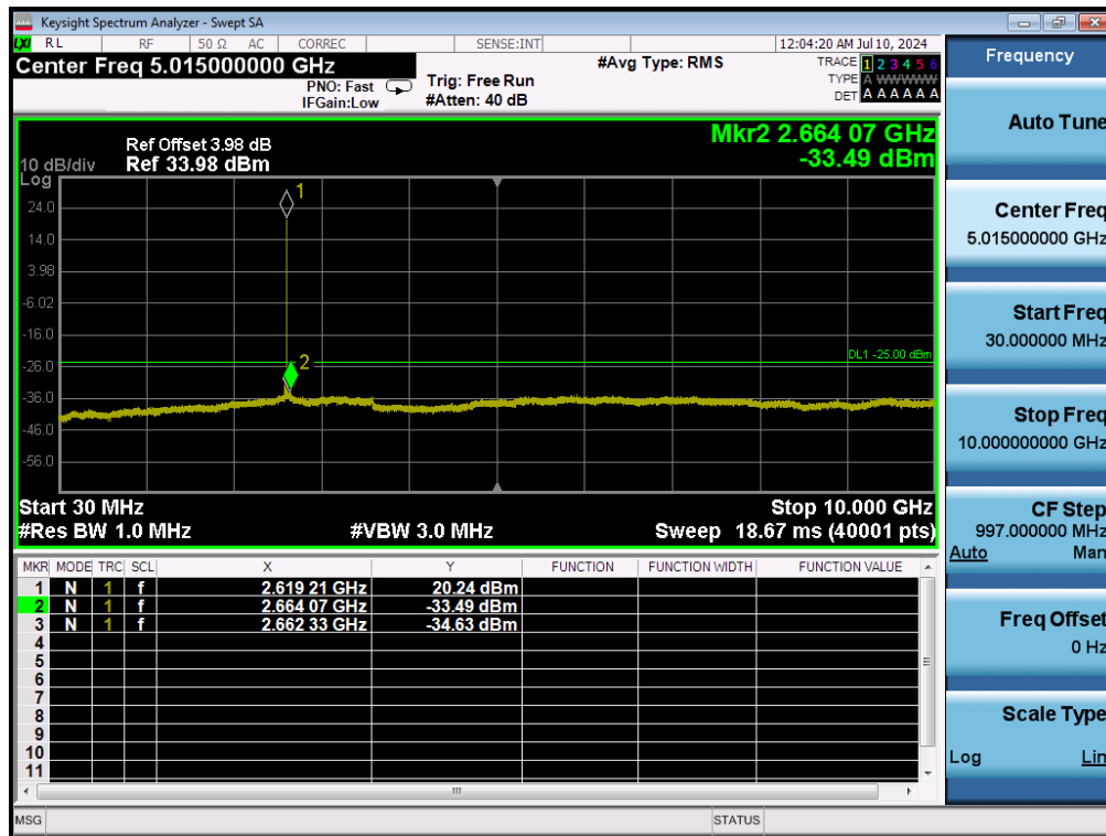
LTE Band 38 / 20MHz / 256QAM - RB Size/Offset (1/99) - High Channel
