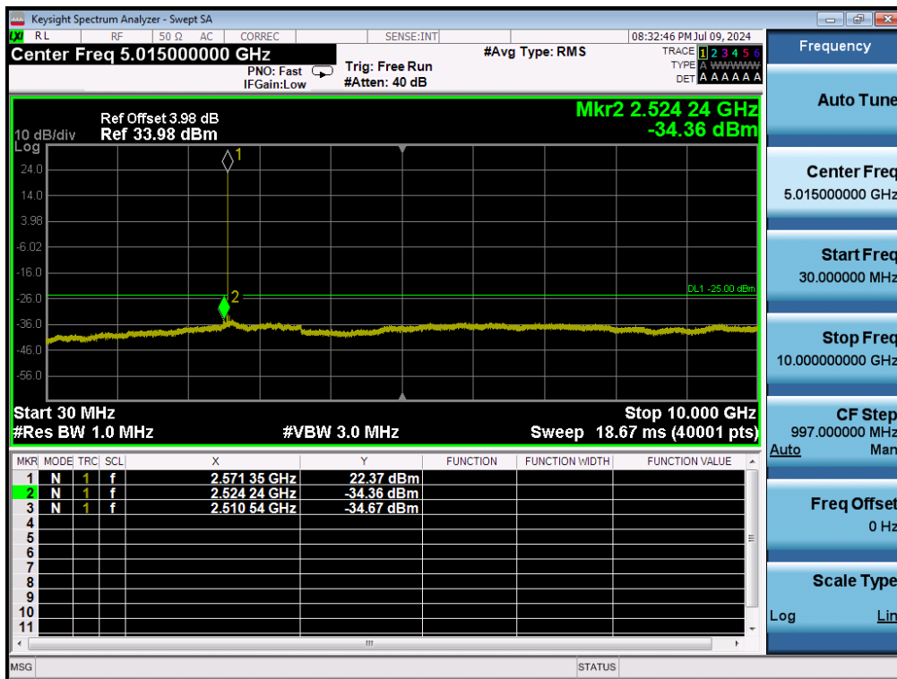
LTE Band 38 / 20MHz / 16QAM - RB Size/Offset (1/0) - Low Channel
