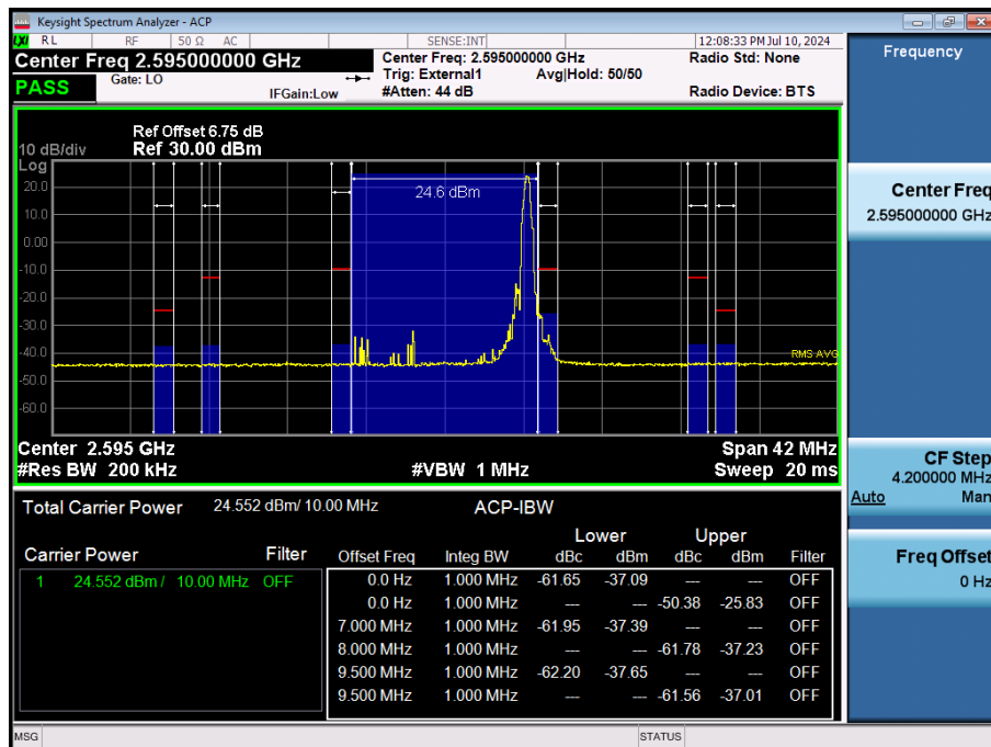
LTE Band 38 / 10MHz / QPSK - RB Size/Offset (1/49)
