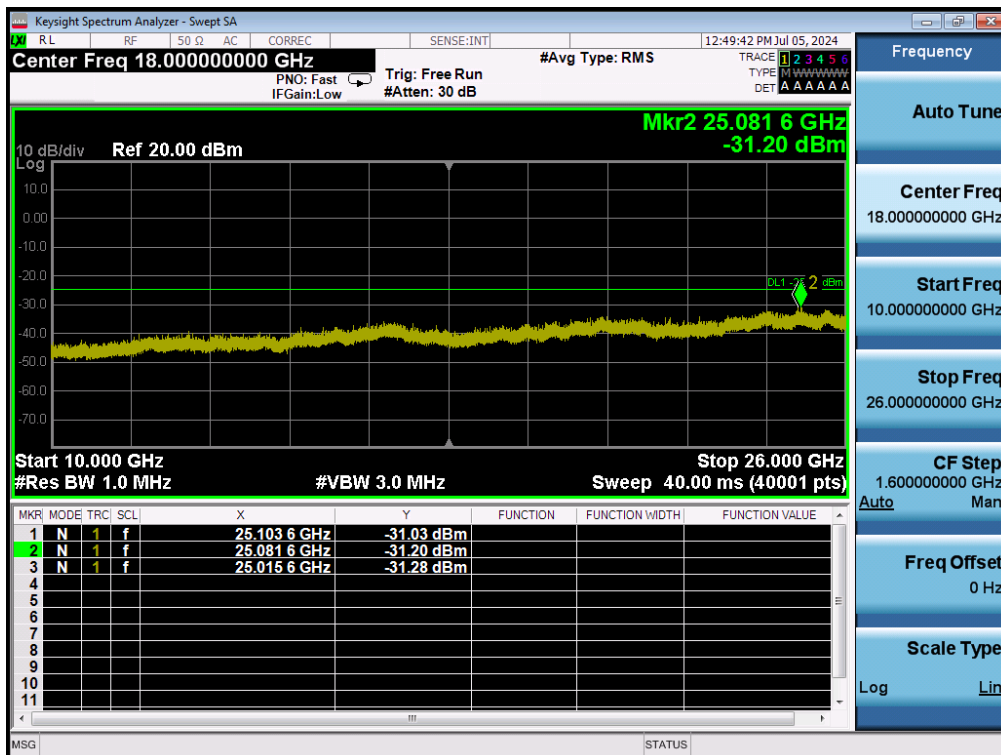
LTE Band 7 / 20MHz / 256QAM - RB Size/Offset (50/0) - Mid Channel
