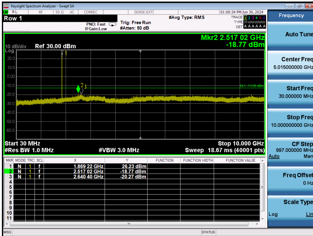
LTE Band 2 / 20MHz / 64QAM - RB Size/Offset (1/99) - Low Channel
