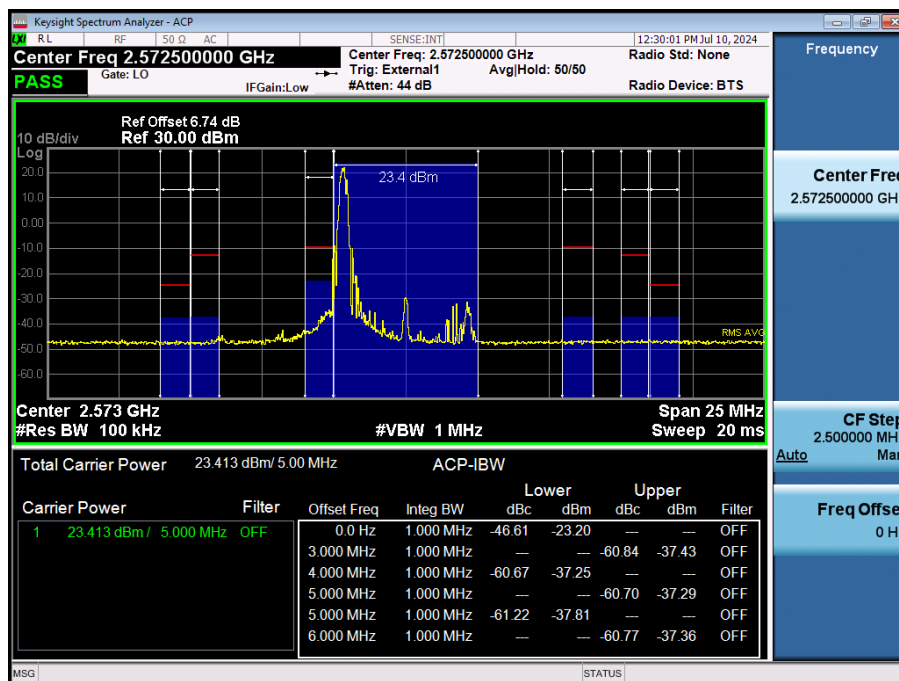
LTE Band 38 / 5MHz / QPSK - RB Size/Offset (1/0)
