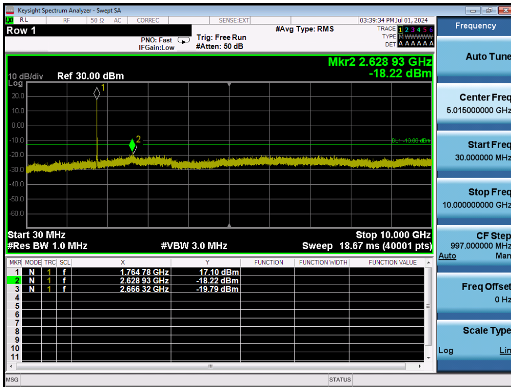
LTE Band 66 / 20MHz / 64QAM -- RB Size/Offset (50/0) - High Channel
