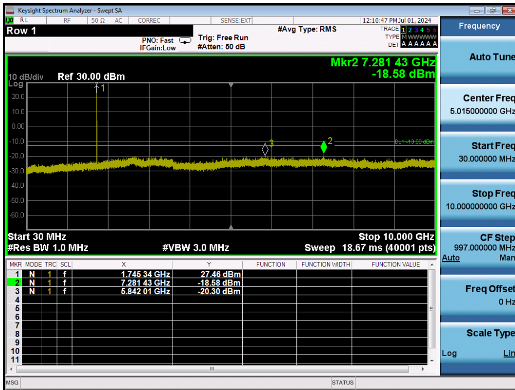
LTE Band 66 / 20MHz / 16QAM - RB Size/Offset (1/50) - Mid Channel
