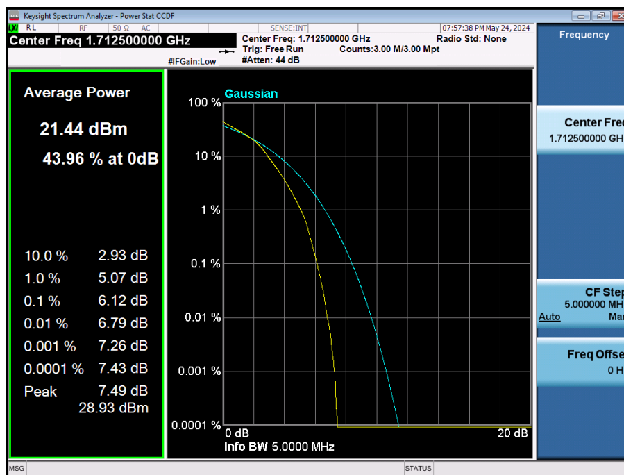
LTE Band 66 / 5 MHz / 16QAM / FULL RB Size
