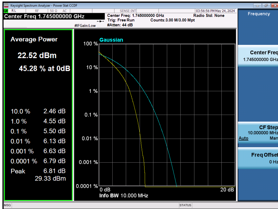
LTE Band 66 / 10 MHz / QPSK / FULL RB Size
