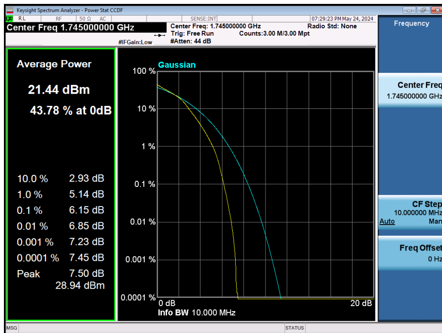
LTE Band 66 / 10 MHz / 16QAM / FULL RB Size
