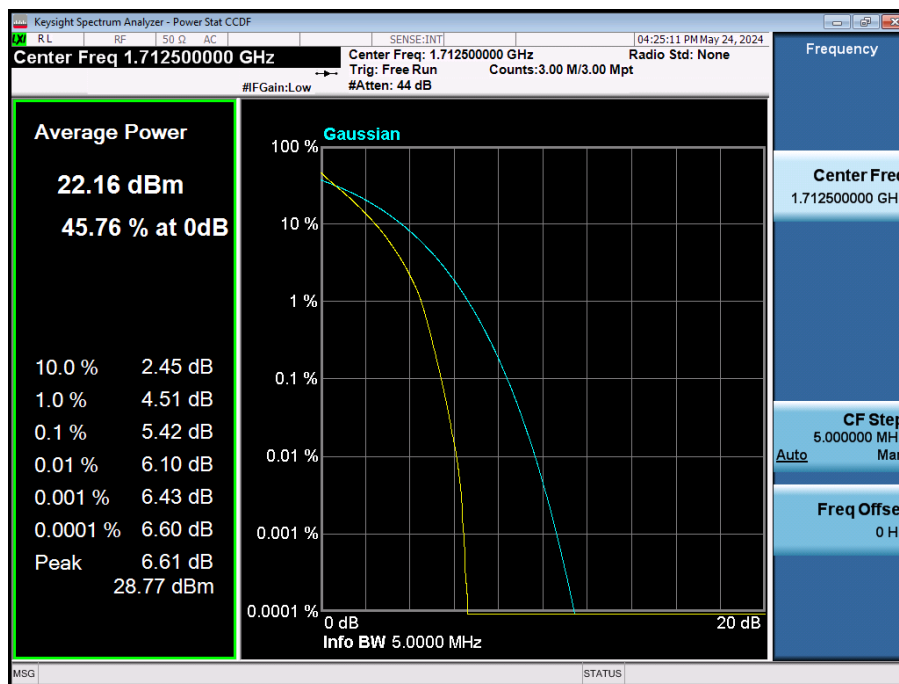
LTE Band 66 / 5 MHz / QPSK / FULL RB Size
