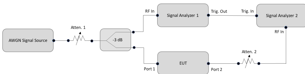
Figure 2. Contention-based protocol test setup conducted method
