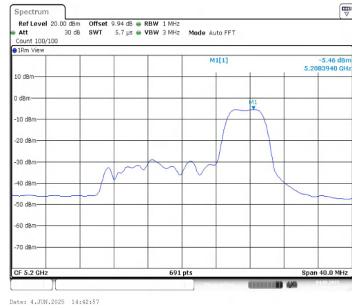
11AX20MIMO-Ant1-5200-52Tone-RU40-PASS
