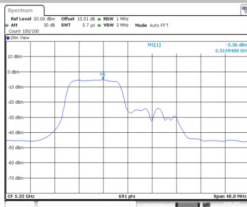
11AX20MIMO-Ant2-5320-52Tone-RU40-PASS
