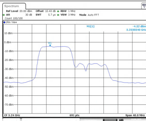
11AX20MIMO-Ant1-5240-52Tone-RU40-PASS
