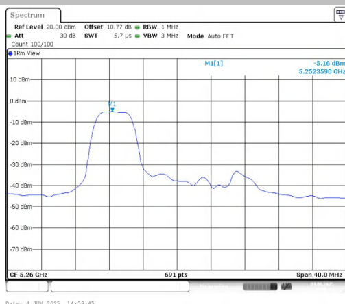
11AX20MIMO-Ant1-5260-52Tone-RU37-PASS
