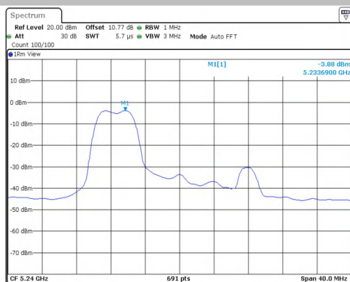
11AX20MIMO-Ant1-5240-26Tone-RU8-PASS
