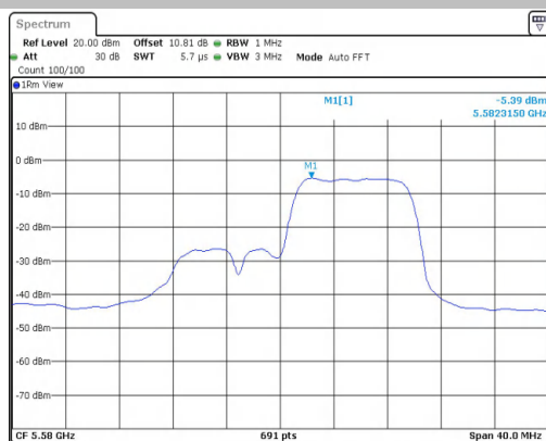
11AX20MIMO-Ant1-5580-106Tone-RU53-PASS
