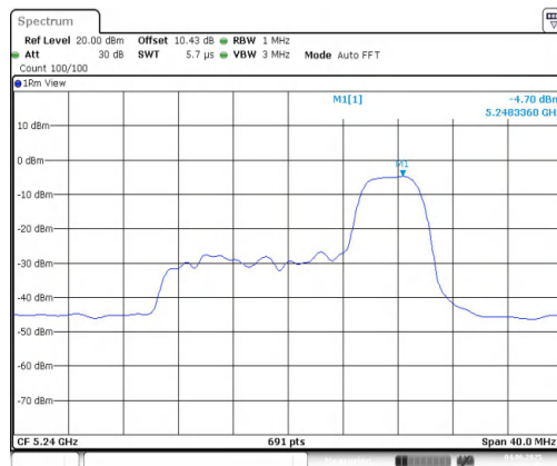
11AX20MIMO-Ant2-5240-52Tone-RU40-PASS
