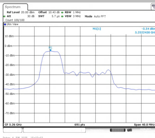
11AX20MIMO-Ant2-5260-52Tone-RU37-PASS
