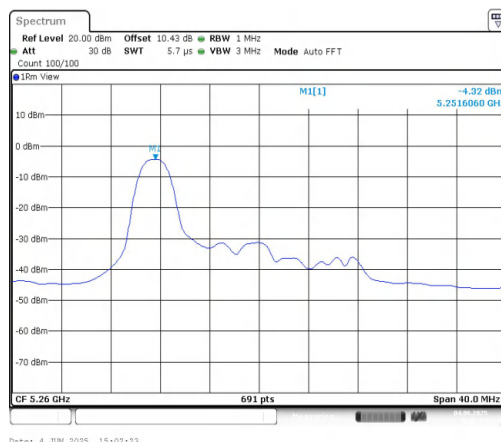
11AX20MIMO-Ant2-5260-26Tone-RU0-PASS
