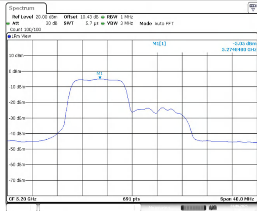
11AX20MIMO-Ant2-5280-52Tone-RU40-PASS
