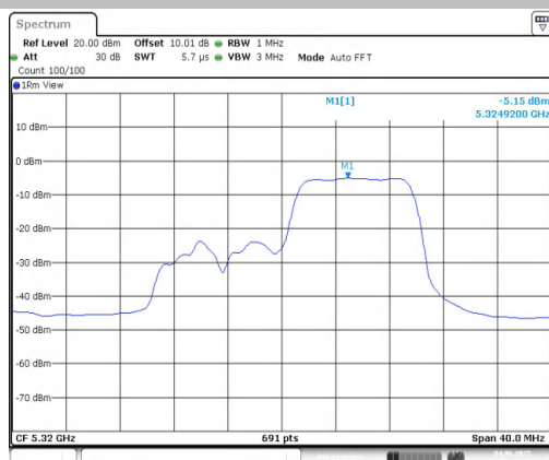
11AX20MIMO-Ant1-5320-106Tone-RU53-PASS
