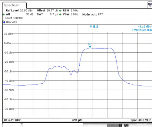
11AX20MIMO-Ant1-5280-106Tone-RU53-PASS
