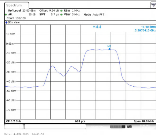
11AX20MIMO-Ant1-5200-106Tone-RU54-PASS
