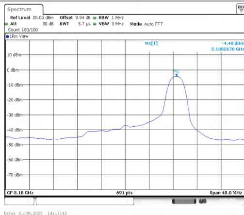
11AX20MIMO-Ant1-5180-26Tone-RU8-PASS
