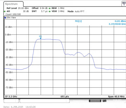
11AX20MIMO-Ant1-5200-106Tone-RU53-PASS
