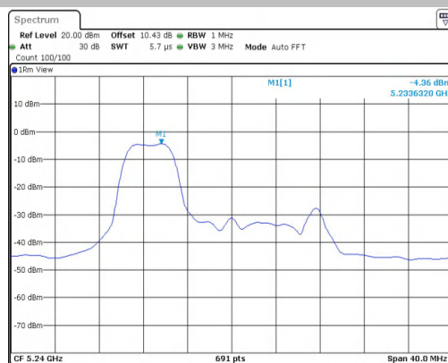
11AX20MIMO-Ant2-5240-26Tone-RU8-PASS
