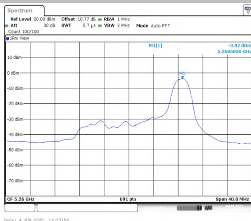
11AX20MIMO-Ant1-5260-26Tone-RU8-PASS
