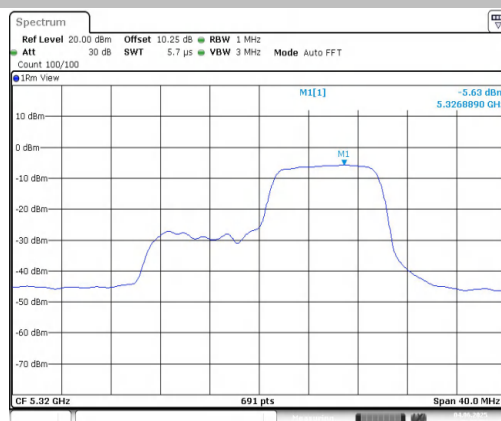
11AX20MIMO-Ant2-5320-106Tone-RU53-PASS
