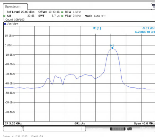
11AX20MIMO-Ant2-5260-26Tone-RU8-PASS
