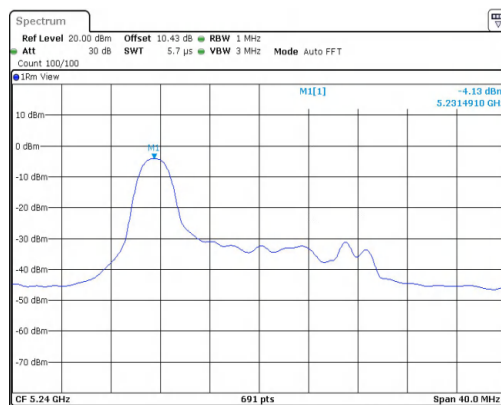
11AX20MIMO-Ant2-5240-26Tone-RU0-PASS
