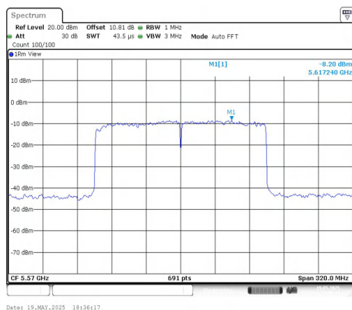
11AX160MIMO-Ant1-5570-PASS
