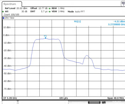
11AX20MIMO-Ant1-5280-52Tone-RU40-PASS
