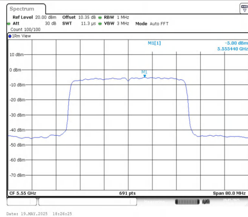
11AX40MIMO-Ant2-5550-PASS
