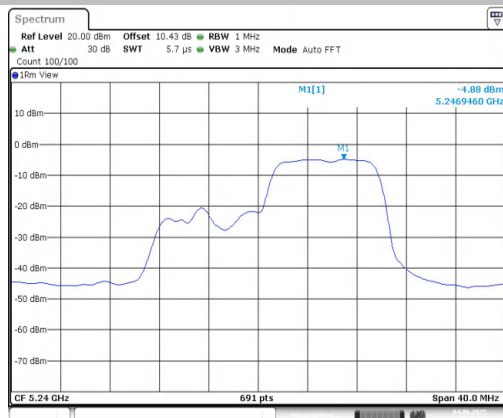
11AX20MIMO-Ant2-5240-106Tone-RU53-PASS
