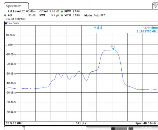
11AX20MIMO-Ant2-5180-52Tone-RU40-PASS
