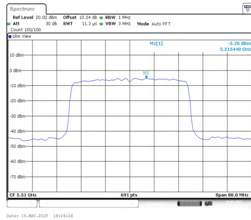
11AX40MIMO-Ant2-5510-PASS
