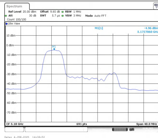
11AX20MIMO-Ant2-5180-52Tone-RU37-PASS
