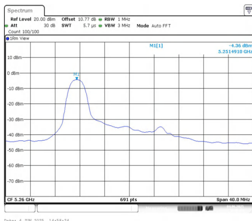
11AX20MIMO-Ant1-5260-26Tone-RU0-PASS
