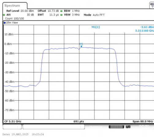
11AX40MIMO-Ant1-5510-PASS
