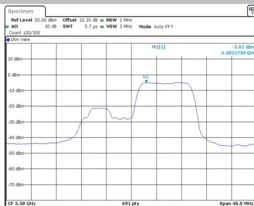
11AX20MIMO-Ant2-5580-106Tone-RU53-PASS
