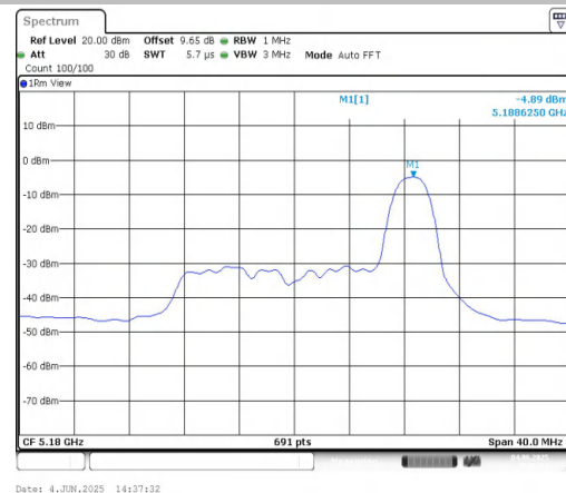
11AX20MIMO-Ant2-5180-26Tone-RU8-PASS
