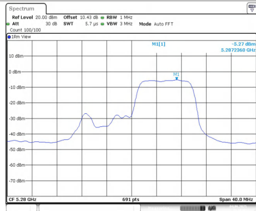
11AX20MIMO-Ant2-5280-106Tone-RU53-PASS
