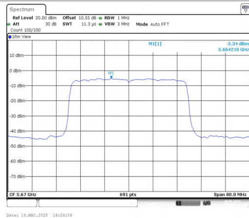
11AX40MIMO-Ant2-5670-PASS
