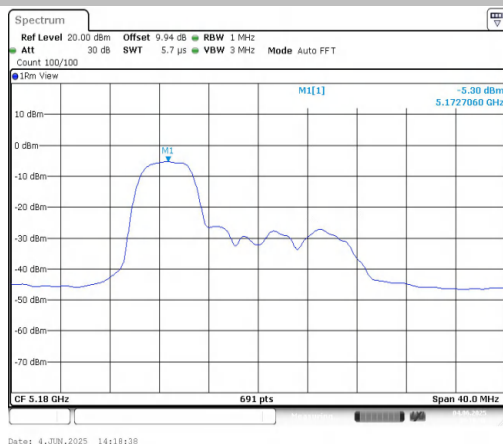
11AX20MIMO-Ant1-5180-52Tone-RU37-PASS
