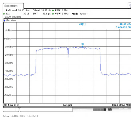
11AX160MIMO-Ant2-5570-PASS
