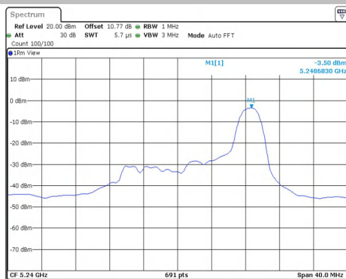
11AX20MIMO-Ant1-5240-26Tone-RU0-PASS
