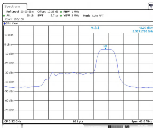
11AX20MIMO-Ant1-5320-52Tone-RU40-PASS
