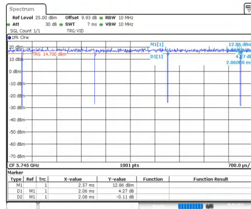
NTNV-11A-CDD-Ant2-5745
