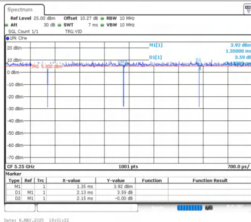
NTNV-11AC160MIMO-Ant1-5250
