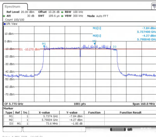
11AC80MIMO-Ant1-5775-PASS
