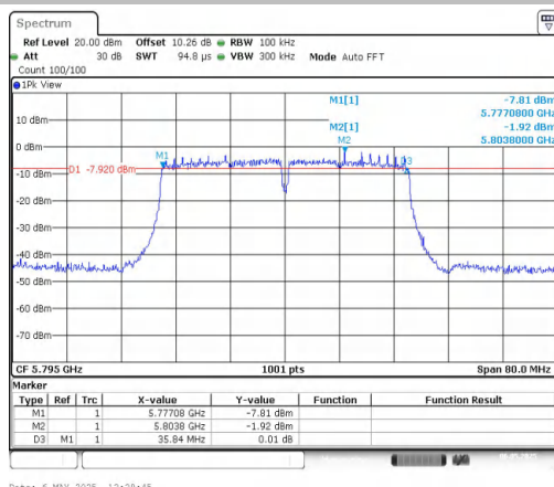
11AC40MIMO-Ant1-5795-PASS
