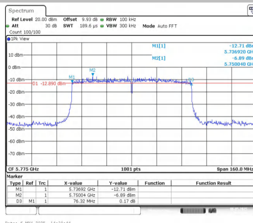
11AC80MIMO-Ant2-5775-PASS
