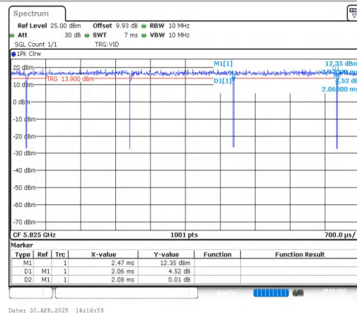
NTNV-11A-CDD-Ant2-5825
