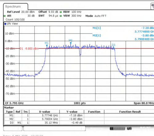
11AC40MIMO-Ant2-5795-PASS
