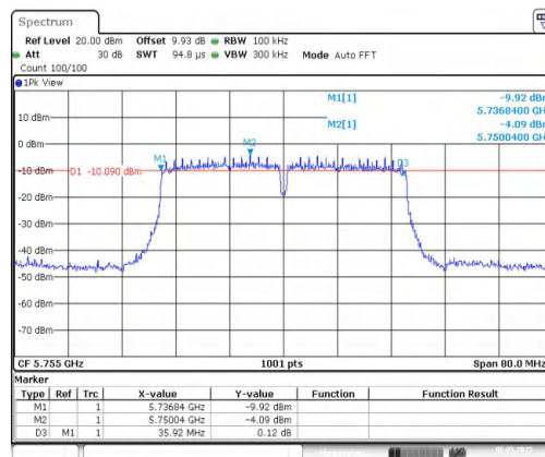
11AC40MIMO-Ant2-5755-PASS
