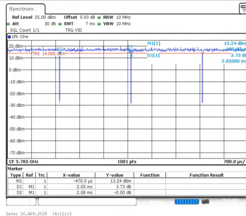
NTNV-11A-CDD-Ant2-5785
