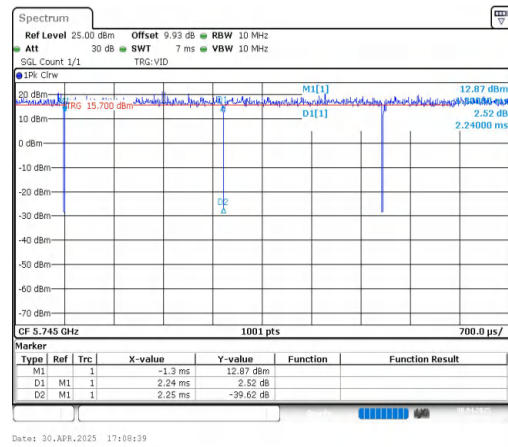
NTNV-11AC20MIMO-Ant2-5745
