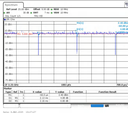
NTNV-11AC160MIMO-Ant2-5250
