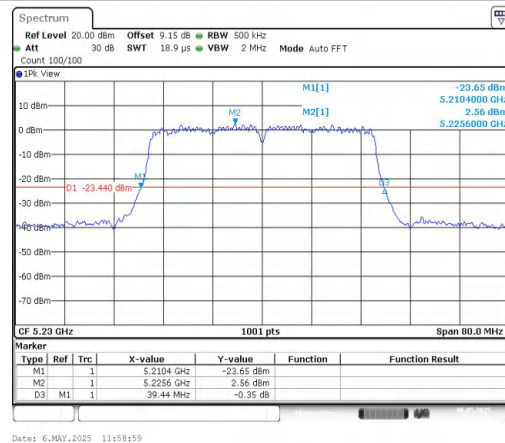
11AC40MIMO-Ant2-5230
