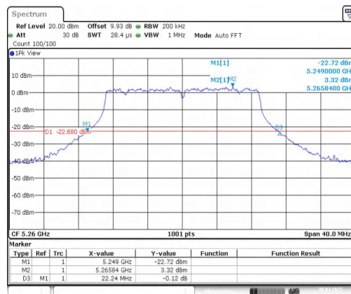
11AC20MIMO-Ant2-5260
