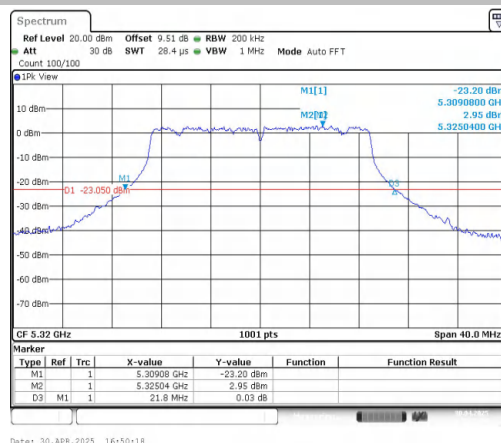
11AC20MIMO-Ant2-5320
