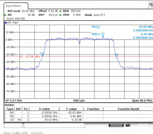
11AC40MIMO-Ant2-5270
