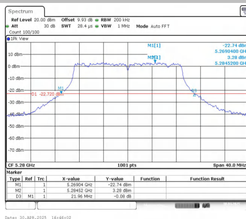
11AC20MIMO-Ant2-5280
