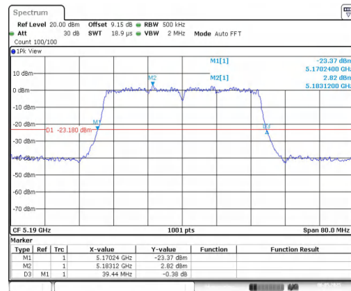
11AC40MIMO-Ant2-5190
