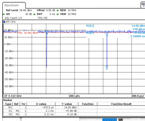
NTNV-11G-CDD-Ant1-2412
