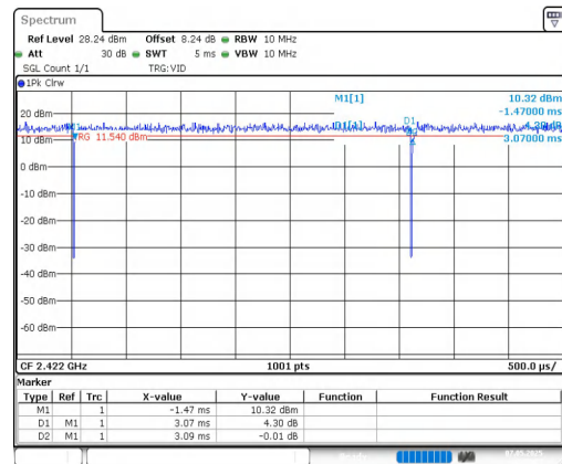
NTNV-11N40MIMO-Ant2-2422
