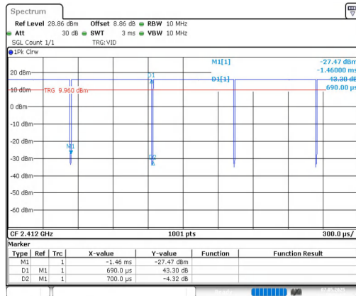
NTNV-11B-CDD-Ant1-2412
