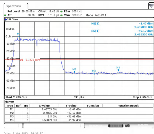
11AX40MIMO-Ant2-2452-PASS
