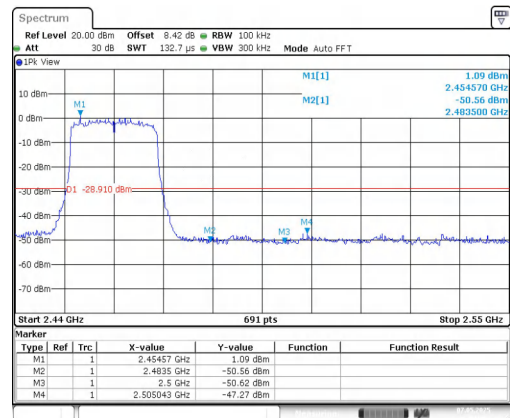
11AX20MIMO-Ant2-2462-PASS
