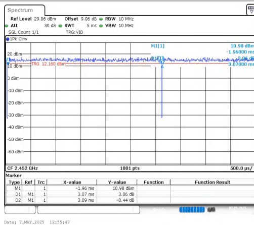
NTNV-11N40MIMO-Ant1-2452
