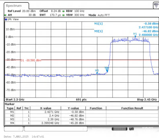
11AX40MIMO-Ant2-2422-PASS
