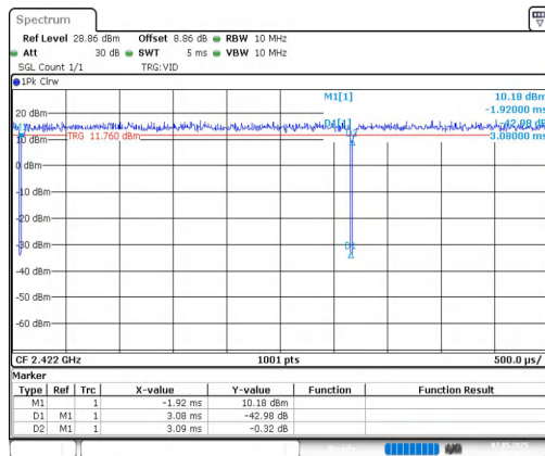
NTNV-11N40MIMO-Ant1-2422
