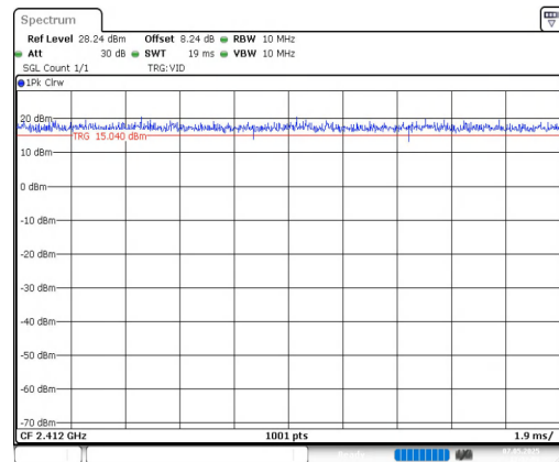
NTNV-11N20MIMO-Ant2-2412
