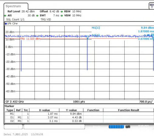
NTNV-11N40MIMO-Ant2-2452
