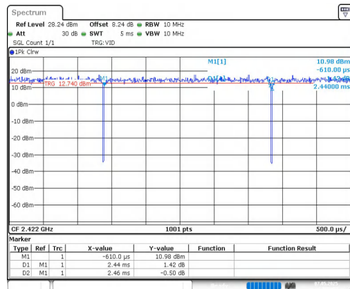
NTNV-11AX40MIMO-Ant2-2422
