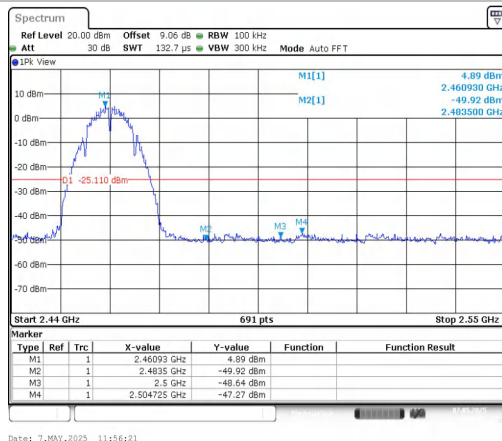
11B-CDD-Ant1-2462-PASS
