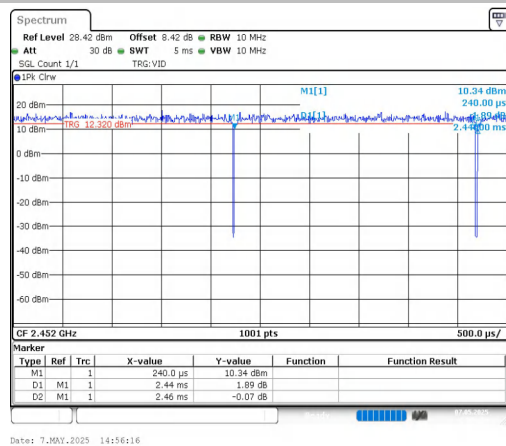
NTNV-11AX40MIMO-Ant2-2452
