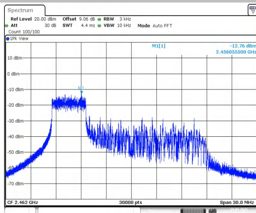
11AX20MIMO-Ant1-2462-26Tone-RU8-PASS
