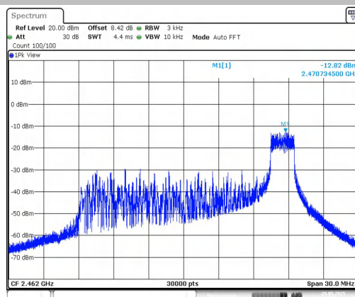
11AX20MIMO-Ant2-2462-26Tone-RU0-PASS
