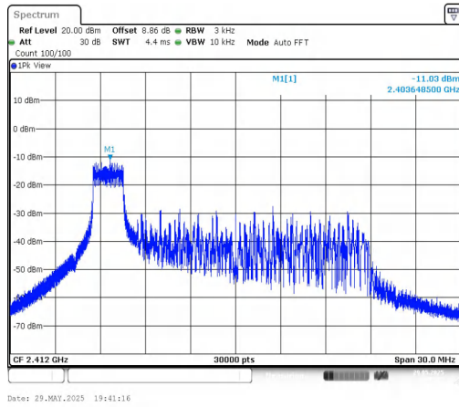
11AX20MIMO-Ant1-2412-26Tone-RU0-PASS
