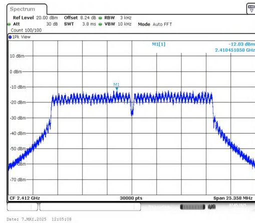
11G-CDD-Ant2-2412-PASS
