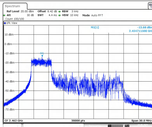
11AX20MIMO-Ant2-2462-26Tone-RU8-PASS
