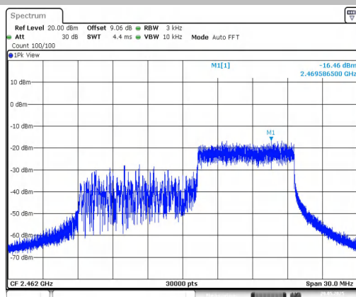
11AX20MIMO-Ant1-2462-26Tone-RU0-PASS
