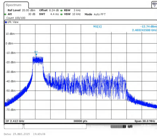
11AX20MIMO-Ant2-2412-26Tone-RU0-PASS
