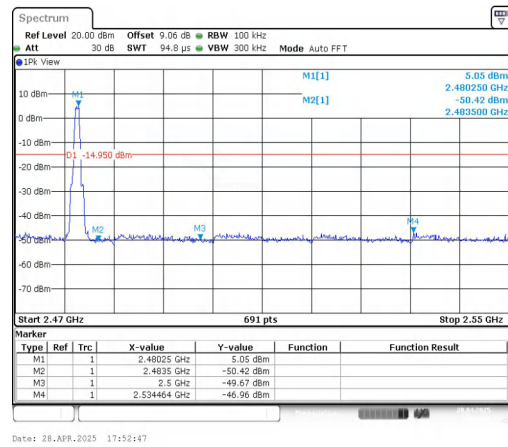
BLE_1M-Ant1-2480-PASS
