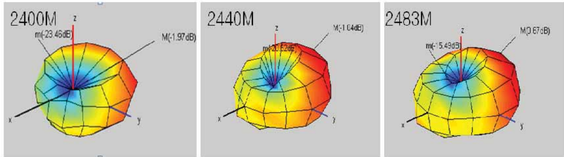
< 3D Pattern >
