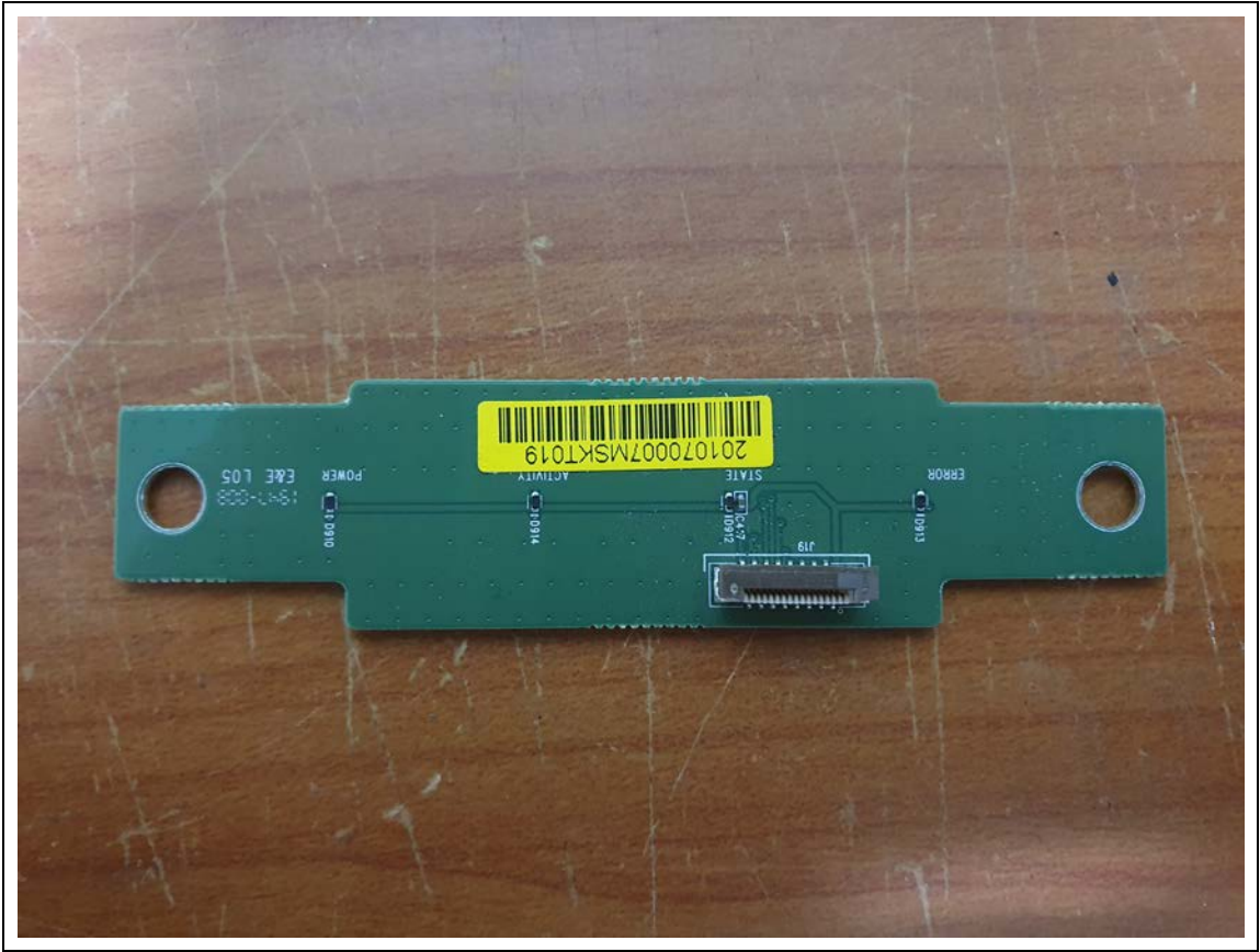
Sub Board-Rear
