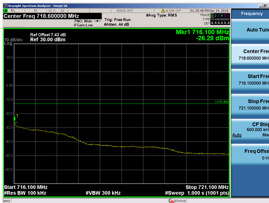
LTE Band 12 / 5MHz / QPSK - RB Size/Offset (12/13)
