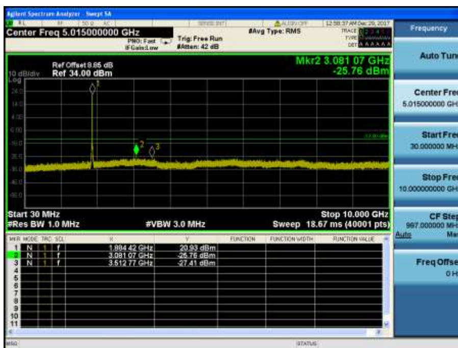
LTE Band 2 / 20MHz / QPSK - RB Size/Offset (50/25) – Mid Channel
