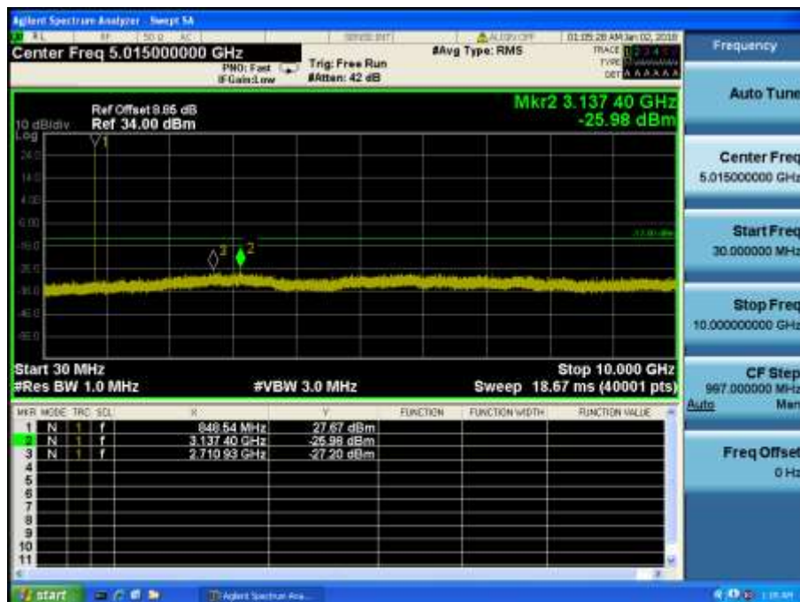
LTE Band 5 / 1.4MHz / 16QAM - RB Size/Offset (1/3) – High Channel
