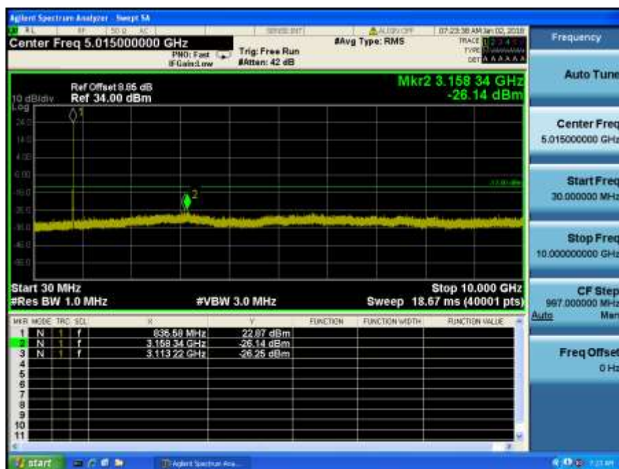
LTE Band 5 / 10MHz / 16QAM - RB Size/Offset (25/0) – Mid Channel
