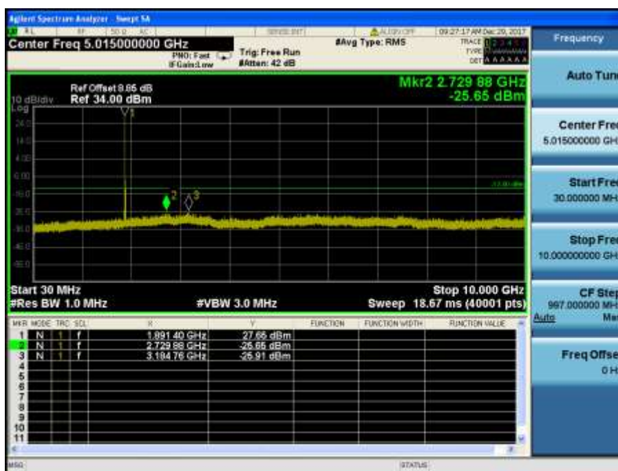
LTE Band 2 / 20MHz / 16QAM - RB Size/Offset (1/0) – High Channel
