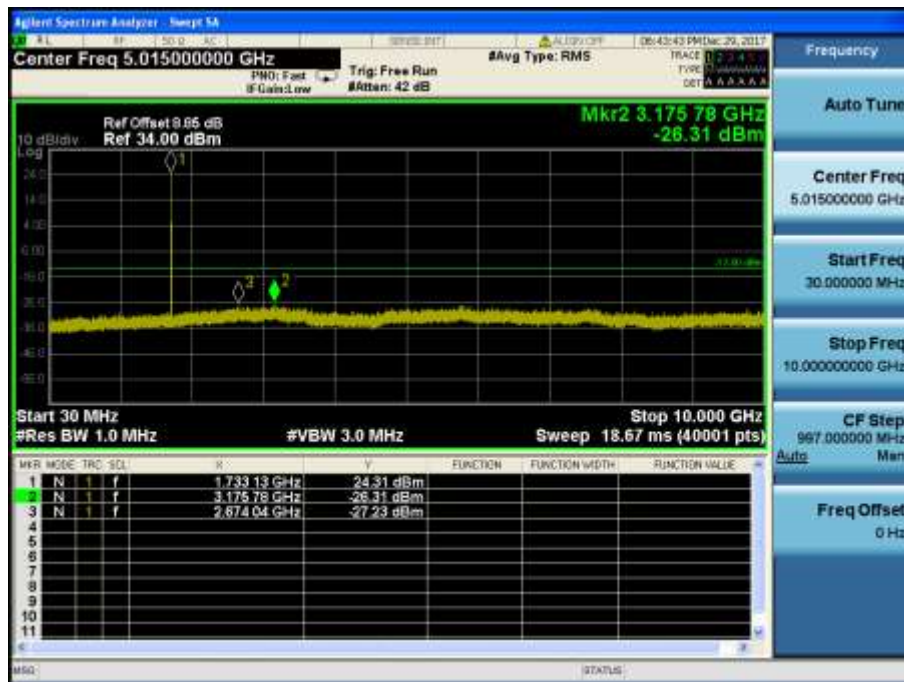
LTE Band 4 / 3MHz / QPSK - RB Size/Offset (8/3) – Mid Channel
