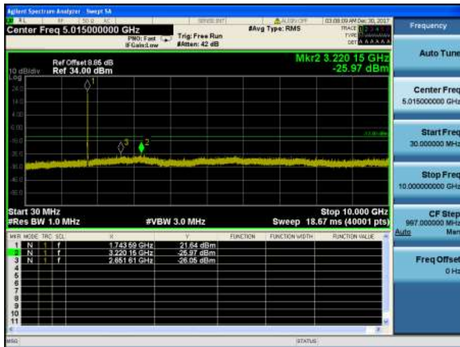
LTE Band 4 / 15MHz / QPSK - RB Size/Offset (36/0) – High Channel
