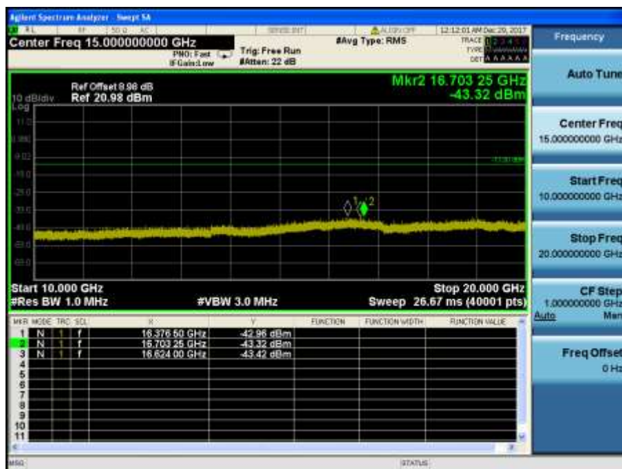
LTE Band 2 / 15MHz / QPSK - RB Size/Offset (36/19) – Mid Channel
