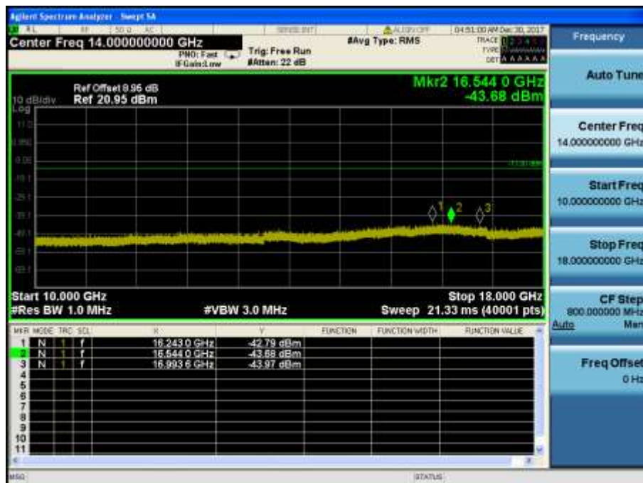
LTE Band 4 / 20MHz / QPSK - RB Size/Offset (50/50) – High Channel
