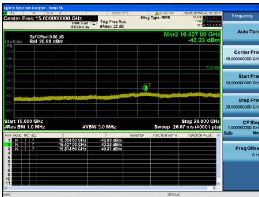
LTE Band 2 / 1.4MHz / QPSK - RB Size/Offset (3/1) – Low Channel
