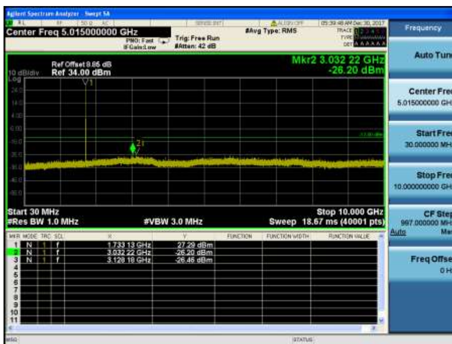
LTE Band 4 / 1.4MHz / 16QAM - RB Size/Offset (3/3) – Mid Channel
