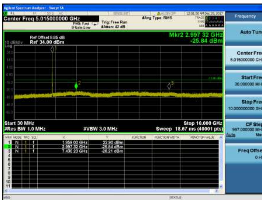
LTE Band 2 / 15MHz / QPSK - RB Size/Offset (36/39) – Low Channel
