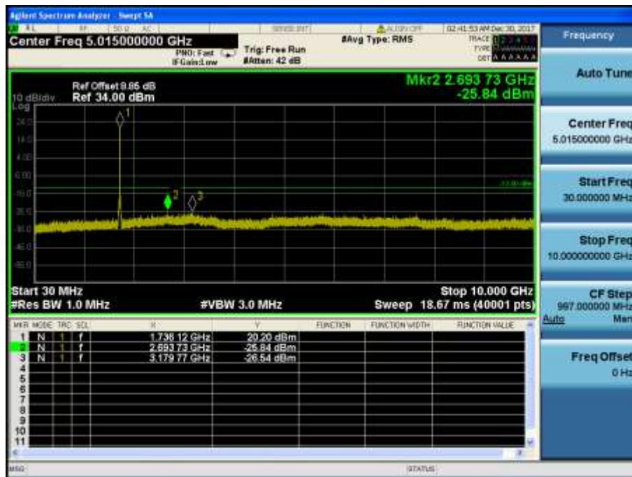
LTE Band 4 / 15MHz / QPSK - RB Size/Offset (75/0) – Mid Channel
