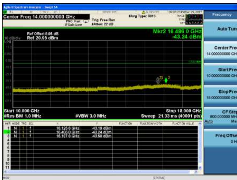
LTE Band 4 / 5MHz / QPSK - RB Size/Offset (1/12) – Low Channel
