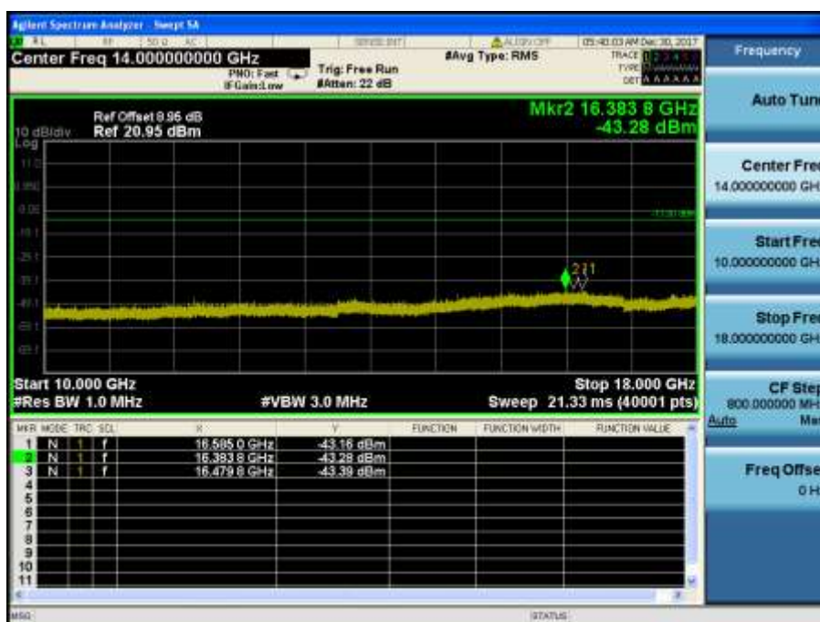
LTE Band 4 / 1.4MHz / 16QAM - RB Size/Offset (3/3) – Mid Channel
