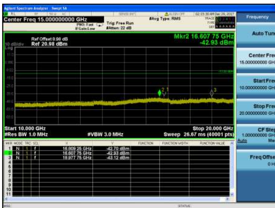
LTE Band 2 / 1.4MHz / 16QAM - RB Size/Offset (1/0) – High Channel
