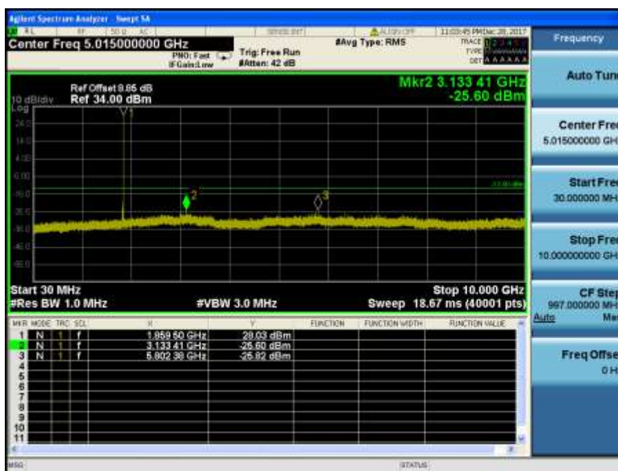
LTE Band 2 / 10MHz / QPSK - RB Size/Offset (1/49) – Low Channel
