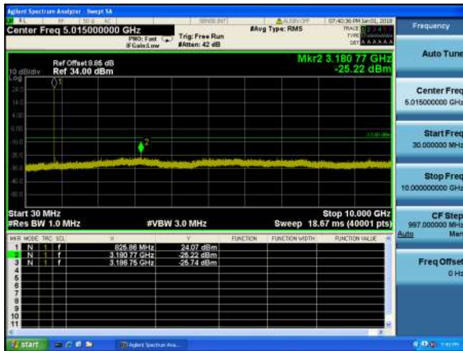
LTE Band 5 / 3MHz / QPSK - RB Size/Offset (8/3) – Low Channel
