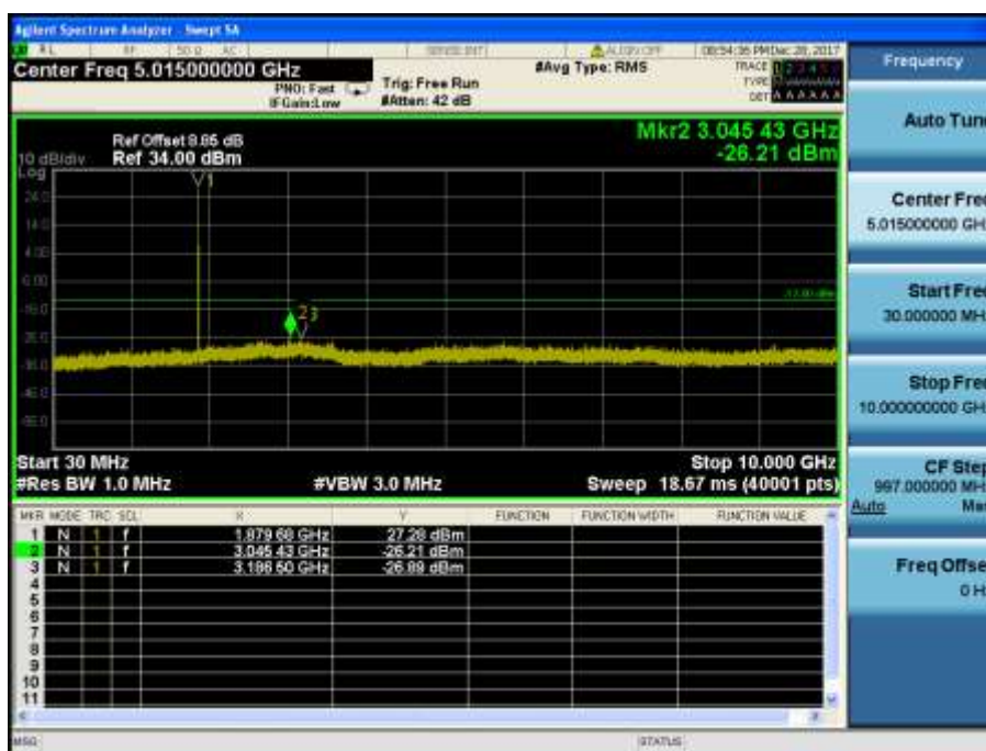
LTE Band 2 / 1.4MHz / QPSK - RB Size/Offset (1/0) – Mid Channel
