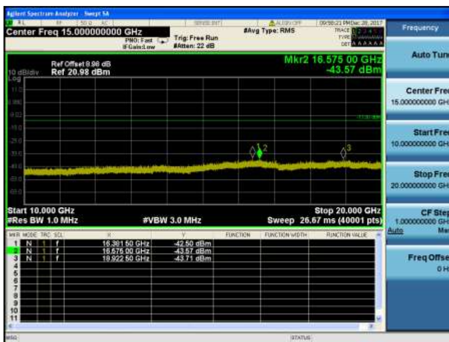
LTE Band 2 / 3MHz / QPSK - RB Size/Offset (8/0) – High Channel
