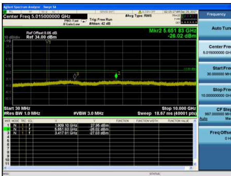
LTE Band 2 / 1.4MHz / 16QAM - RB Size/Offset (1/0) – High Channel
