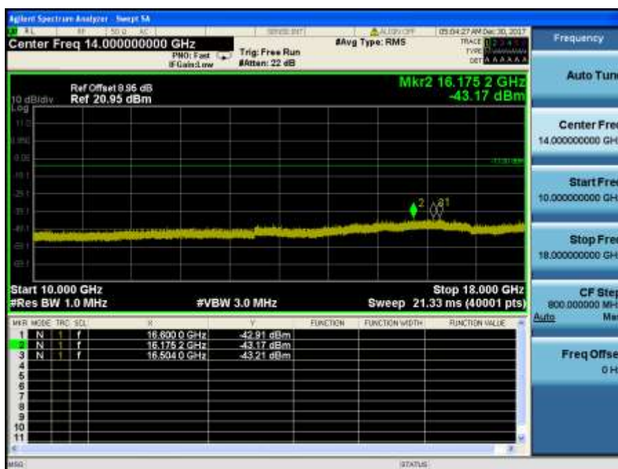
LTE Band 4 / 1.4MHz / 16QAM - RB Size/Offset (1/5) – Low Channel
