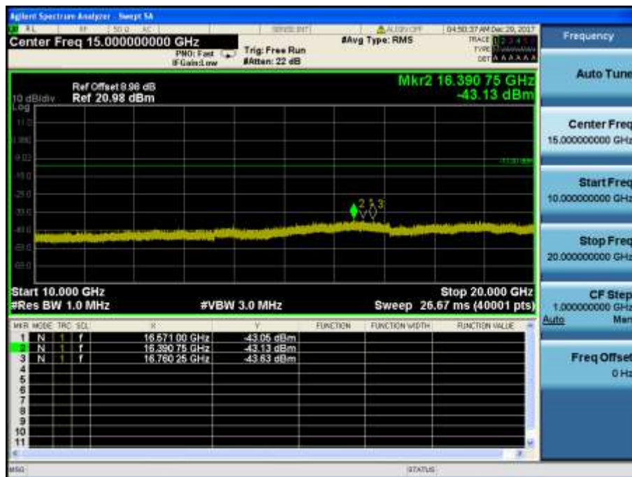
LTE Band 2 / 5MHz / 16QAM - RB Size/Offset (25/0) – Low Channel
