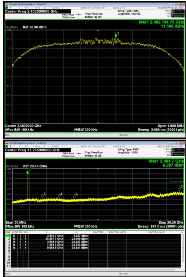
2DH5-CH0 30MHz to 26.5GHz
