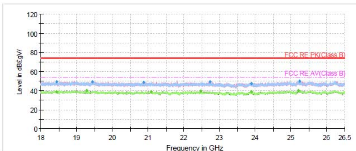
Radiates Emission from 18GHz to 26.5GHz
