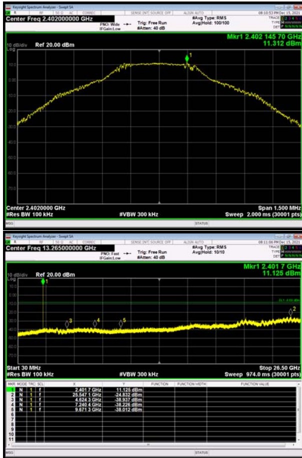
DH5-CH0 30MHz to 26.5GHz
