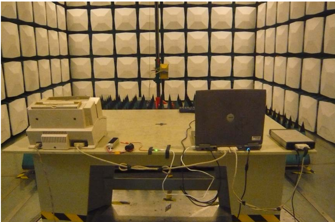
Radiated Emission –Rear View (Above 1 GHz)
