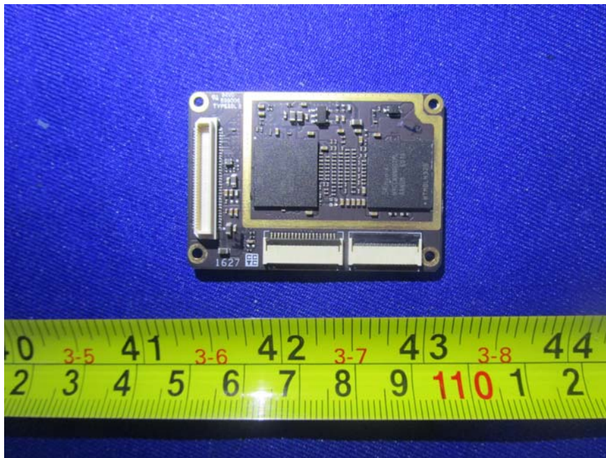
EUT – Board 6 Bottom View
