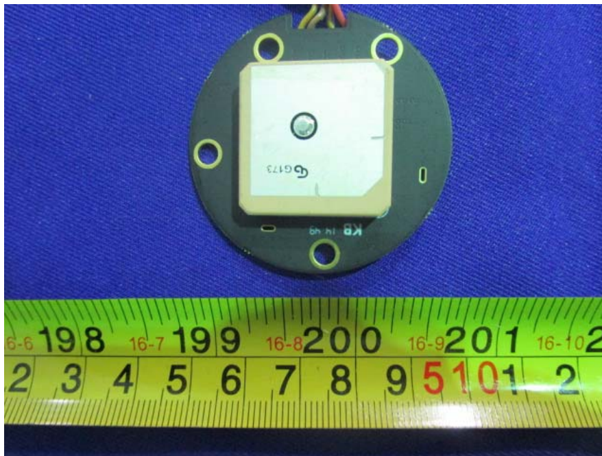
EUT –GPS Board Bottom & Antenna View
