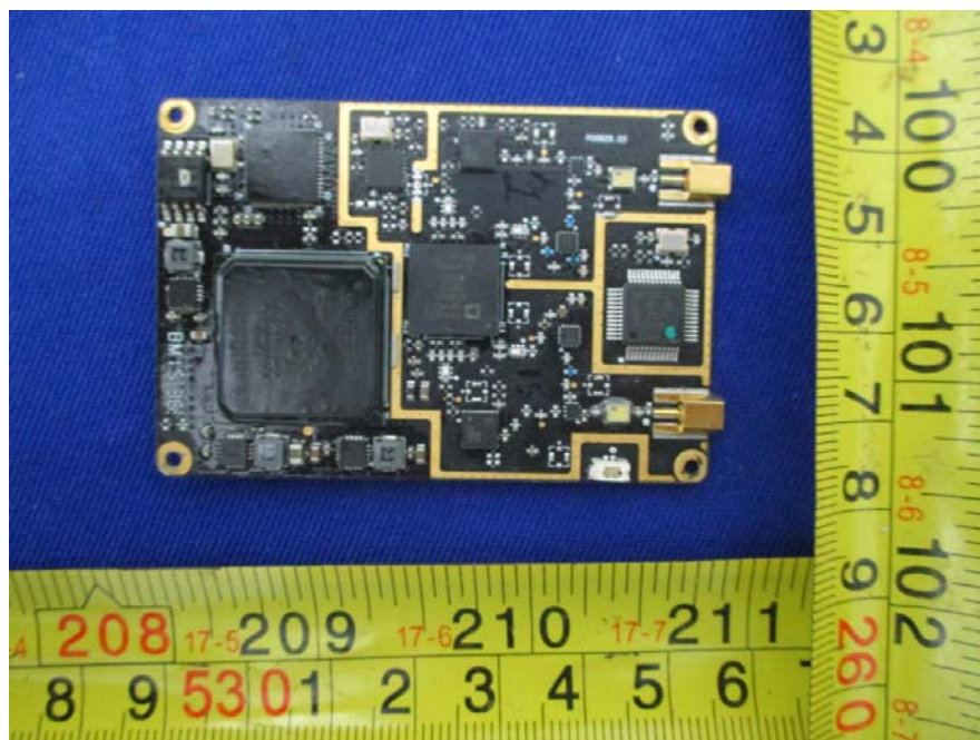
EUT – RF Moudle RF Board Top View
