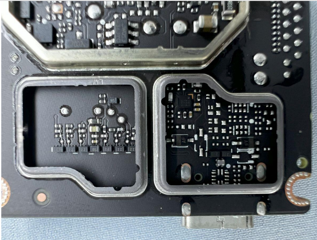
Internal View of EUT-83
