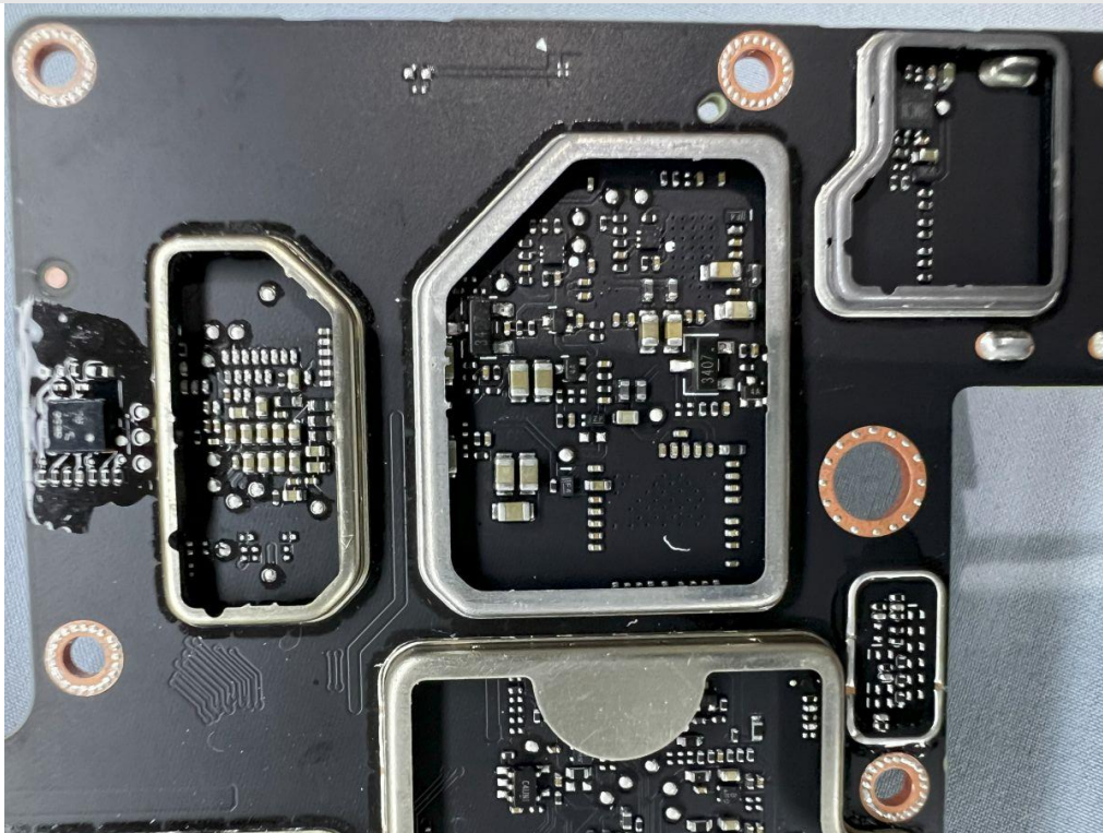
Internal View of EUT-81
