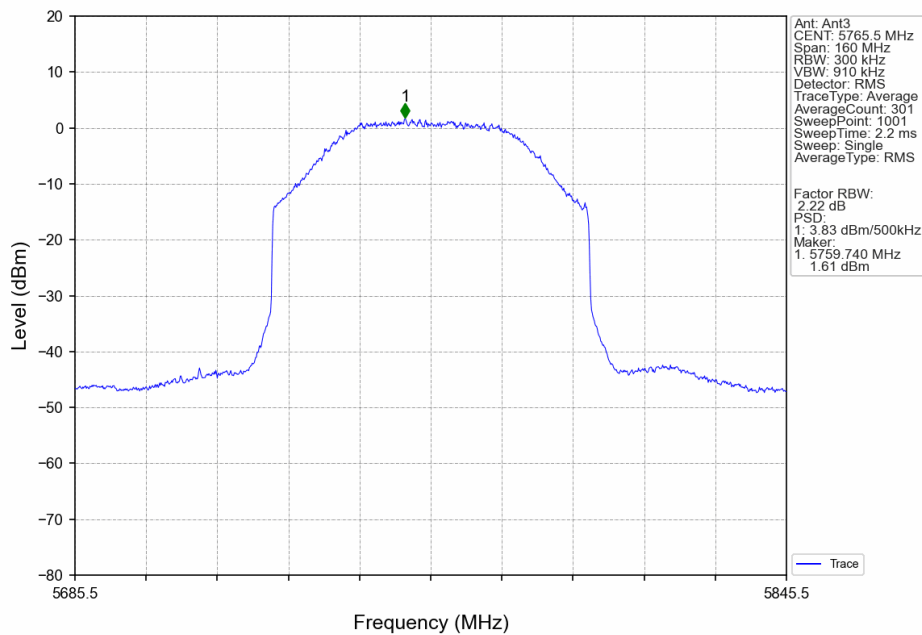
80M_LCH_5765.5MHz_Ant3_NTNV
