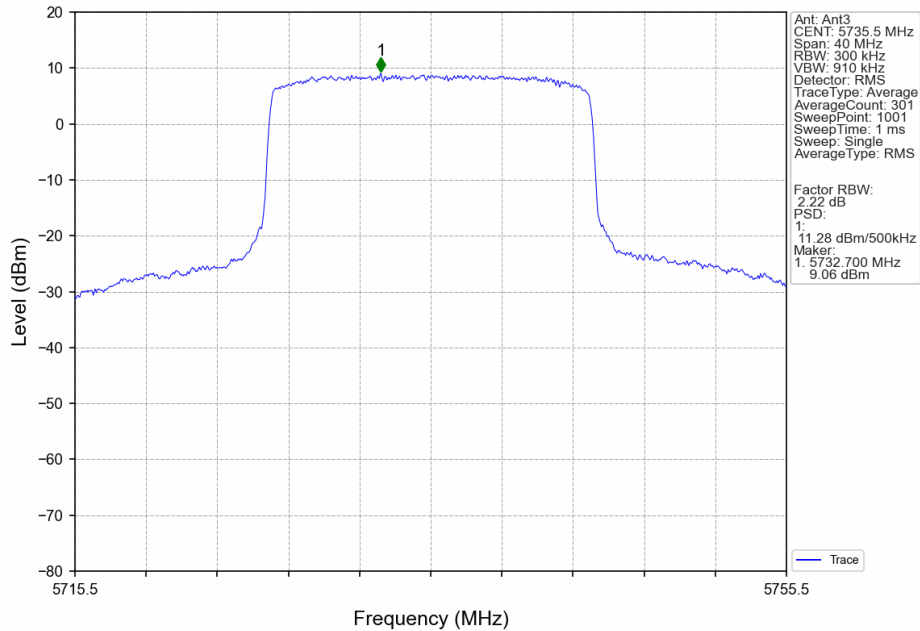
20M_LCH_5735.5MHz_MIMO_NTNV
