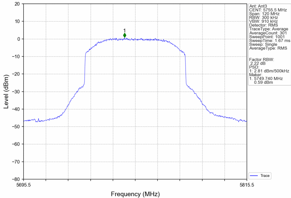
60M_LCH_5755.5MHz_MIMO_NTNV
