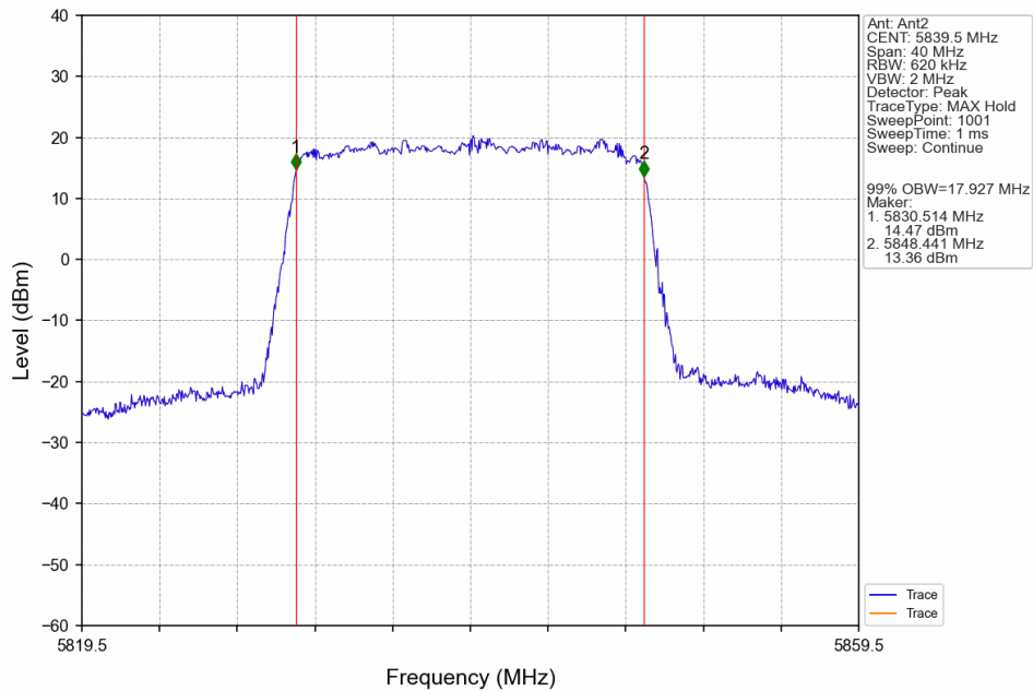
20M_HCH_5839.5MHz_Ant2_NTNV
