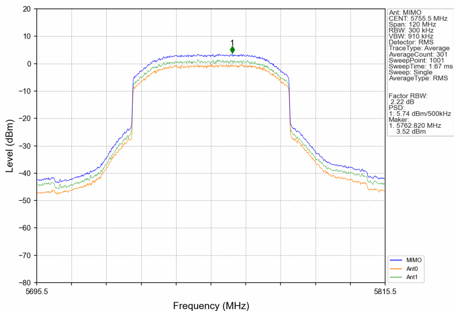
60M_LCH_5755.5MHz_MIMO_NTNV
