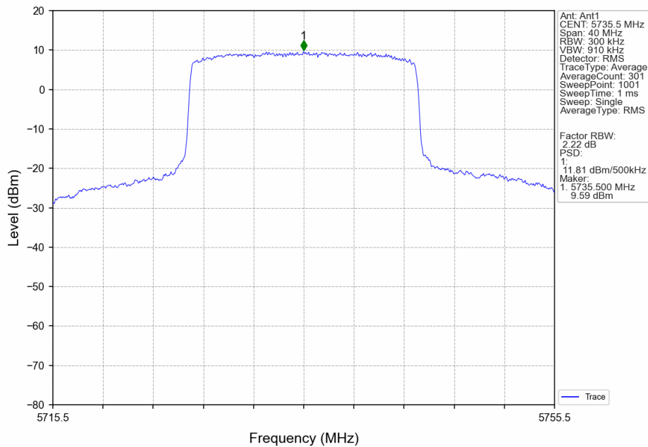
20M_LCH_5735.5MHz_MIMO_NTNV
