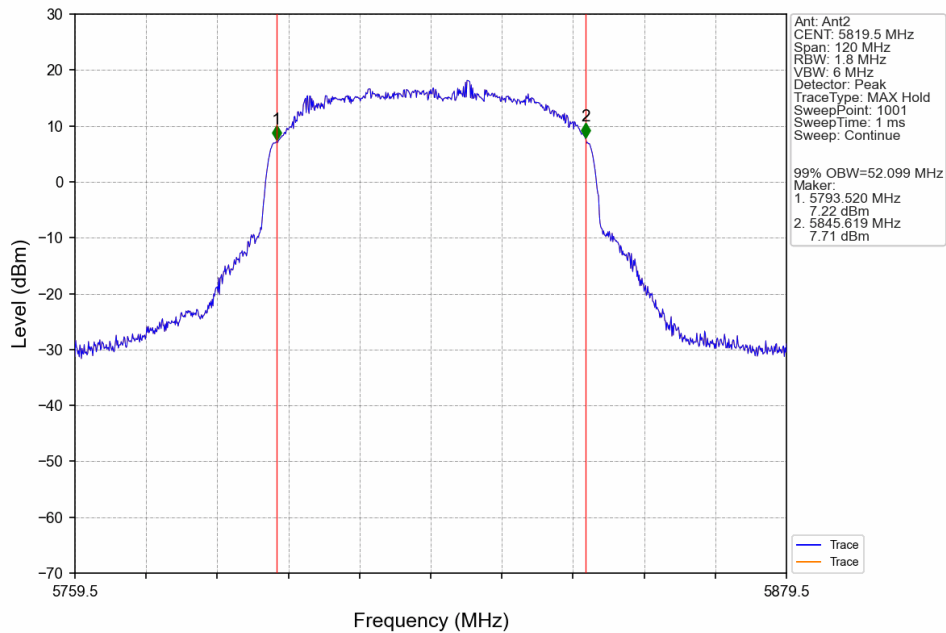
60M_HCH_5819.5MHz_Ant2_NTNV
