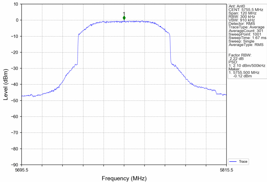
60M_LCH_5755.5MHz_Ant0_NTNV
