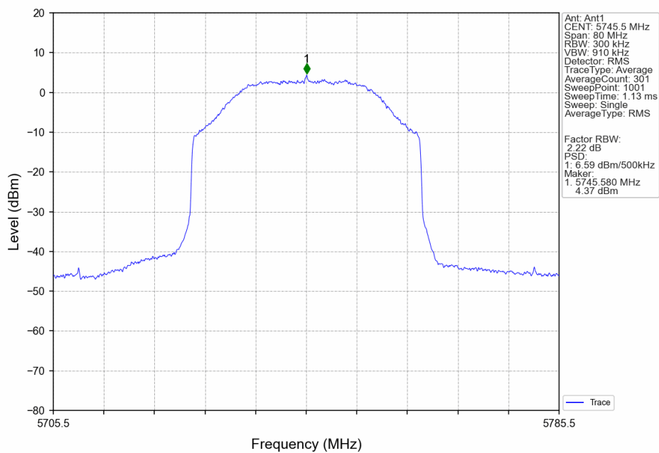
40M_LCH_5745.5MHz_Ant1_NTNV
