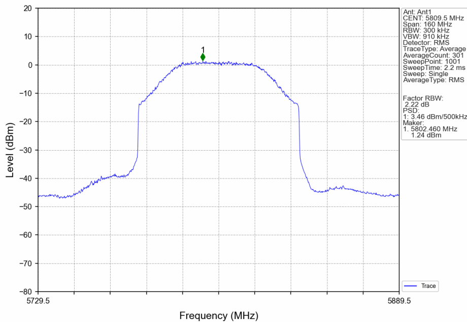
80M_HCH_5809.5MHz_Ant1_NTNV
