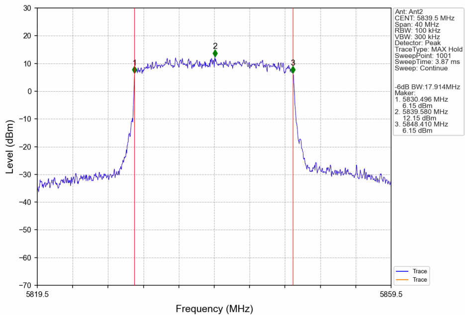
20M_HCH_5839.5MHz_Ant2_NTNV
