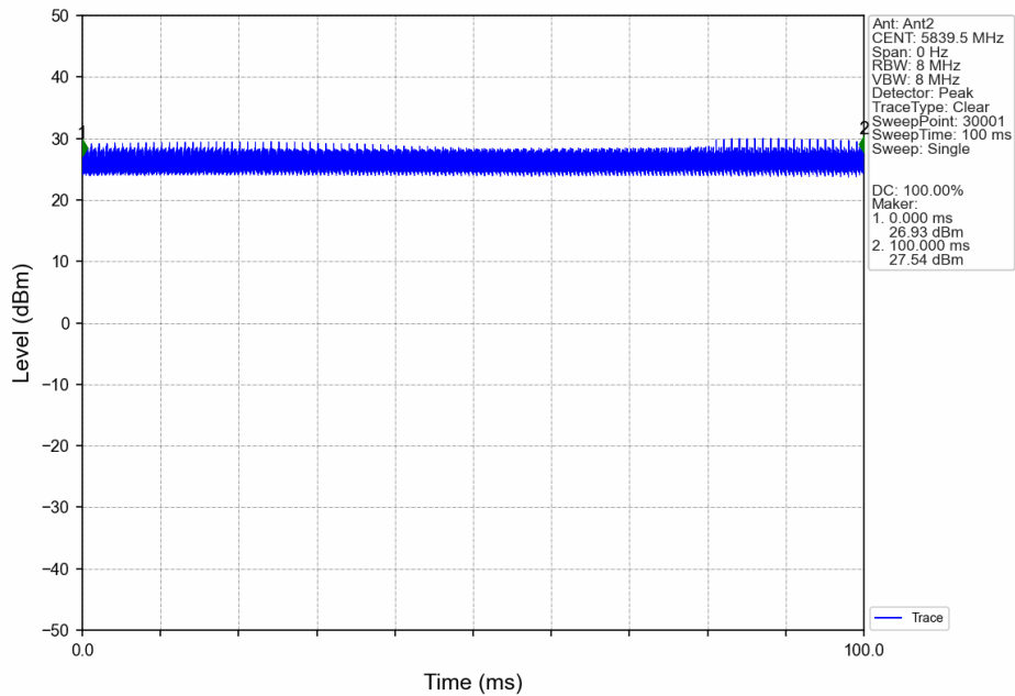
20M_HCH_5839.5MHz_Ant2_NTNV
