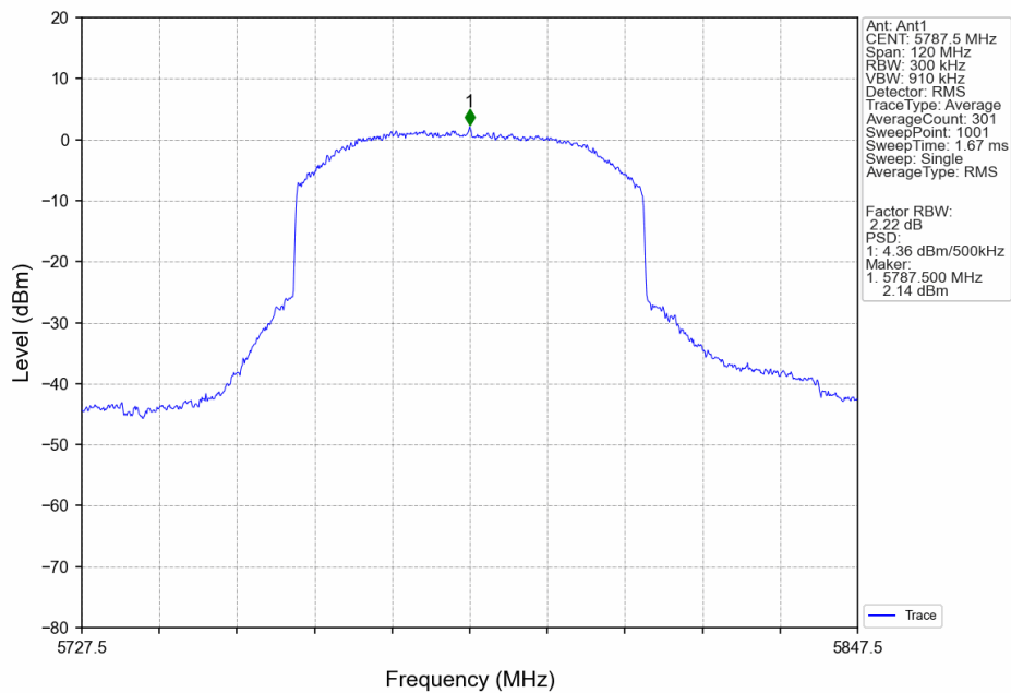
60M_MCH_5787.5MHz_Ant1_NTNV
