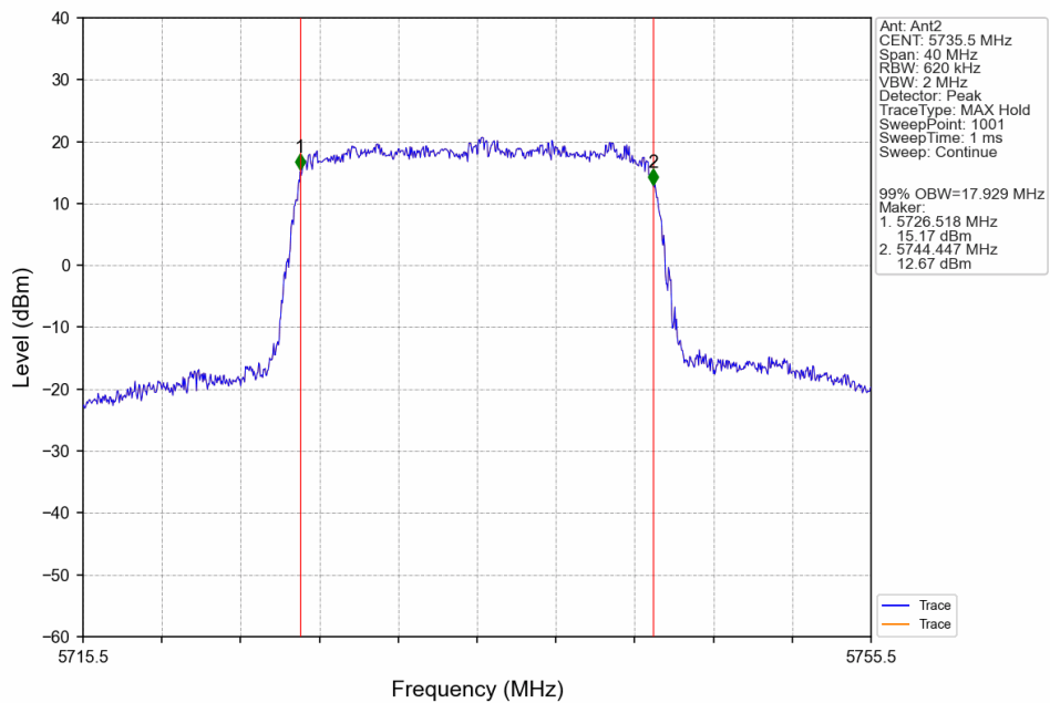
20M_LCH_5735.5MHz_Ant2_NTNV
