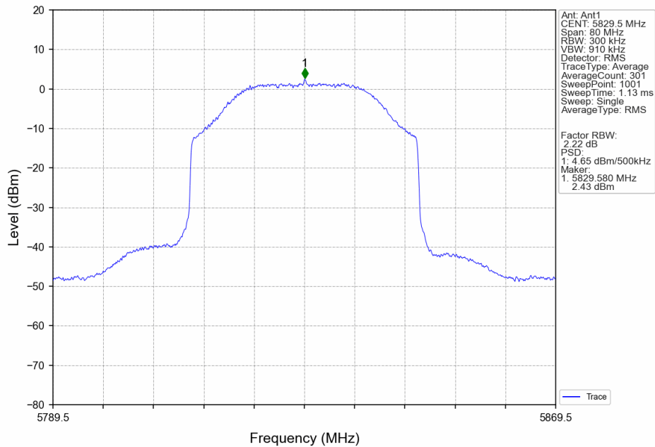
40M_HCH_5829.5MHz_Ant1_NTNV
