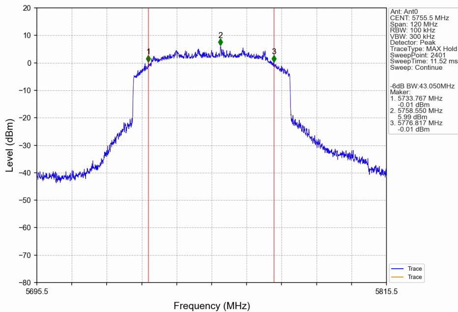
60M_LCH_5755.5MHz_Ant0_NTNV
