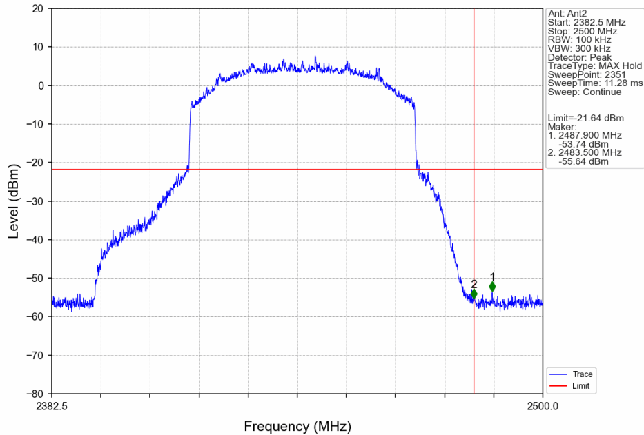
60M_HCH_2442.5MHz_Ant2_NTNV
