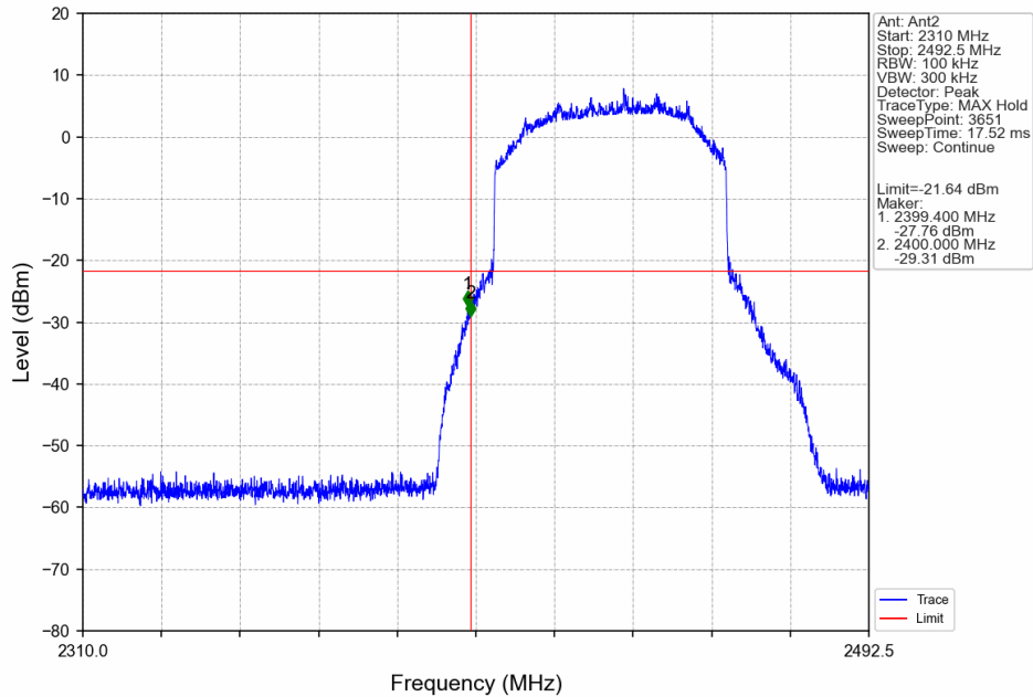
60M_LCH_2432.5MHz_Ant2_NTNV
