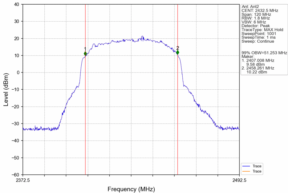
60M_LCH_2432.5MHz_Ant2_NTNV
