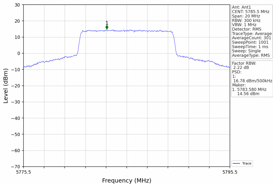
10M_MCH_5785.5MHz_Ant1_NTNV
