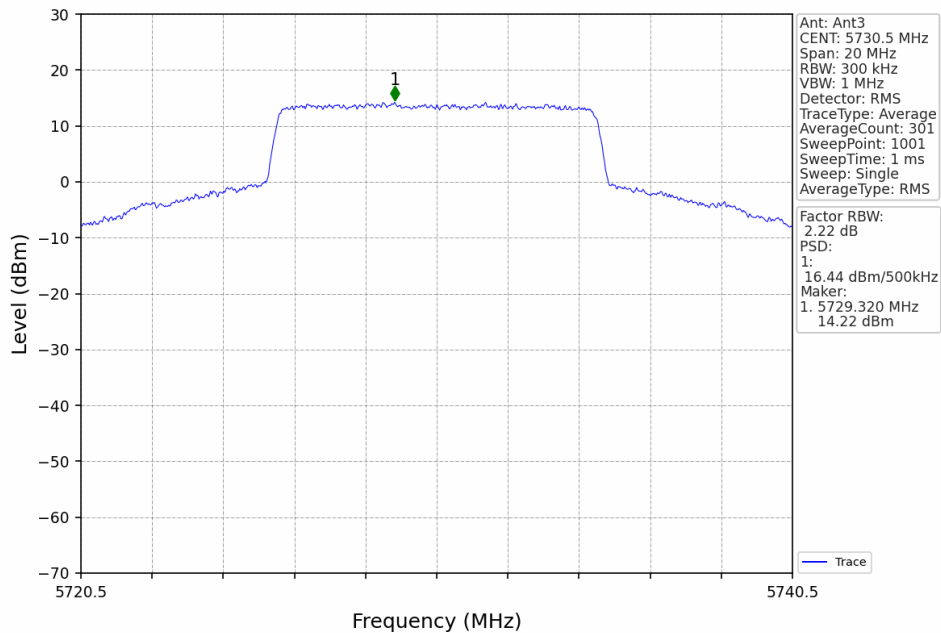
10M_LCH_5730.5MHz_Ant3_NTNV
