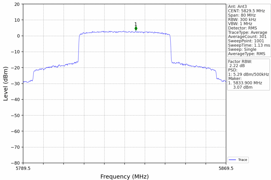
40M_HCH_5829.5MHz_Ant3_NTNV
