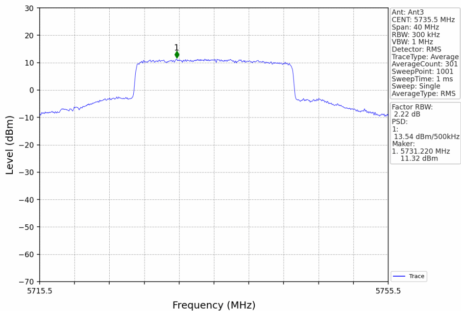
20M_LCH_5735.5MHz_Ant3_NTNV
