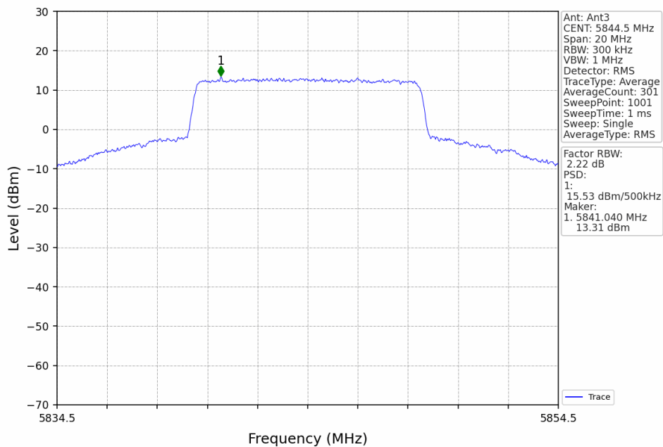
10M_HCH_5844.5MHz_Ant3_NTNV
