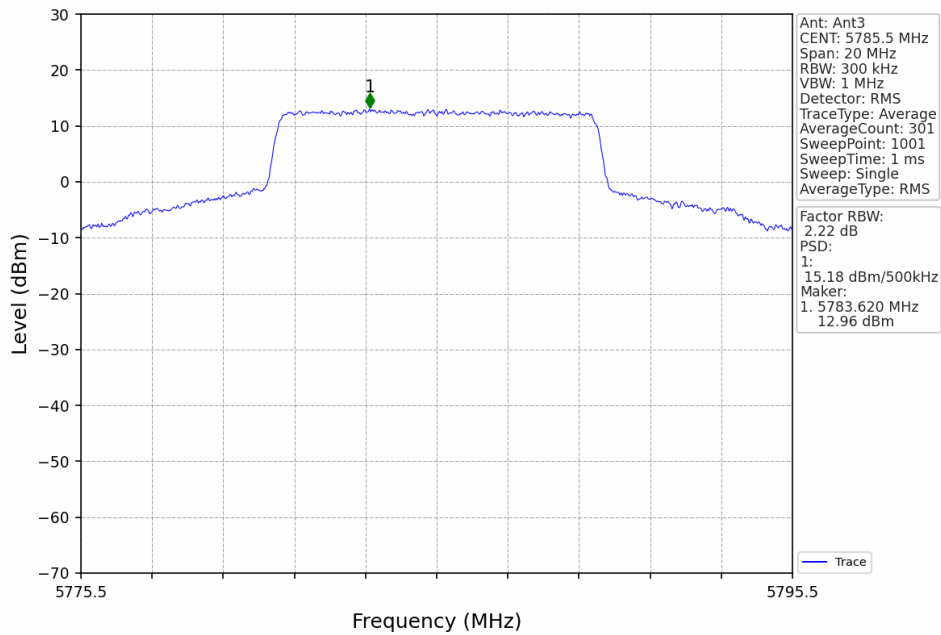
10M_MCH_5785.5MHz_Ant3_NTNV
