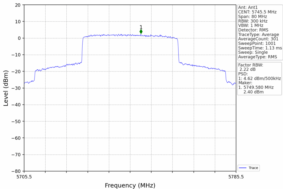
40M_LCH_5745.5MHz_Ant1_NTNV
