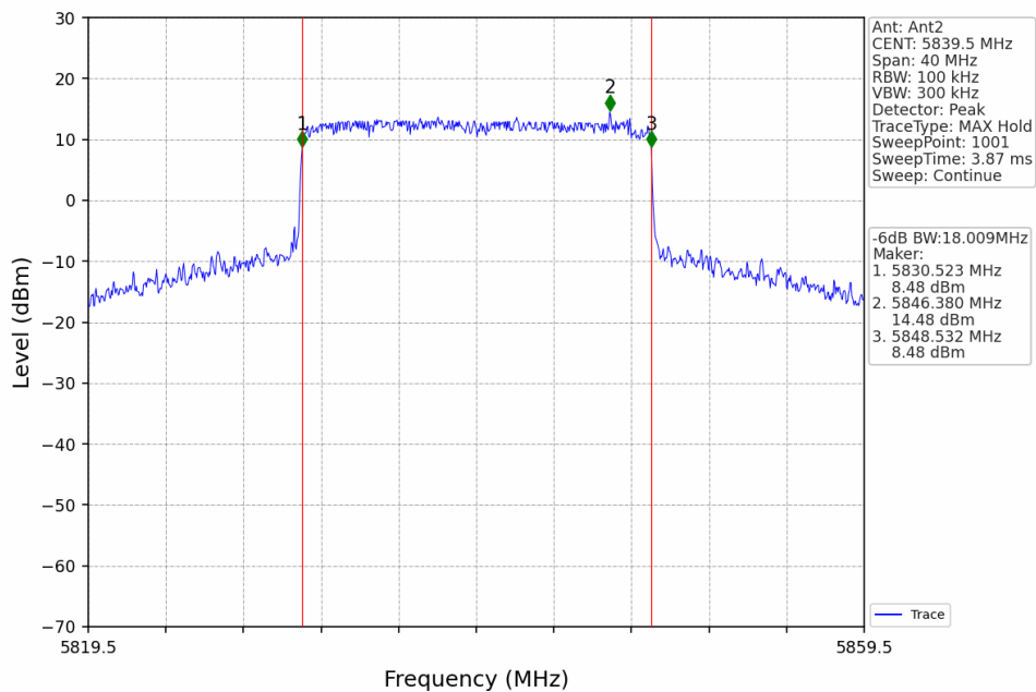
20M_HCH_5839.5MHz_Ant2_NTNV
