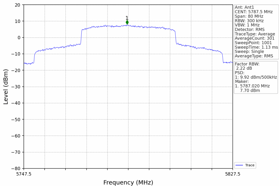
40M_MCH_5787.5MHz_Ant1_NTNV
