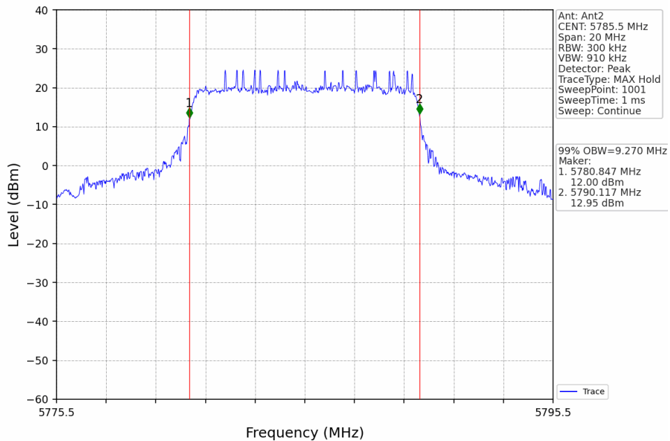
10M_MCH_5785.5MHz_Ant2_NTNV
