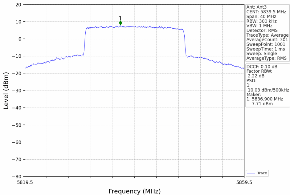
20M_HCH_5839.5MHz_Ant3_NTNV
