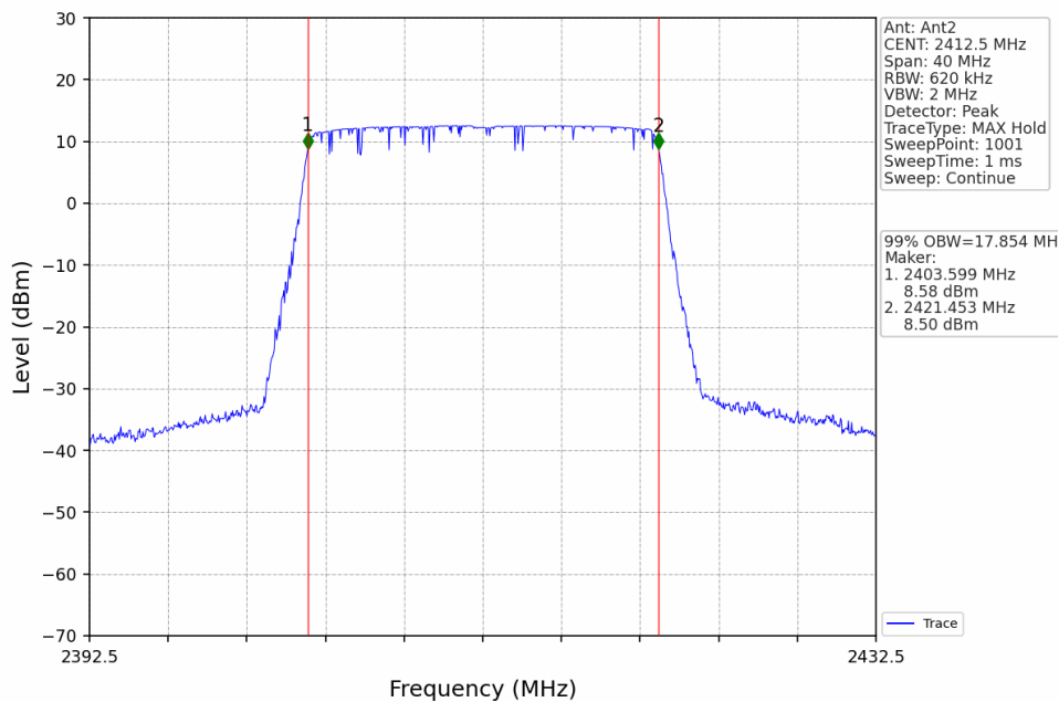
20M_LCH_2412.5MHz_Ant2_NTNV
