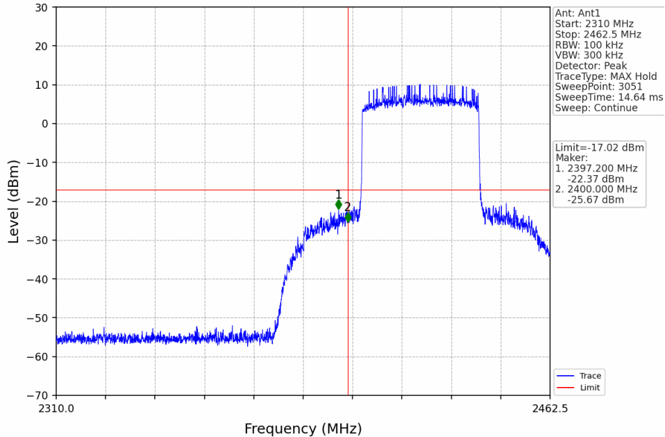
40M_LCH_2422.5MHz_Ant1_NTNV
