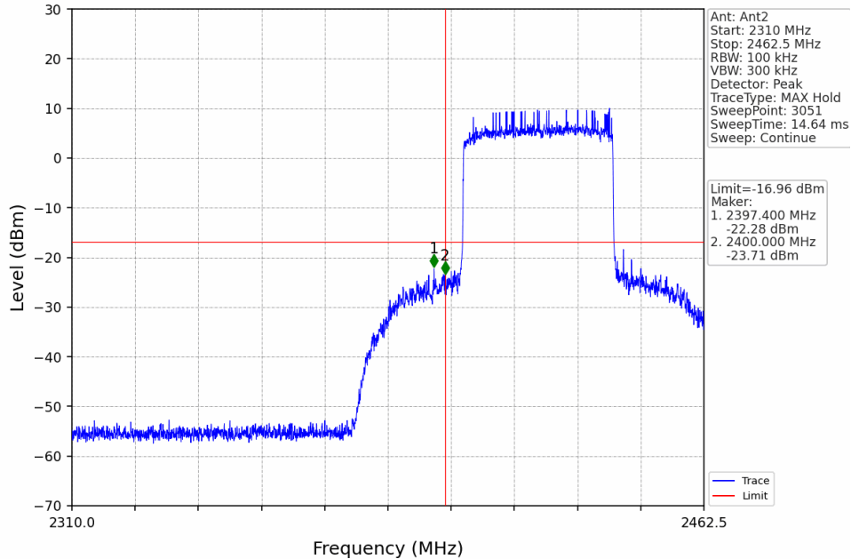
40M_LCH_2422.5MHz_Ant2_NTNV
