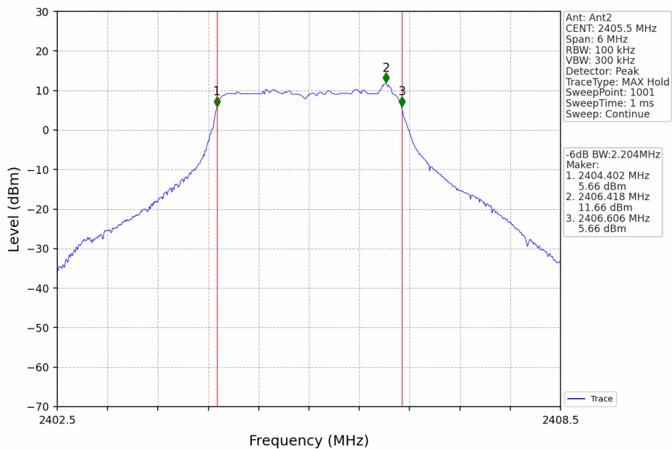
3M_LCH_2405.5MHz_Ant2_NTNV
