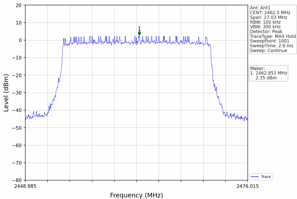
20M_HCH_2462.5MHz_Ant1_NTNV
