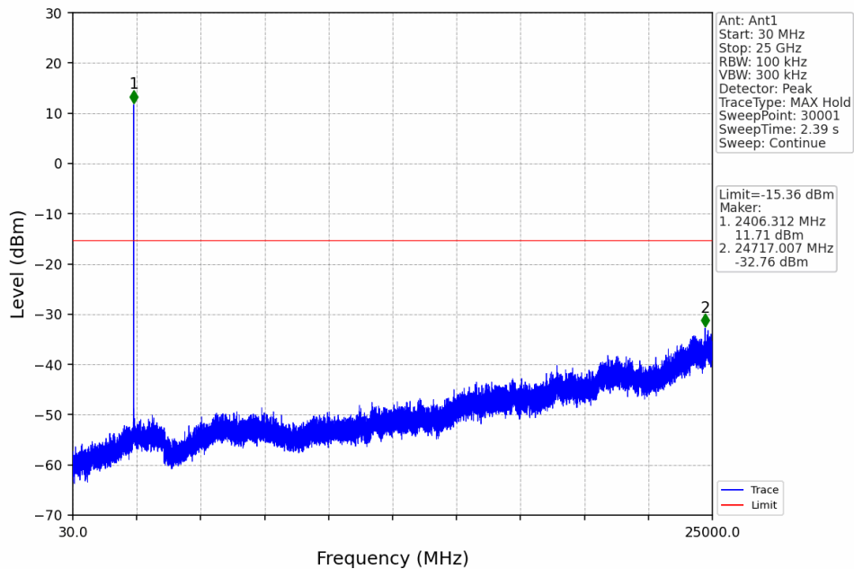
3M_LCH_2405.5MHz_Ant1_NTNV
