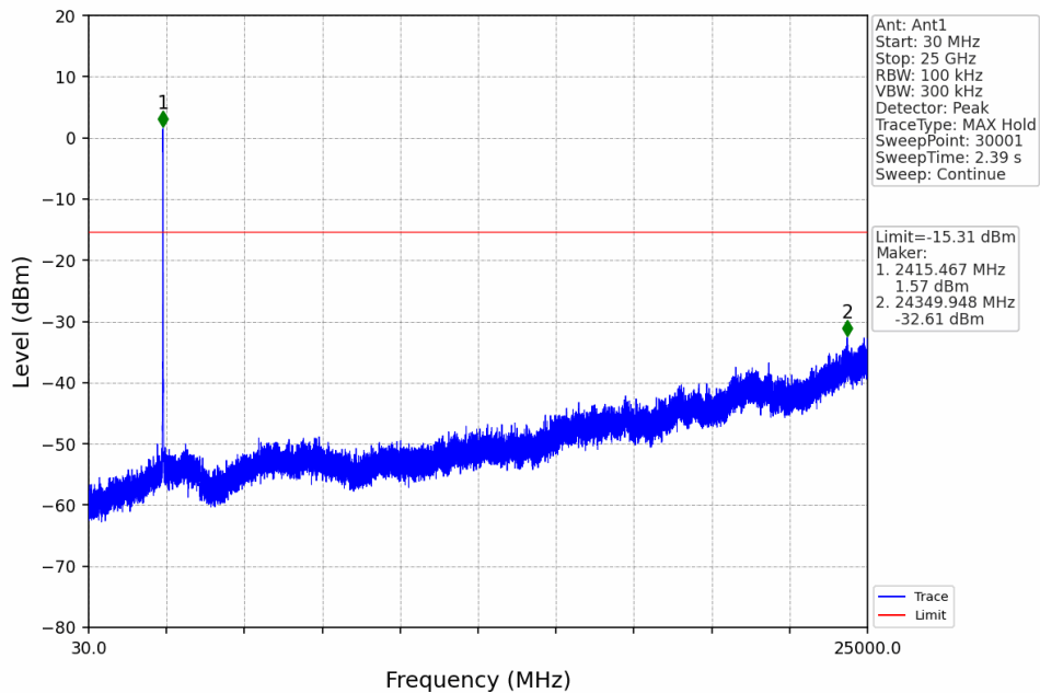
20M_LCH_2412.5MHz_Ant1_NTNV
