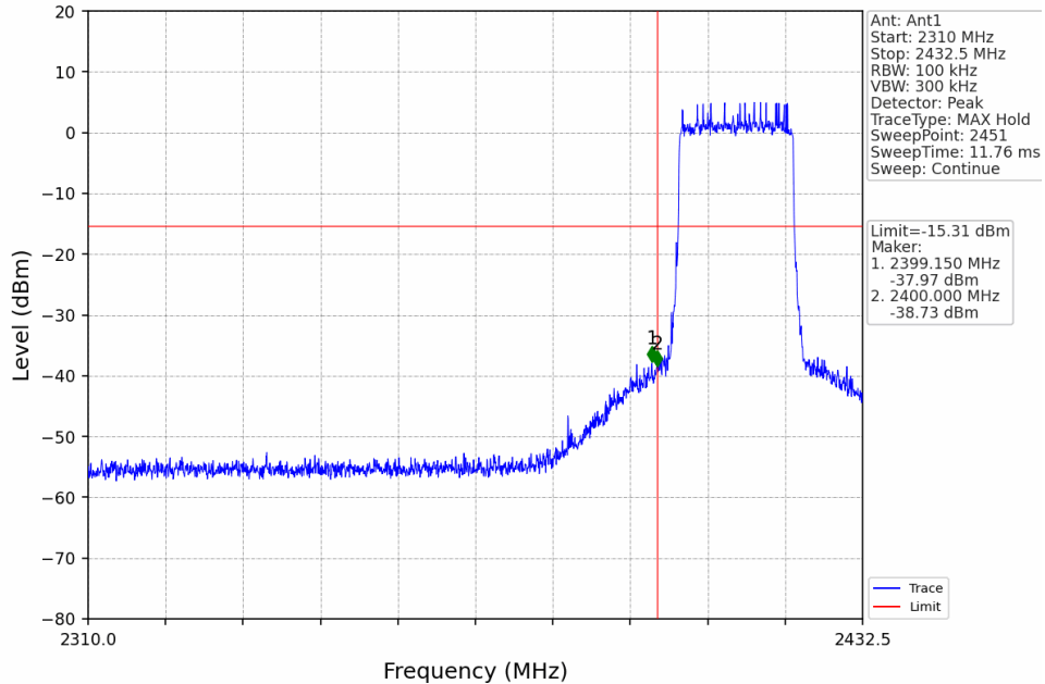
20M_LCH_2412.5MHz_Ant1_NTNV
