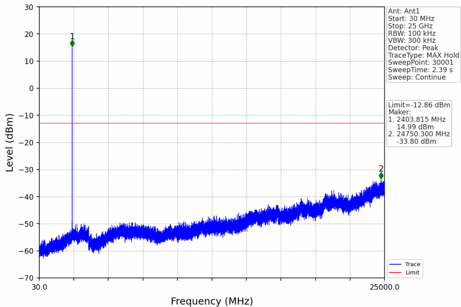
1.4M_LCH_2403.5MHz_Ant1_NTNV
