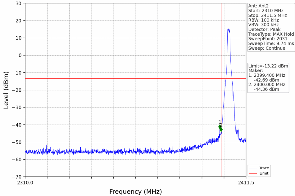
1.4M_LCH_2403.5MHz_Ant2_NTNV
