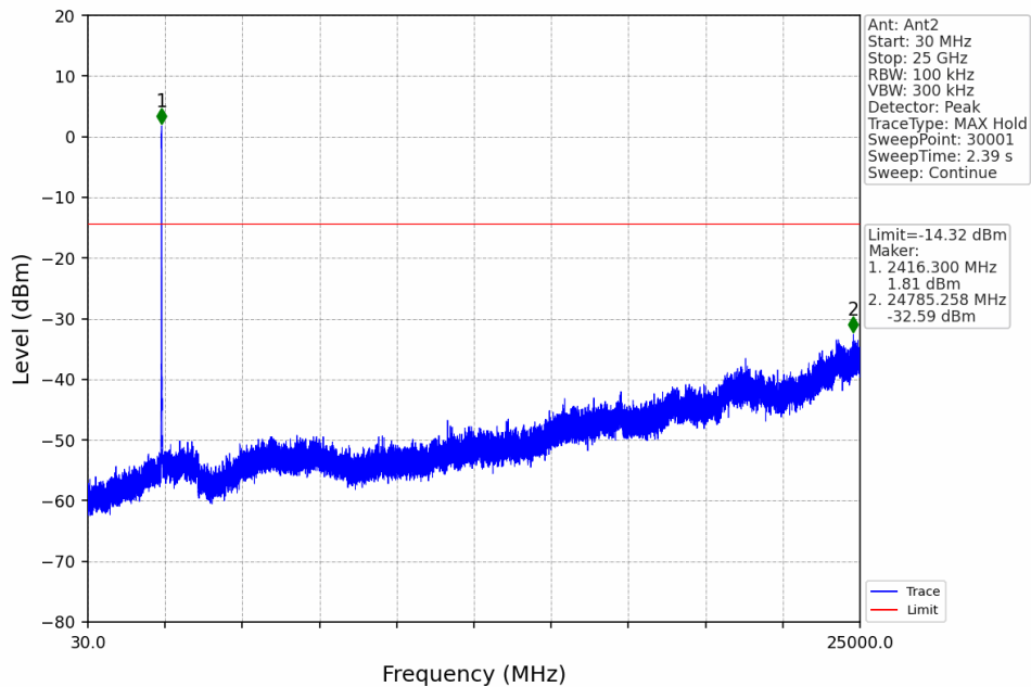
20M_LCH_2412.5MHz_Ant2_NTNV
