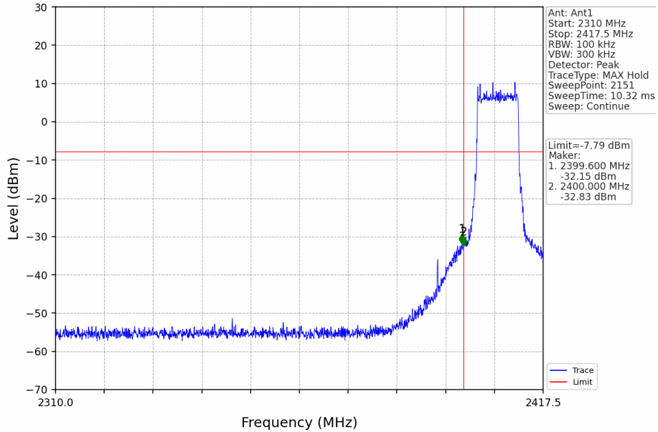
10M_LCH_2407.5MHz_Ant1_NTNV
