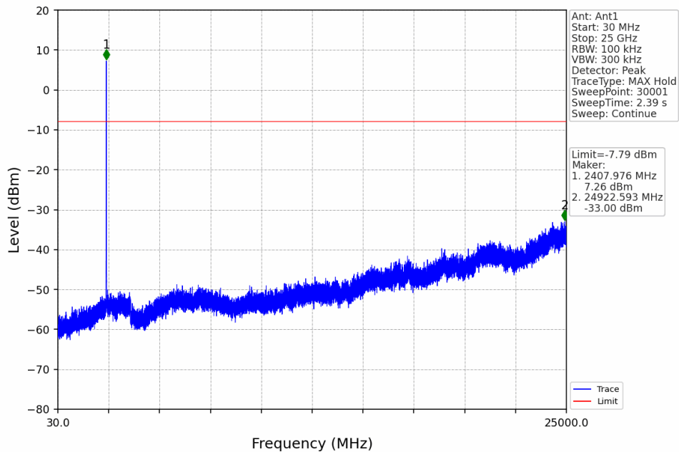
10M_LCH_2407.5MHz_Ant1_NTNV
