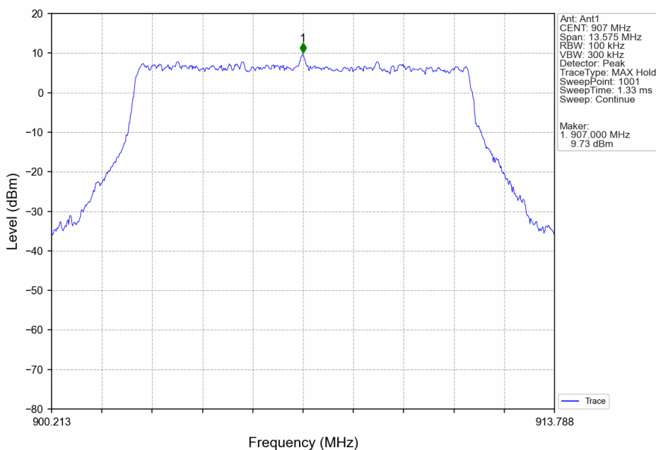
10M_LCH_907MHz_Ant1_NTNV
