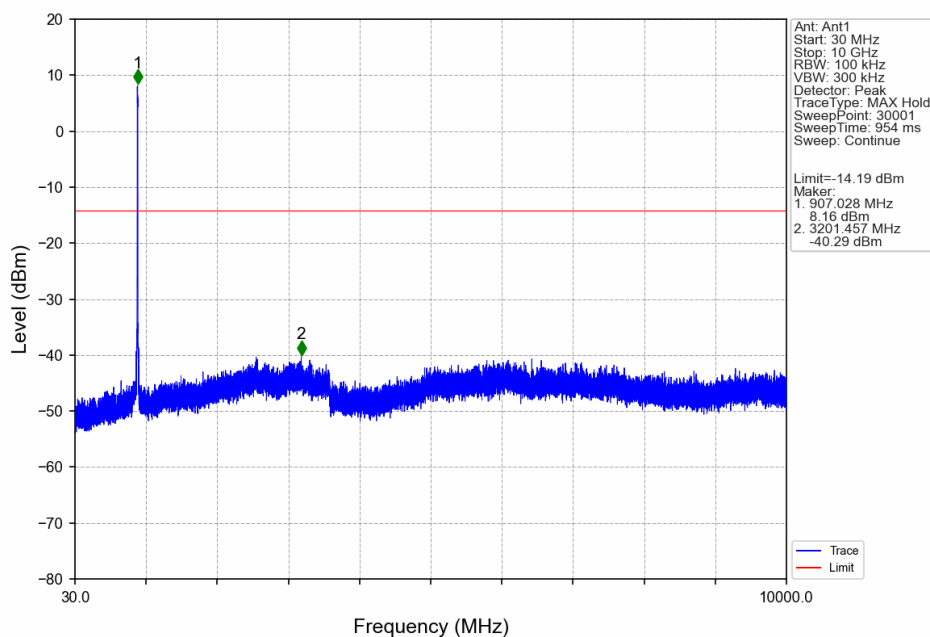
10M_LCH_907MHz_Ant1_NTNV
