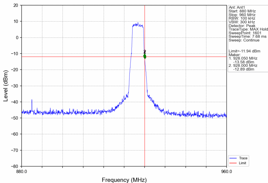
5M_HCH_925.4MHz_Ant1_NTNV
