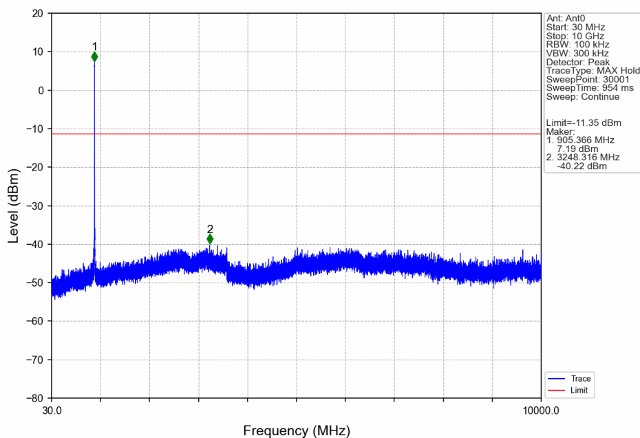
5M_LCH_904.6MHz_Ant0_NTNV
