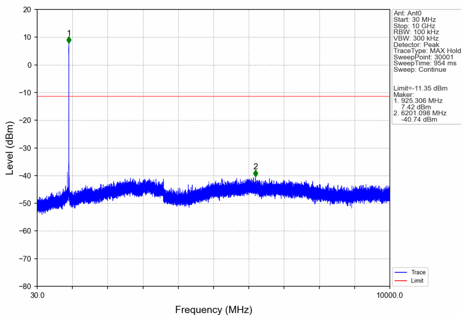
5M_HCH_925.4MHz_Ant0_NTNV
