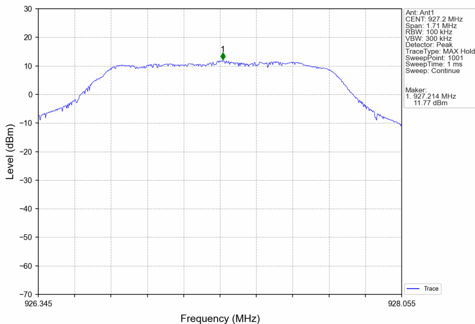
1.4M_HCH_927.2MHz_Ant1_NTNV
