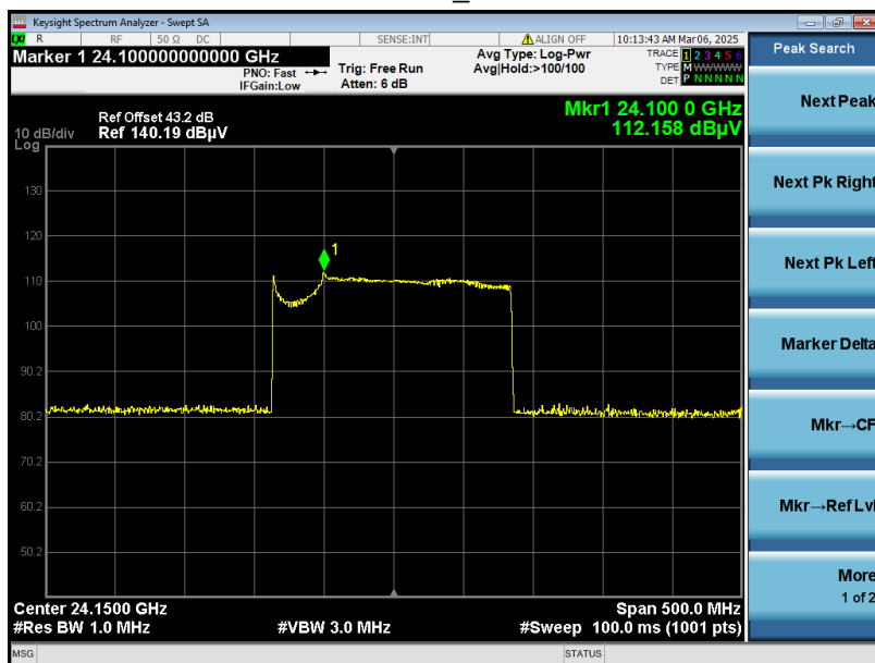
Vertical_Peak
