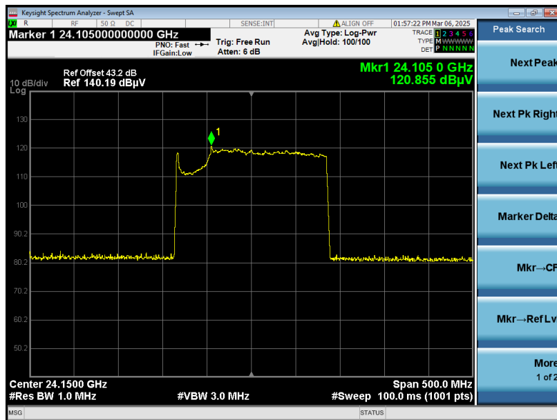
Horizontal_Peak
