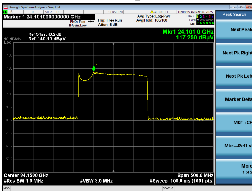
Horizontal_Peak
