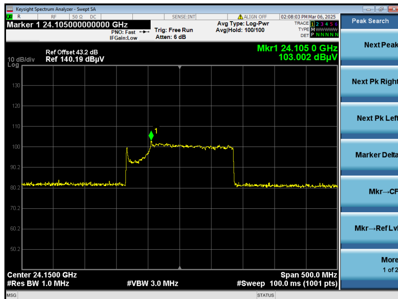
Vertical_Peak
