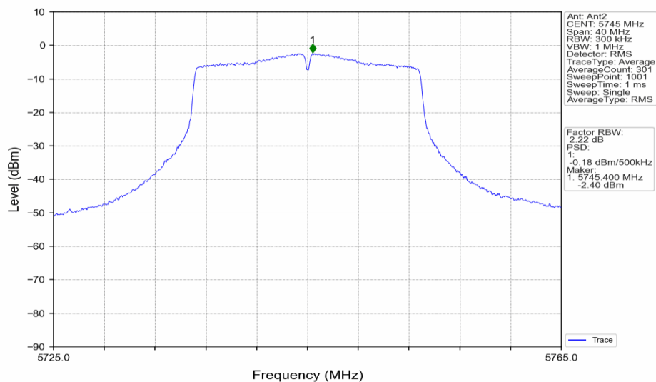
802.11ac(VHT20)_LCH_5745MHz_MIMO_NTNV
