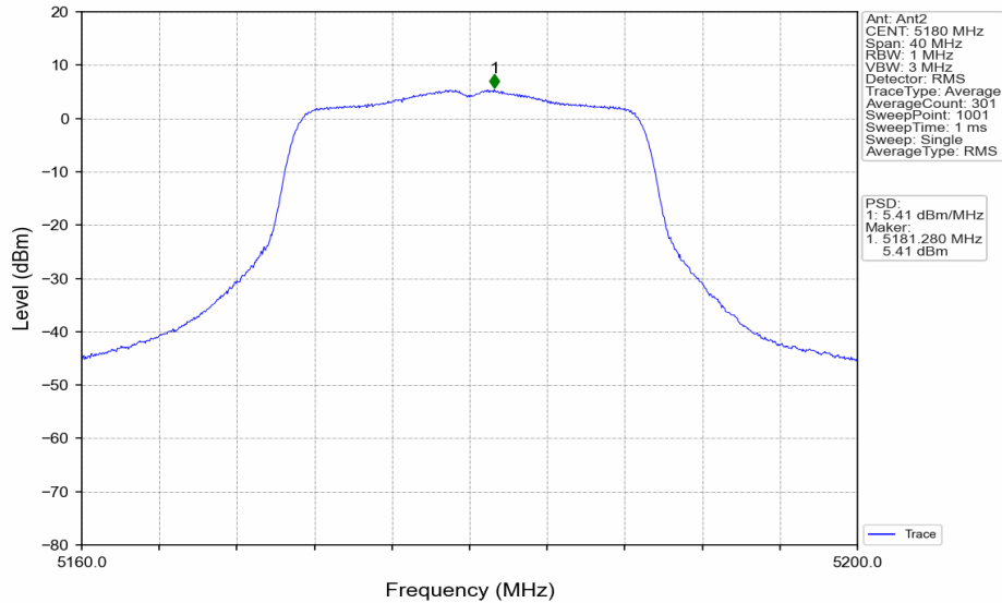
802.11ac(VHT20)_LCH_5180MHz_MIMO_NTNV
