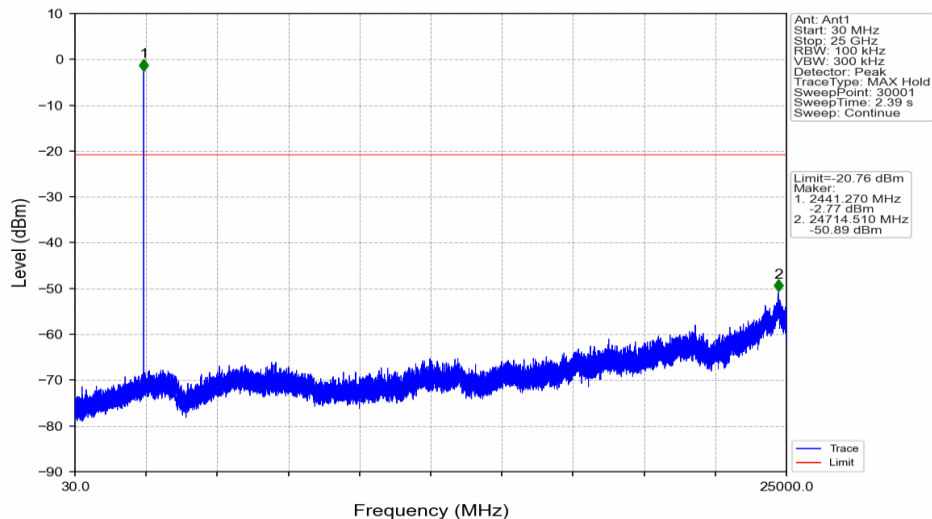
Pi/4DQPSK_2DH5_MCH_2441MHz_Ant1_NTNV
