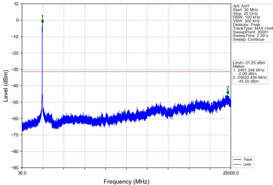
60MHz_HCH_2442.5MHz_Ant1_NTNV
