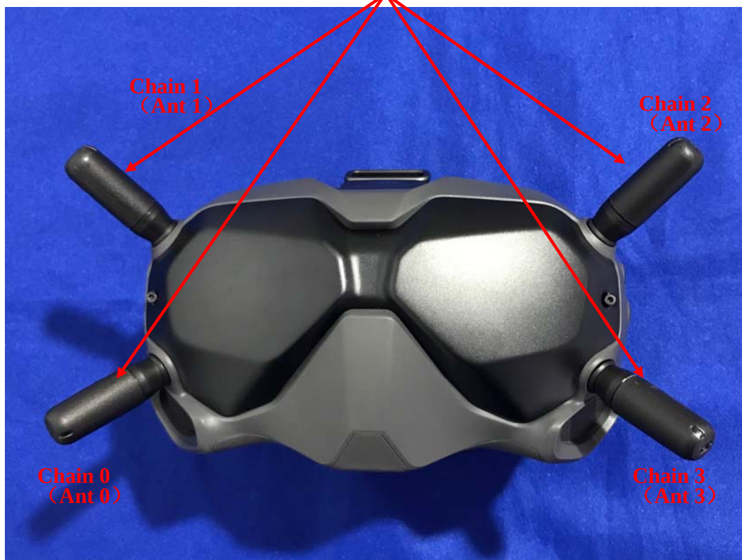
Antennas port
