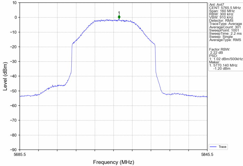
80M_LCH_5765.5MHz_MIMO_NTNV
