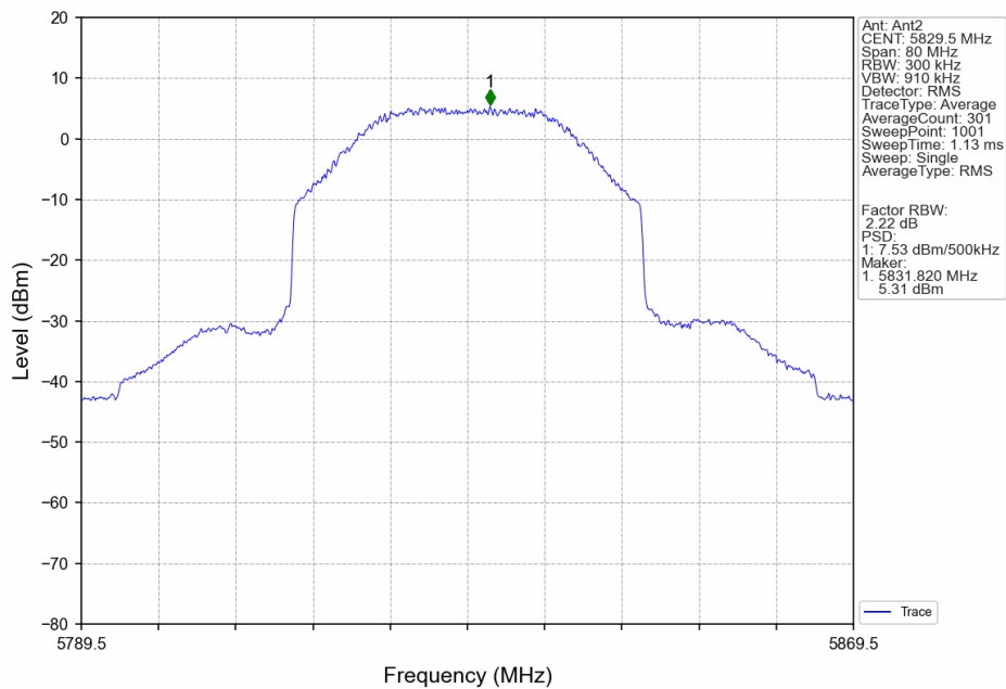
40M_HCH_5829.5MHz_Ant2_NTNV
