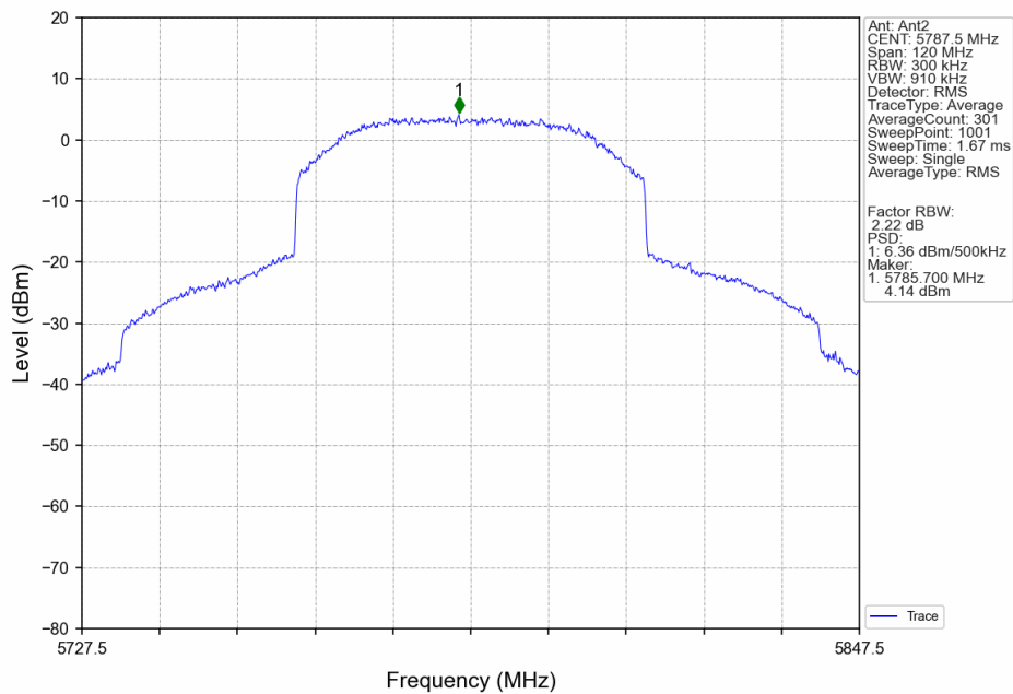
60M_MCH_5787.5MHz_Ant2_NTNV
