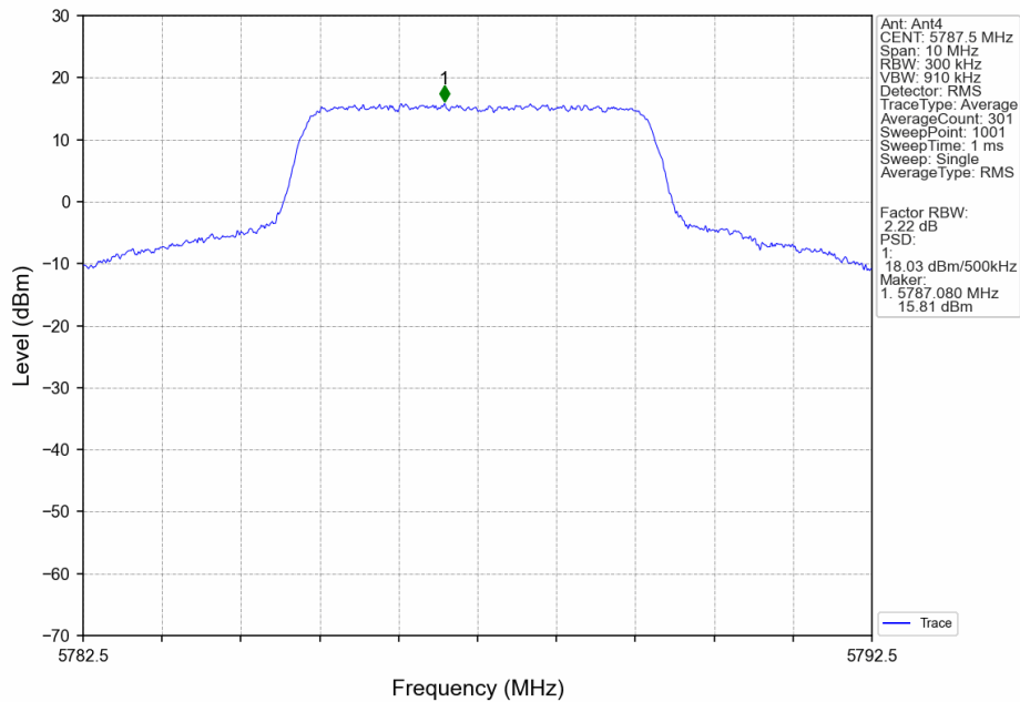
5M_MCH_5787.5MHz_Ant4_NTNV
