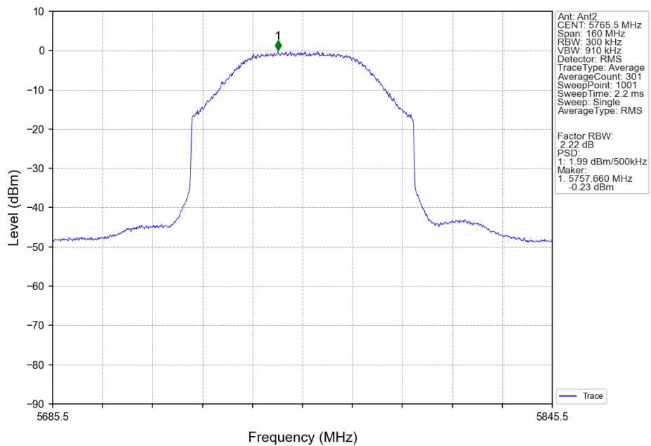
80M_LCH_5765.5MHz_Ant2_NTNV
