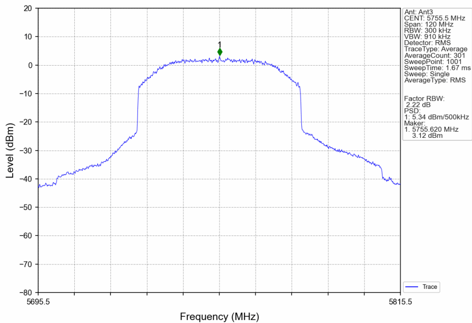
60M_LCH_5755.5MHz_Ant3_NTNV
