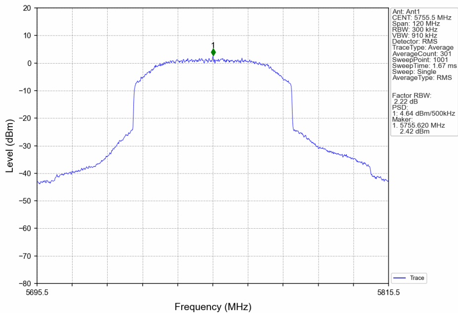
60M_LCH_5755.5MHz_Ant1_NTNV
