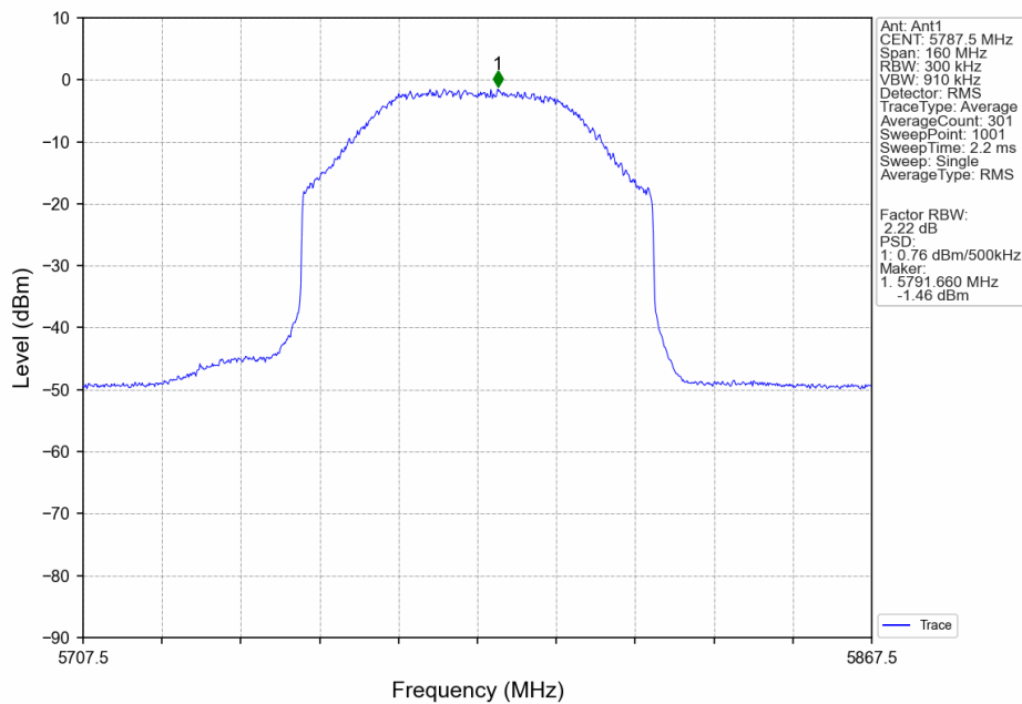
80M_MCH_5787.5MHz_Ant1_NTNV
