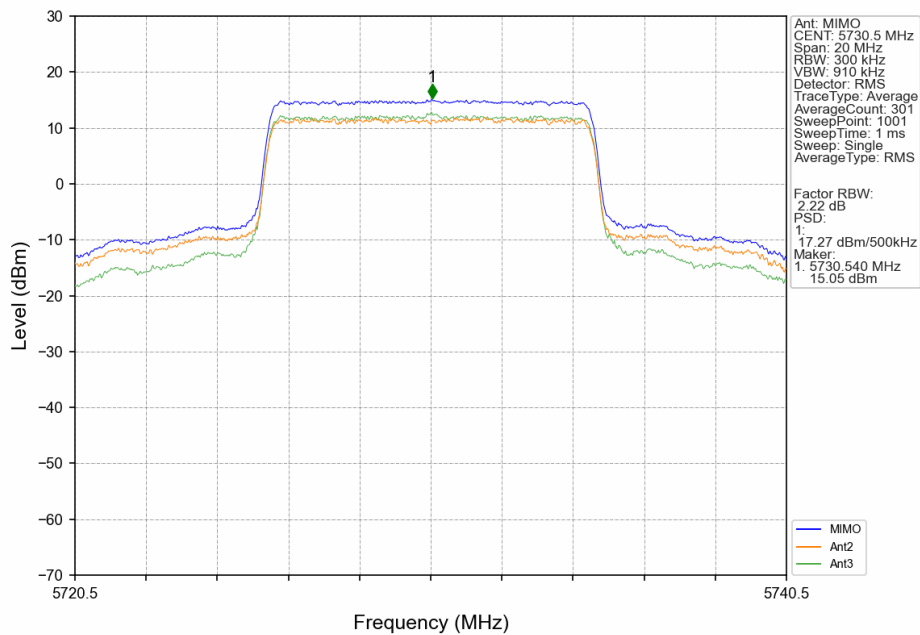
10M_LCH_5730.5MHz_MIMO_NTNV
