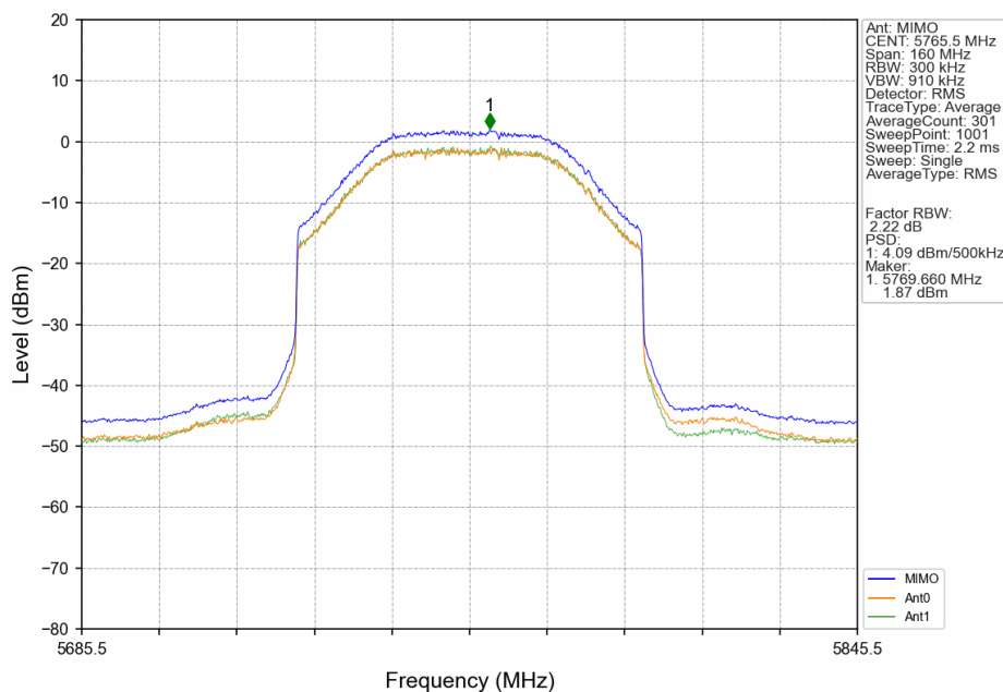
80M_LCH_5765.5MHz_MIMO_NTNV
