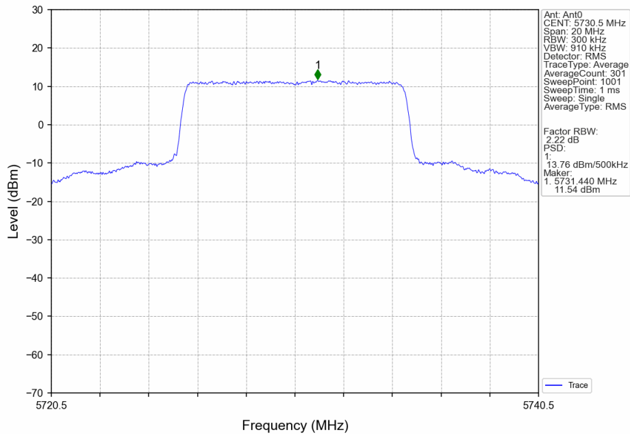
10M_LCH_5730.5MHz_Ant0_NTNV
