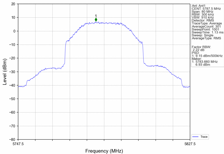
40M_MCH_5787.5MHz_Ant1_NTNV
