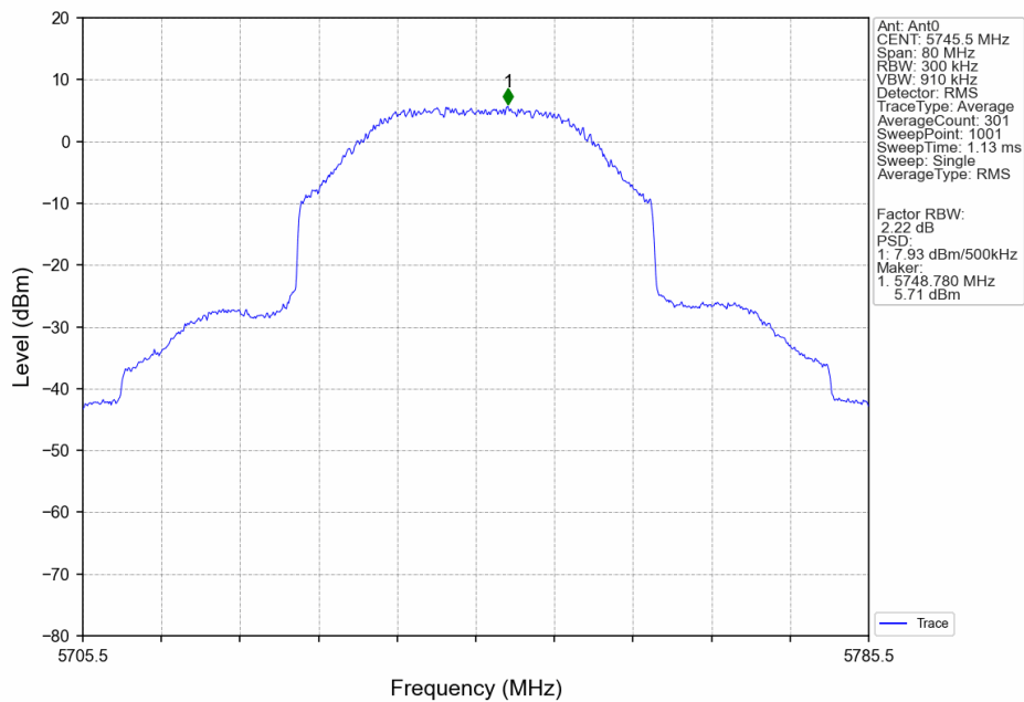
40M_LCH_5745.5MHz_Ant0_NTNV
