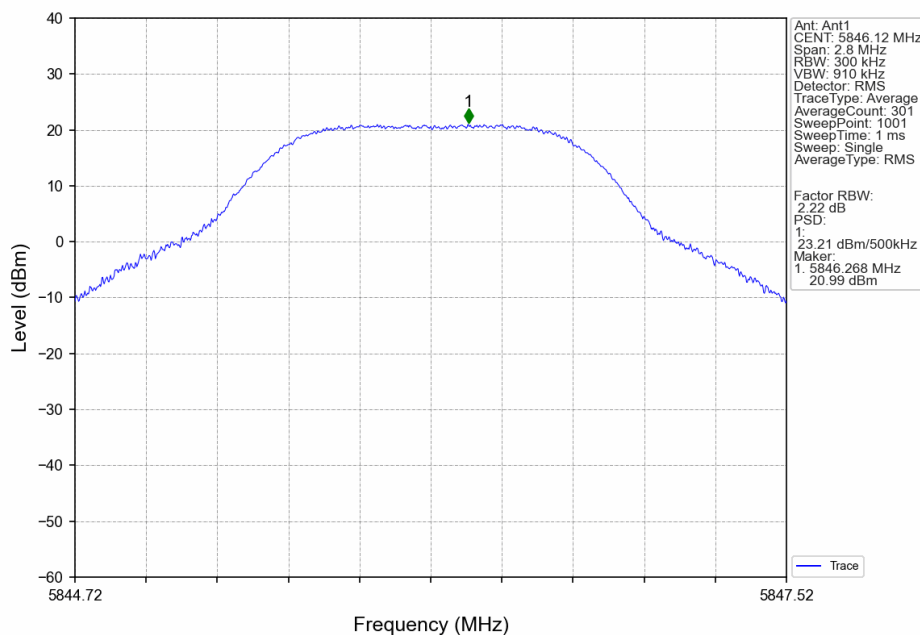
1.4M_HCH_5846.12MHz_Ant1_NTNV
