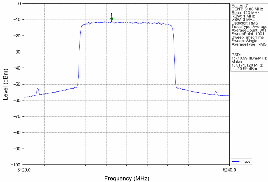
60M_LCH_5180MHz_MIMO_NTNV
