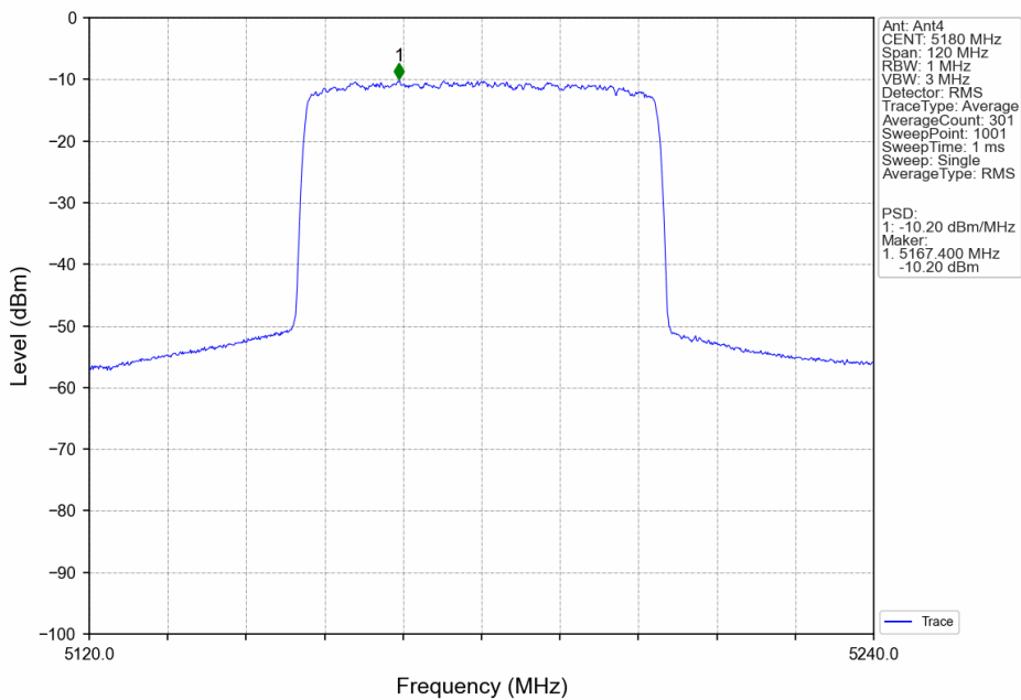
60M_LCH_5180MHz_Ant4_NTNV
