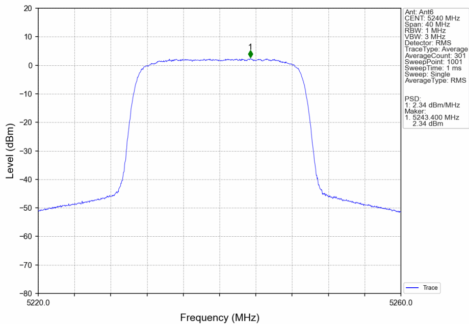
20M_HCH_5240MHz_Ant6_NTNV
