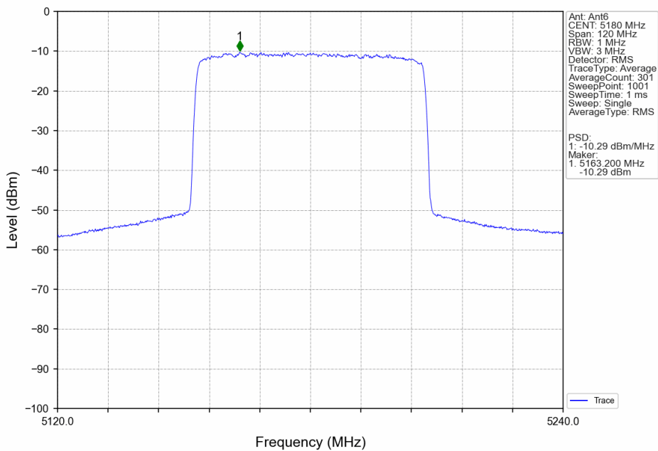
60M_LCH_5180MHz_Ant6_NTNV
