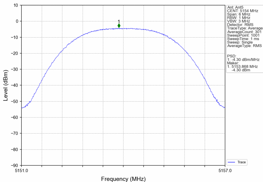
3M_LCH_5154MHz_Ant5_NTNV
