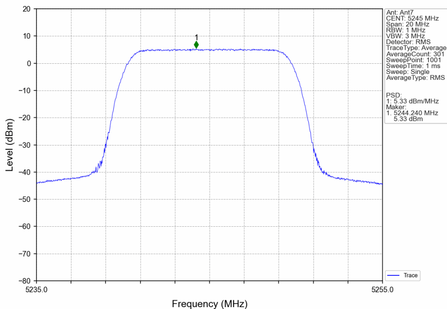
10M_HCH_5245MHz_Ant7_NTNV
