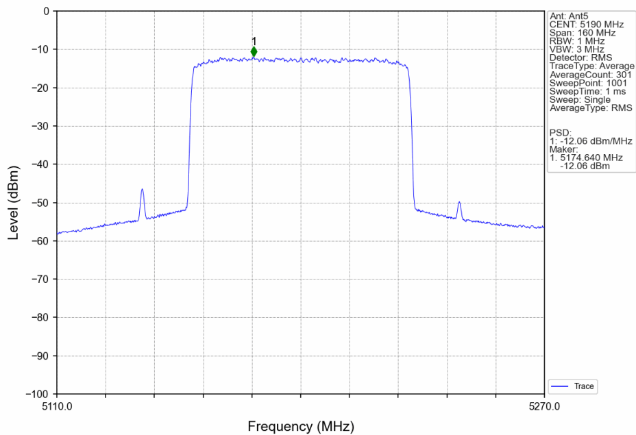
80M_LCH_5190MHz_Ant5_NTNV
