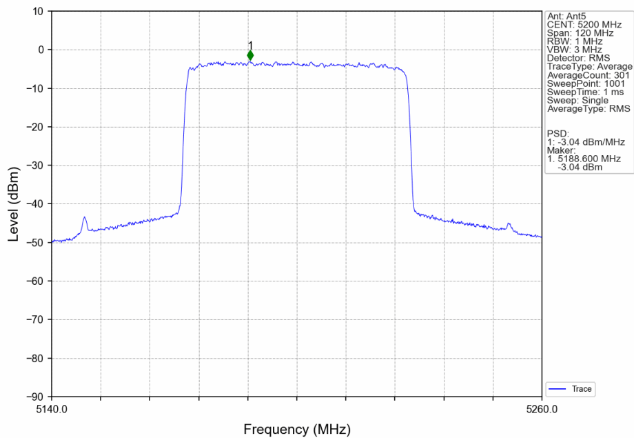
60M_MCH_5200MHz_Ant5_NTNV
