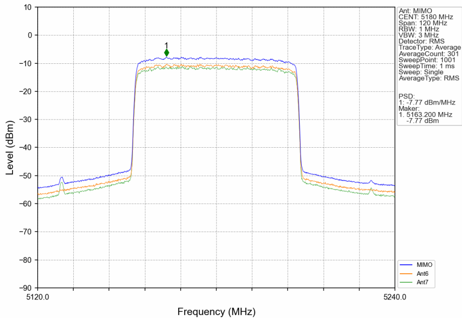
60M_LCH_5180MHz_MIMO_NTNV
