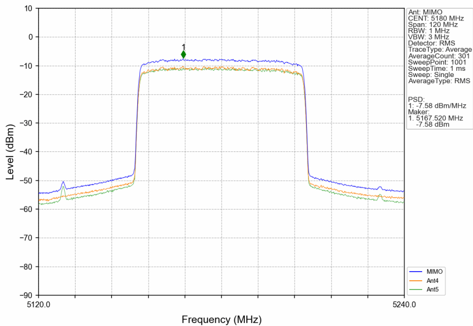
60M_LCH_5180MHz_MIMO_NTNV
