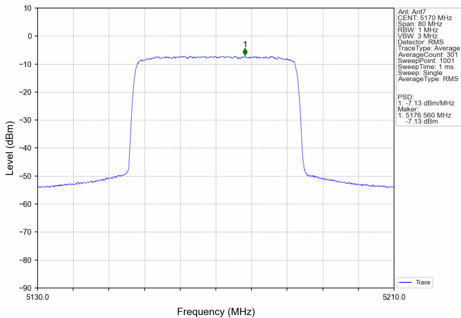
40M_LCH_5170MHz_Ant7_NTNV
