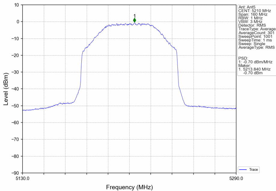
80M_HCH_5210MHz_Ant5_NTNV
