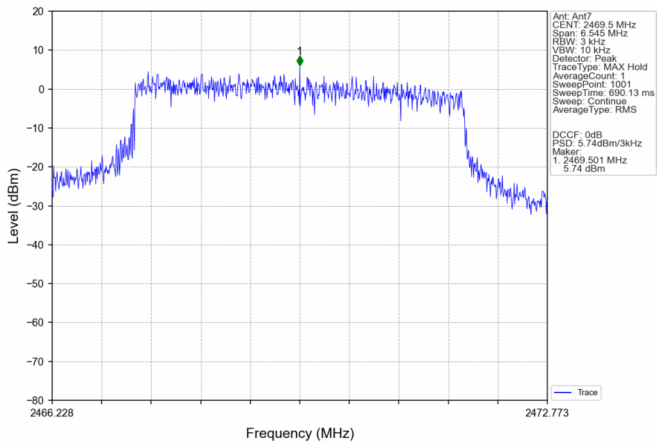
5M_HCH_2469.5MHz_Ant7_NTNV
