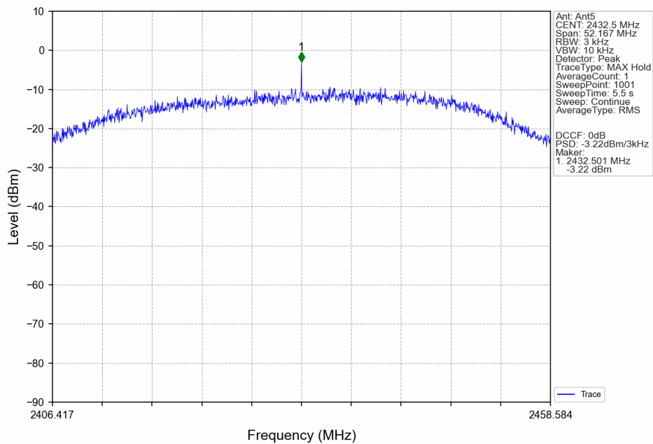
60M_LCH_2432.5MHz_Ant5_NTNV
