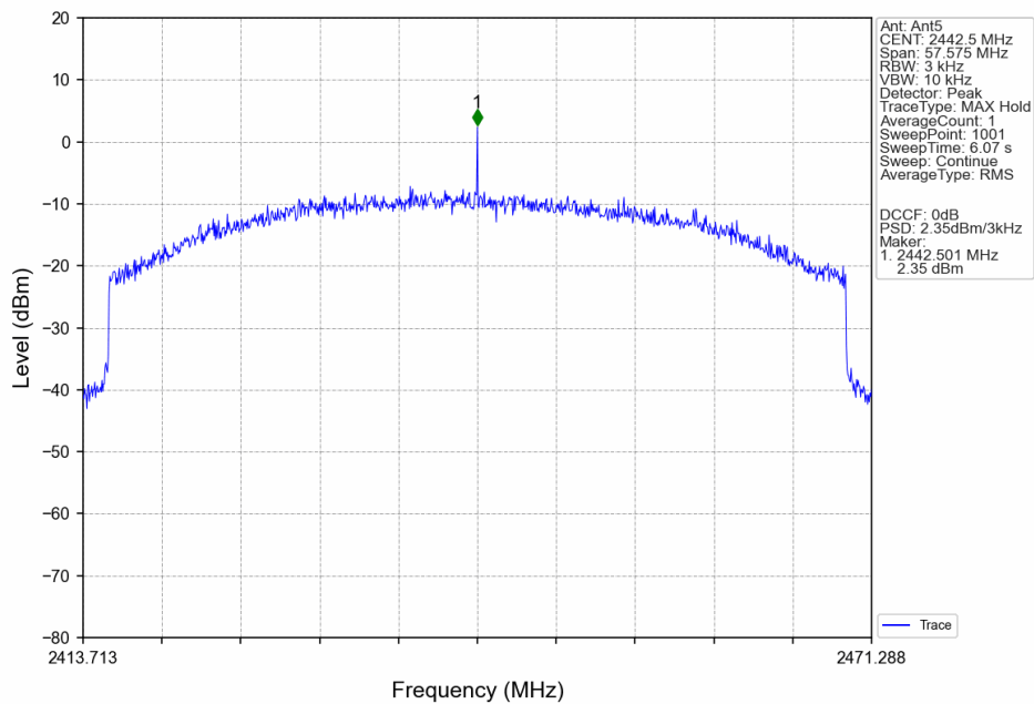
60M_HCH_2442.5MHz_Ant5_NTNV
