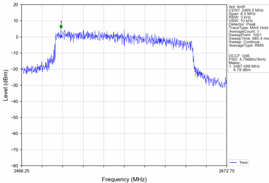
5M_HCH_2469.5MHz_Ant5_NTNV
