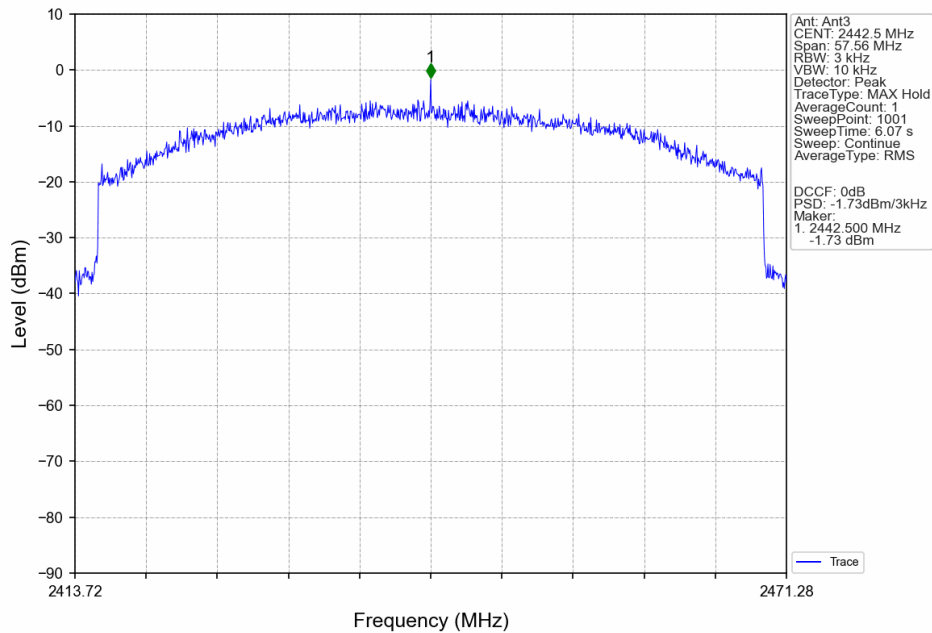
60M_HCH_2442.5MHz_Ant3_NTNV
