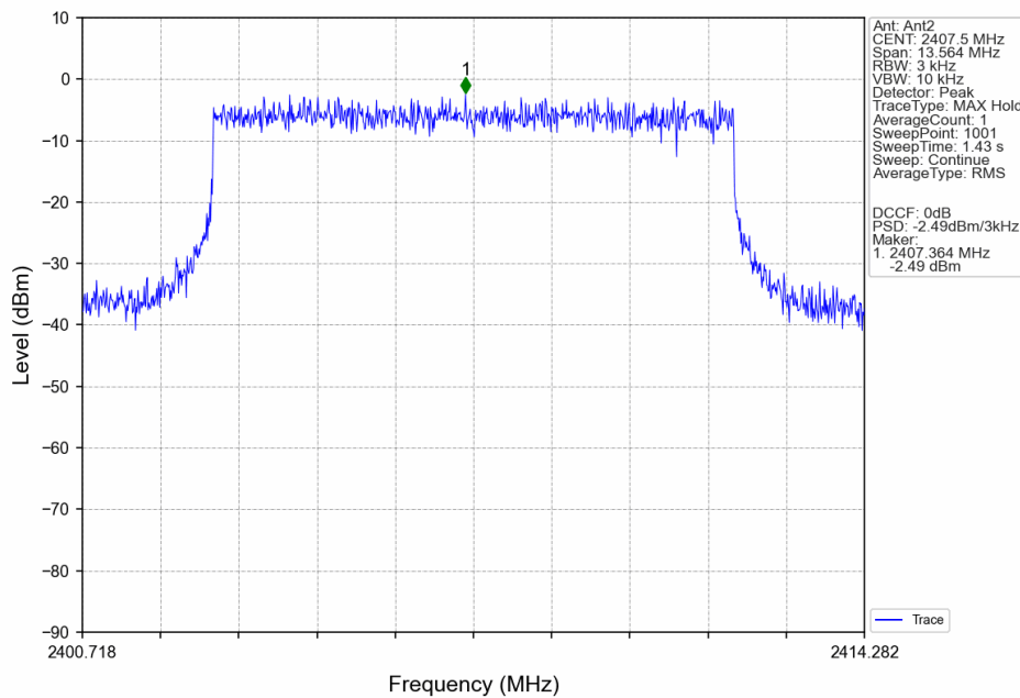
10M_LCH_2407.5MHz_Ant2_NTNV
