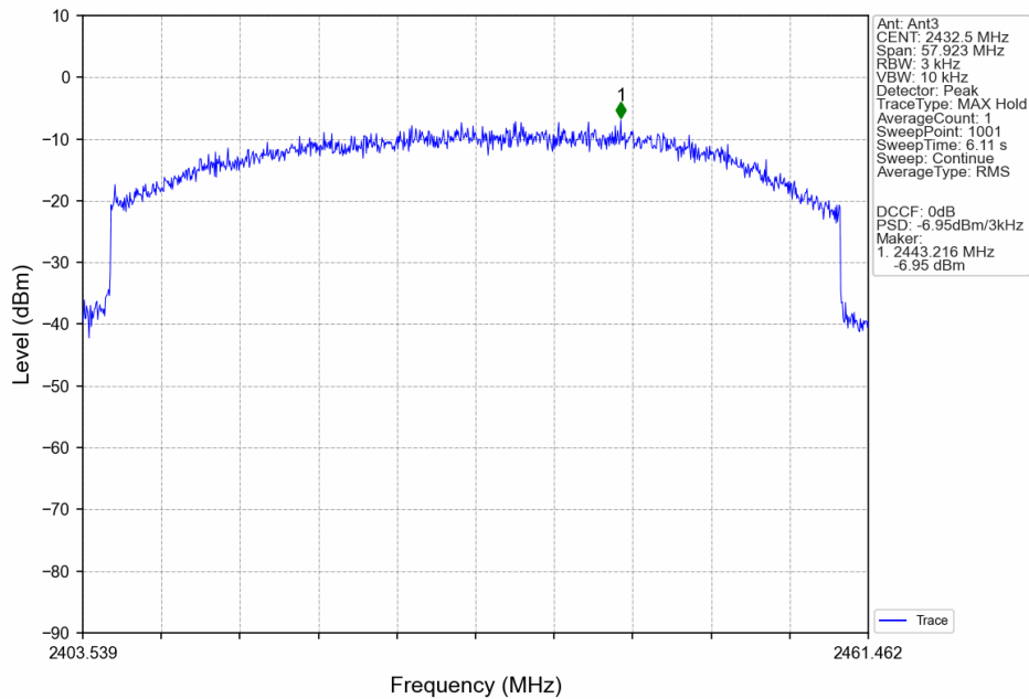
60M_LCH_2432.5MHz_Ant3_NTNV
