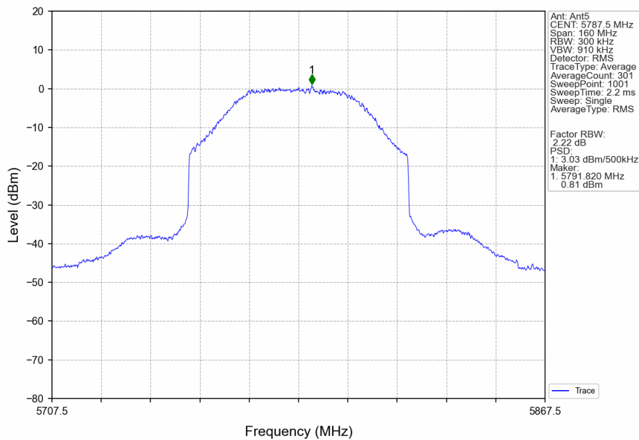
80M_MCH_5787.5MHz_Ant5_NTNV
