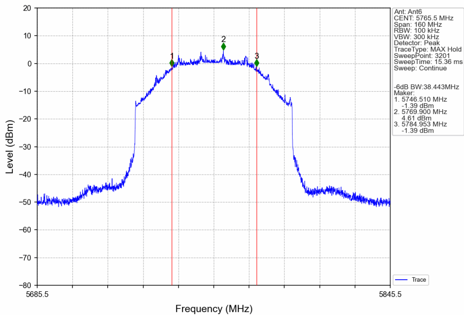
80M_LCH_5765.5MHz_Ant6_NTNV
