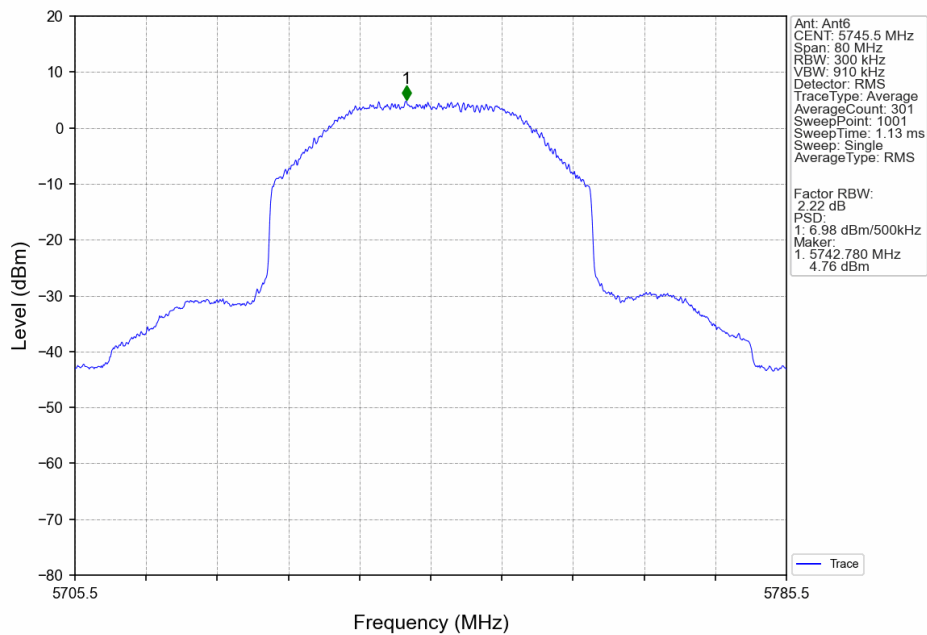
40M_LCH_5745.5MHz_Ant6_NTNV
