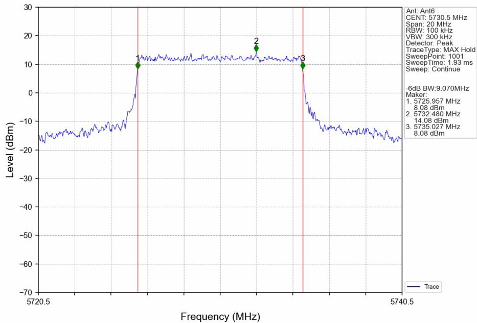
10M_LCH_5730.5MHz_Ant6_NTNV
