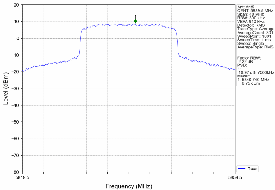
20M_HCH_5839.5MHz_Ant5_NTNV
