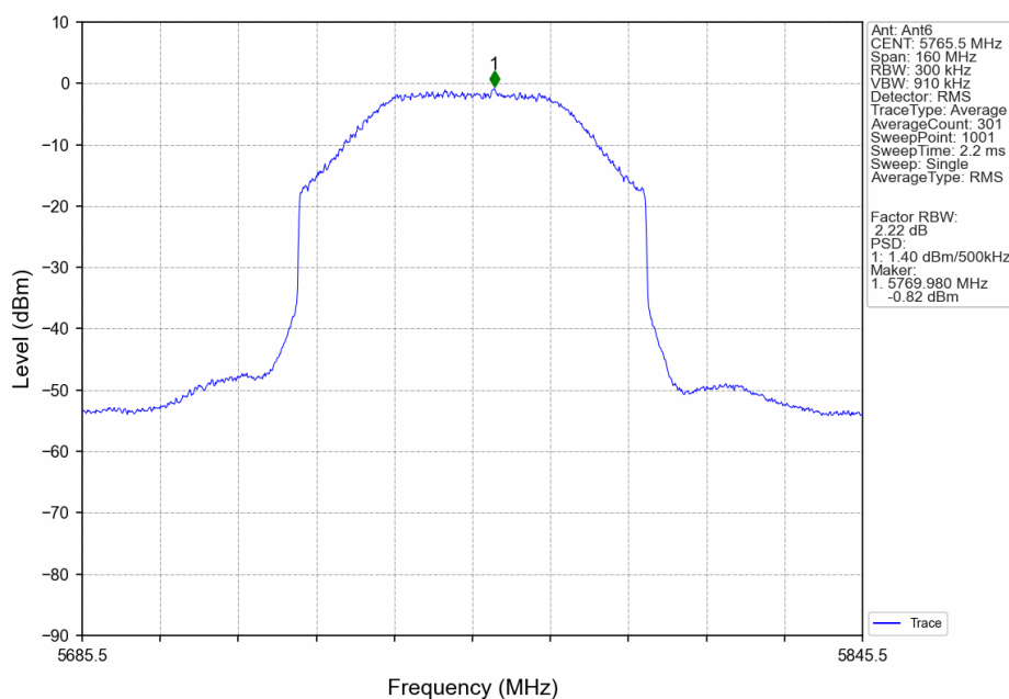
80M_LCH_5765.5MHz_Ant6_NTNV
