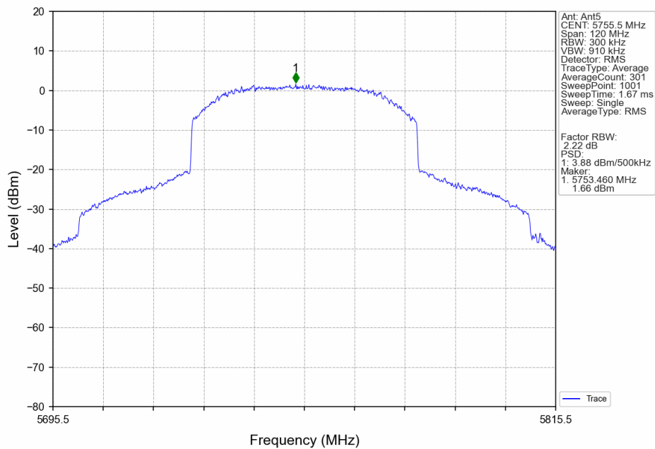
60M_LCH_5755.5MHz_Ant5_NTNV
