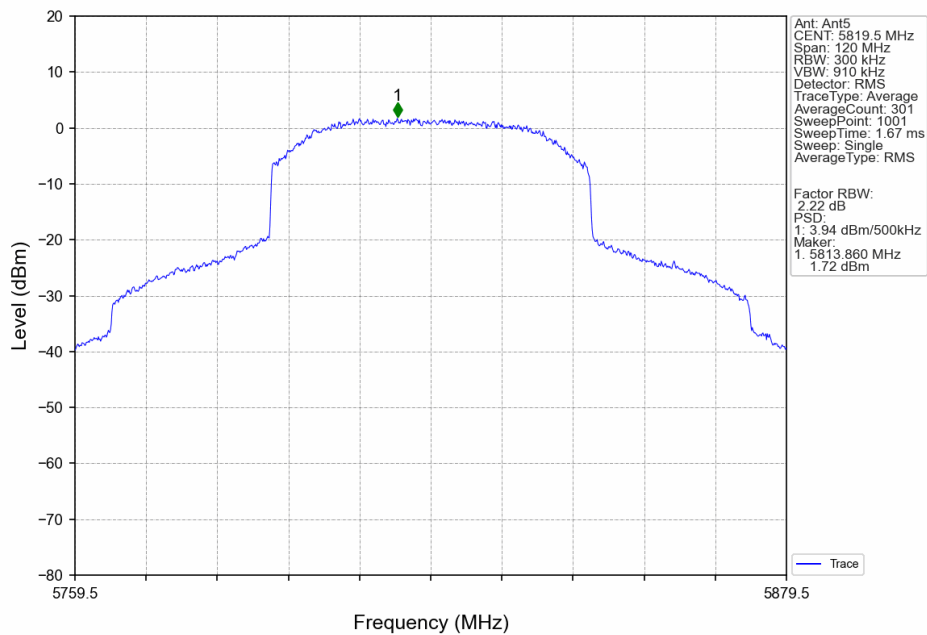
60M_HCH_5819.5MHz_Ant5_NTNV
