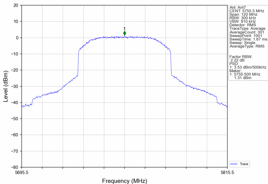
60M_LCH_5755.5MHz_Ant7_NTNV
