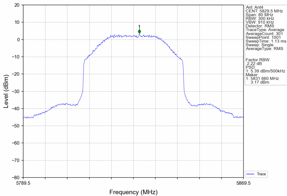
40M_HCH_5829.5MHz_Ant4_NTNV
