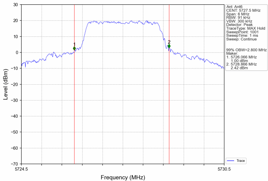
3M_LCH_5727.5MHz_Ant6_NTNV
