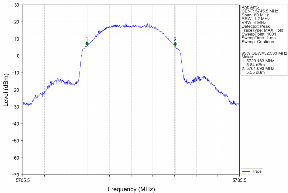
40M_LCH_5745.5MHz_Ant6_NTNV
