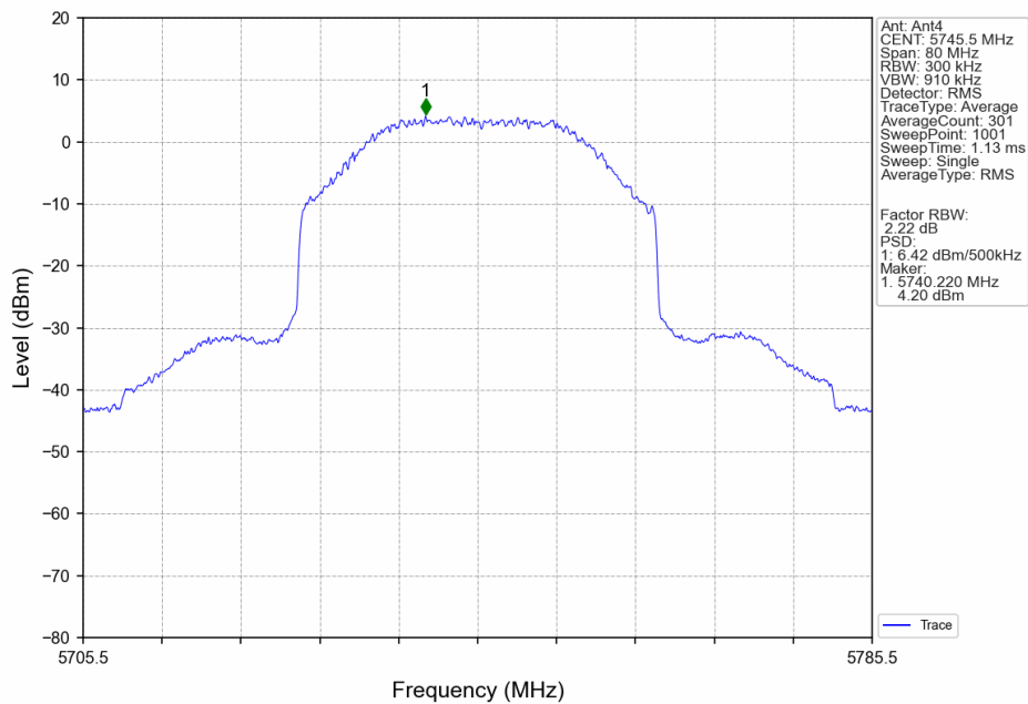
40M_LCH_5745.5MHz_Ant4_NTNV
