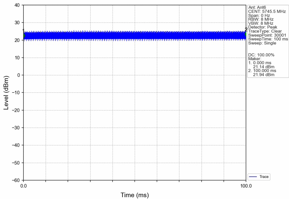
40M_LCH_5745.5MHz_Ant6_NTNV
