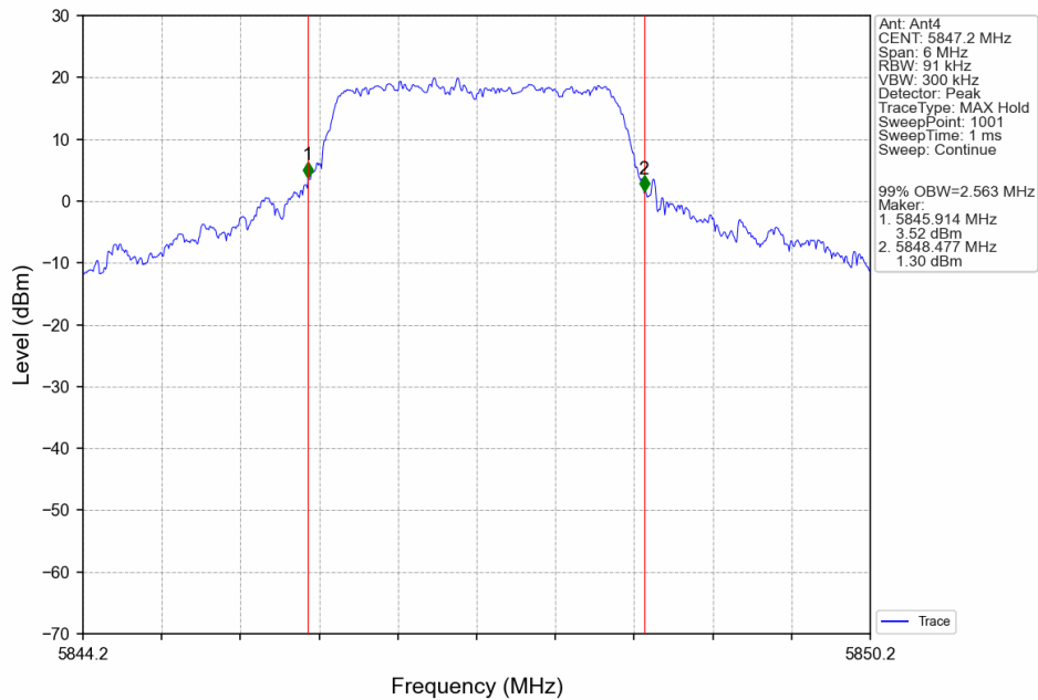
3M_HCH_5847.2MHz_Ant4_NTNV
