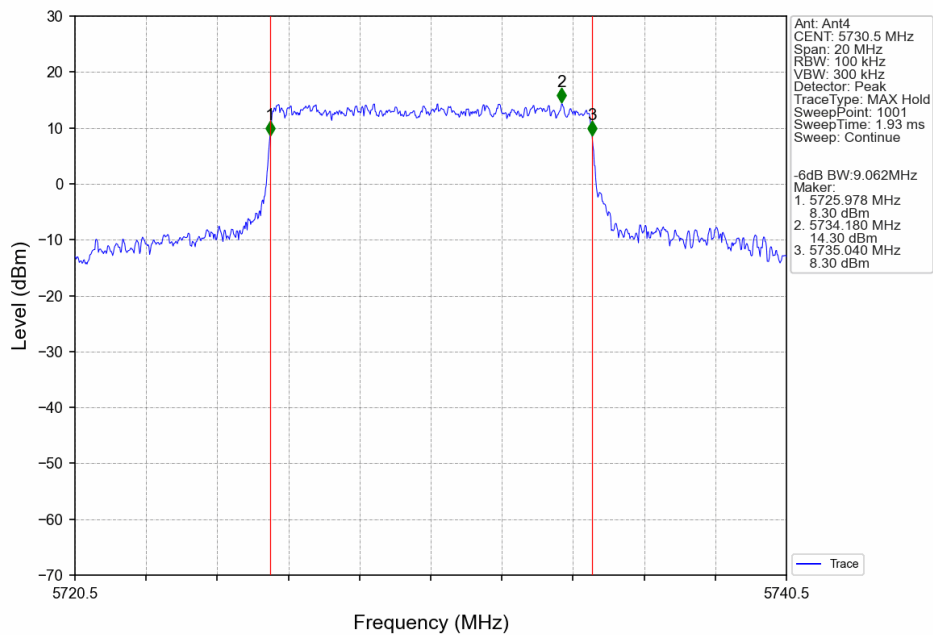
10M_LCH_5730.5MHz_Ant4_NTNV
