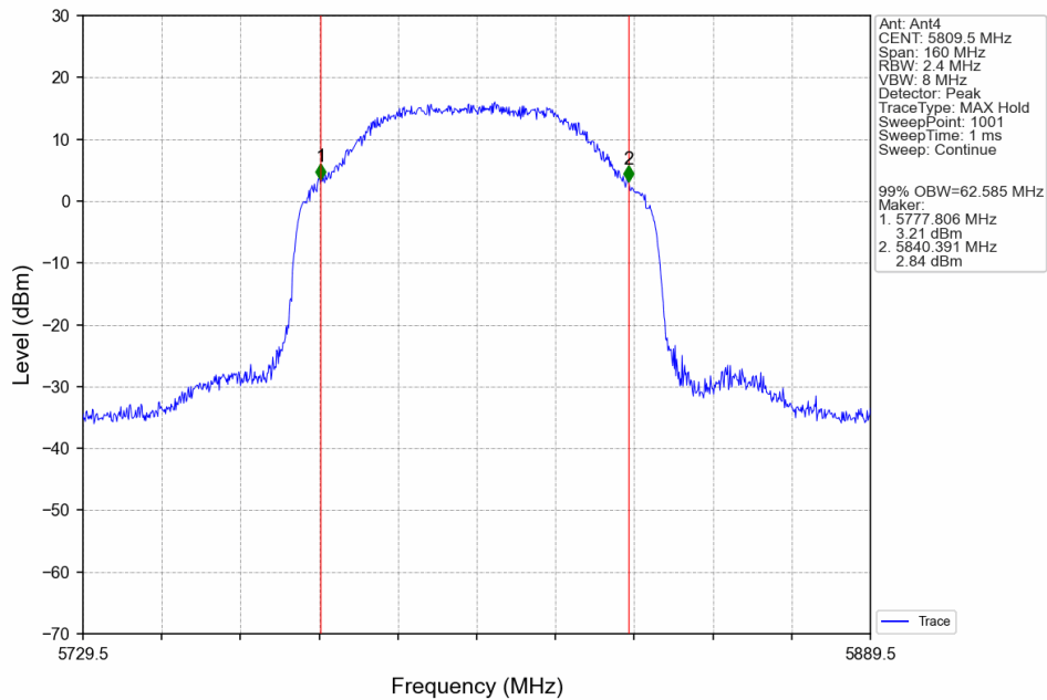
80M_HCH_5809.5MHz_Ant4_NTNV
