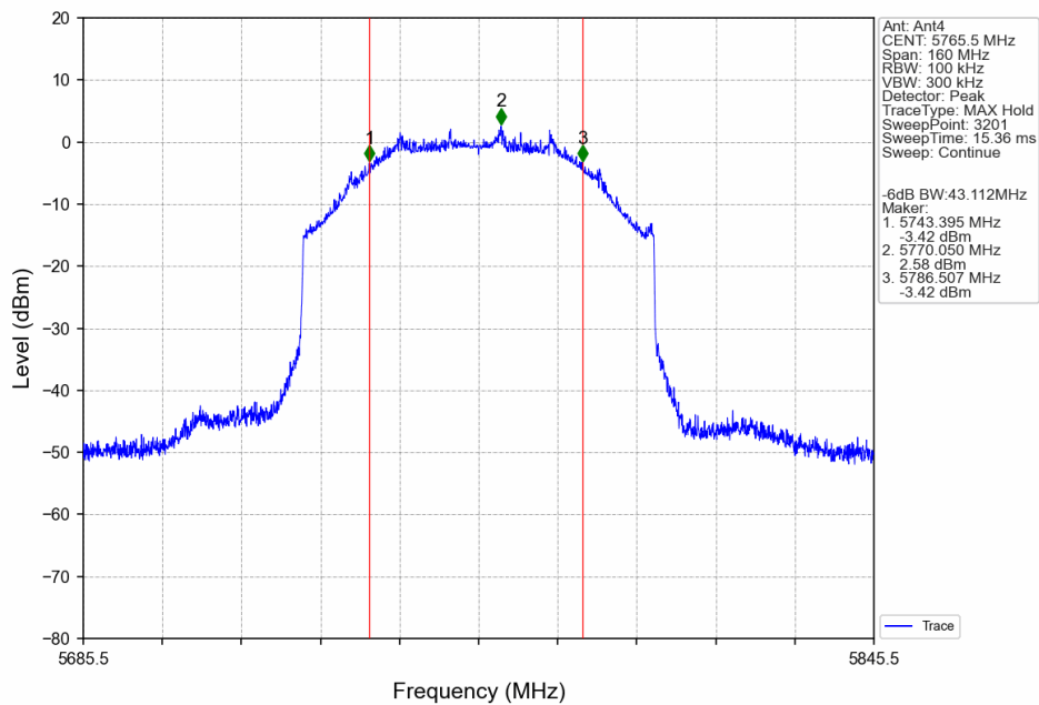
80M_LCH_5765.5MHz_Ant4_NTNV
