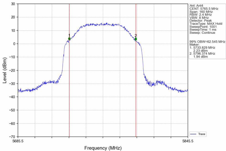
80M_LCH_5765.5MHz_Ant4_NTNV
