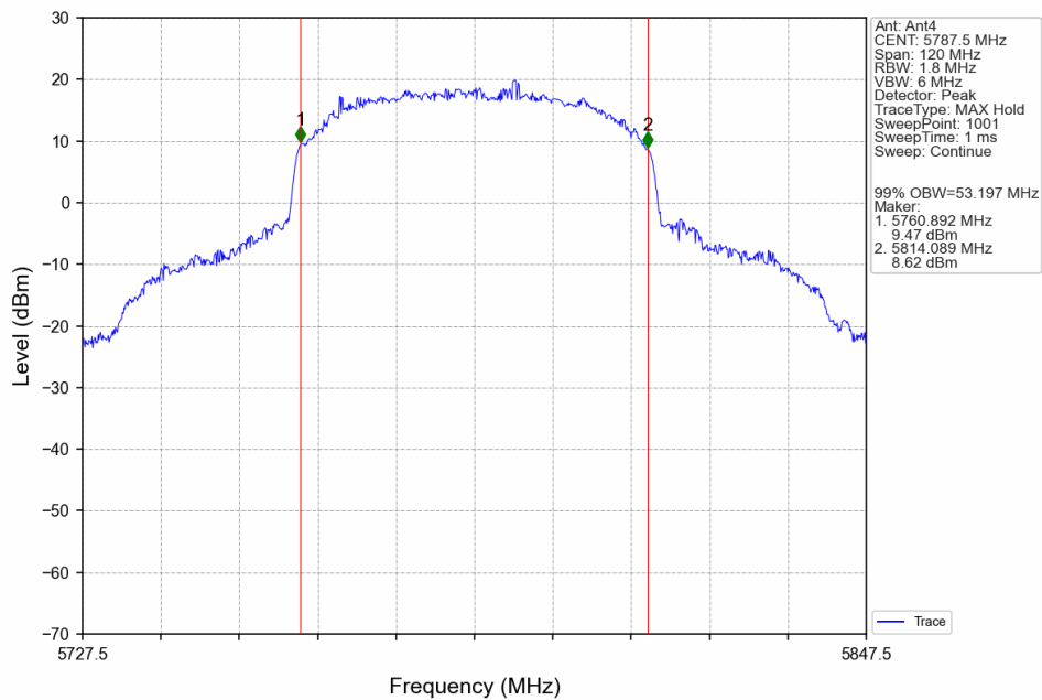
60M_MCH_5787.5MHz_Ant4_NTNV
