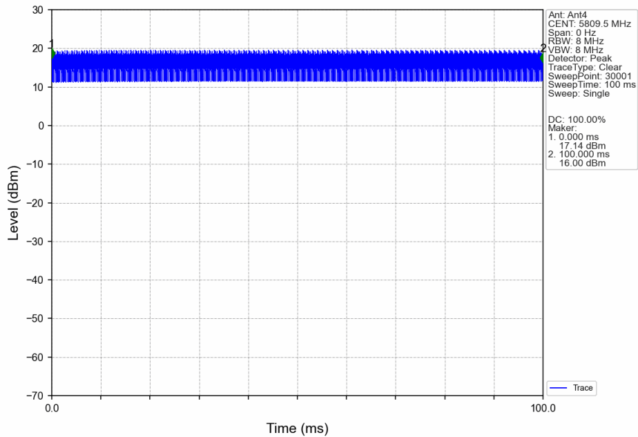
80M_HCH_5809.5MHz_Ant4_NTNV
