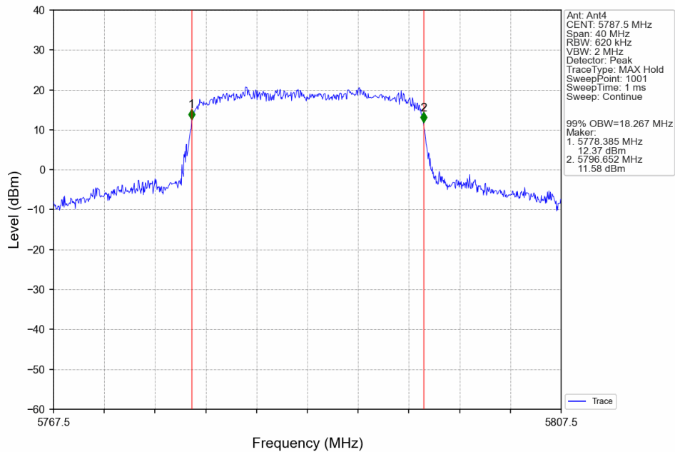
20M_MCH_5787.5MHz_Ant4_NTNV
