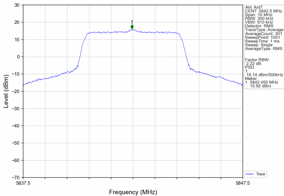
5M_HCH_5842.5MHz_Ant7_NTNV
