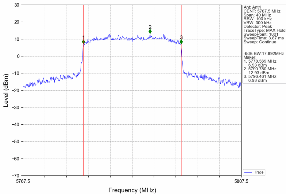
20M_MCH_5787.5MHz_Ant4_NTNV
