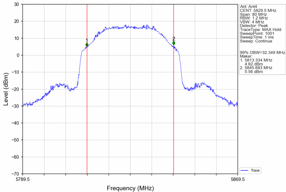
40M_HCH_5829.5MHz_Ant4_NTNV
