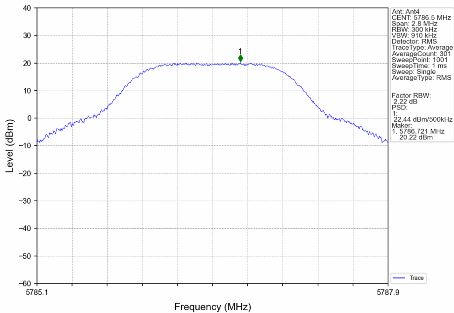
1.4M_MCH_5786.5MHz_Ant4_NTNV
