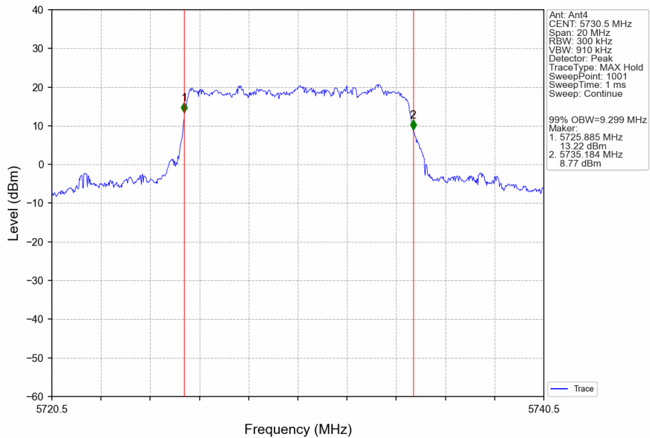
10M_LCH_5730.5MHz_Ant4_NTNV
