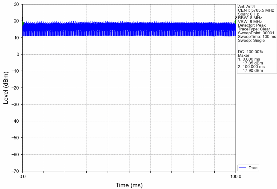
80M_LCH_5765.5MHz_Ant4_NTNV
