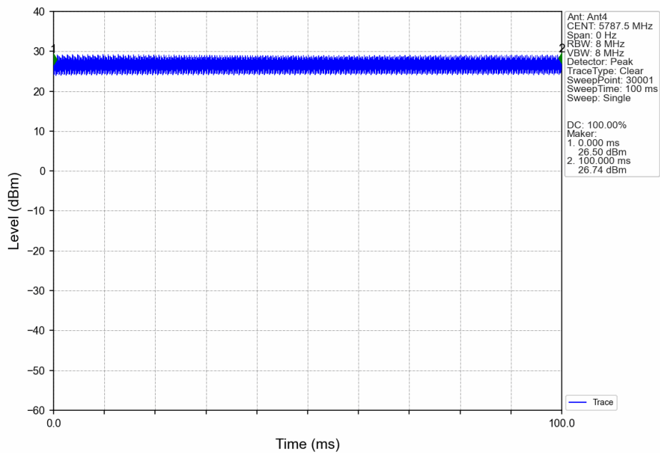
20M_MCH_5787.5MHz_Ant4_NTNV
