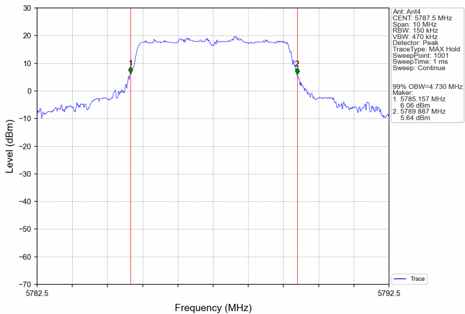
5M_MCH_5787.5MHz_Ant4_NTNV
