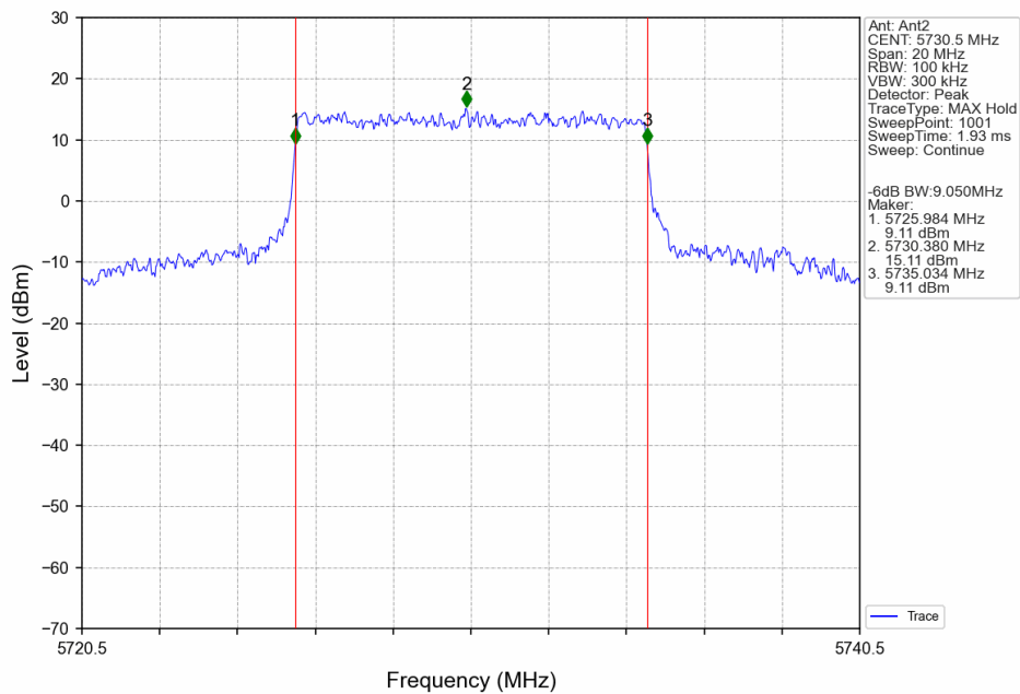
10M_LCH_5730.5MHz_Ant2_NTNV
