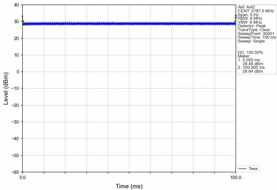
5M_MCH_5787.5MHz_Ant2_NTNV
