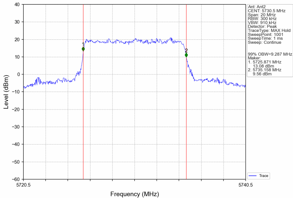
10M_LCH_5730.5MHz_Ant2_NTNV
