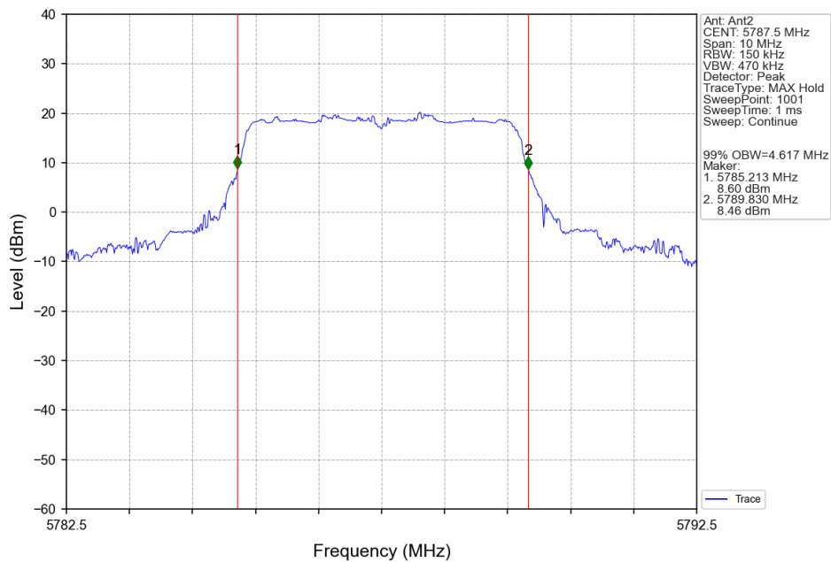
5M_MCH_5787.5MHz_Ant2_NTNV
