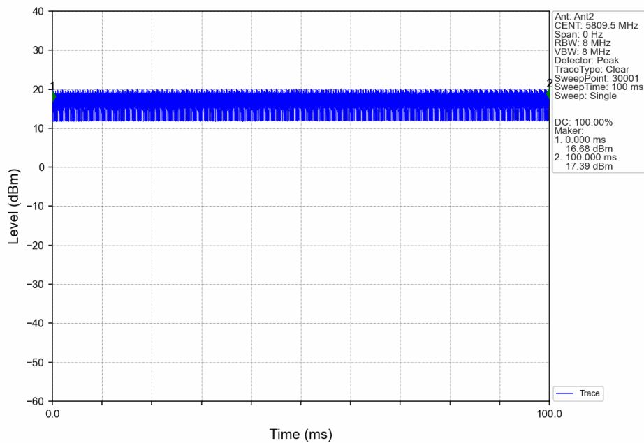
80M_HCH_5809.5MHz_Ant2_NTNV
