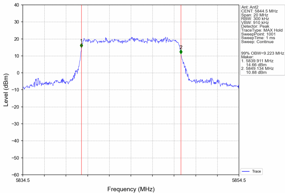
10M_HCH_5844.5MHz_Ant2_NTNV
