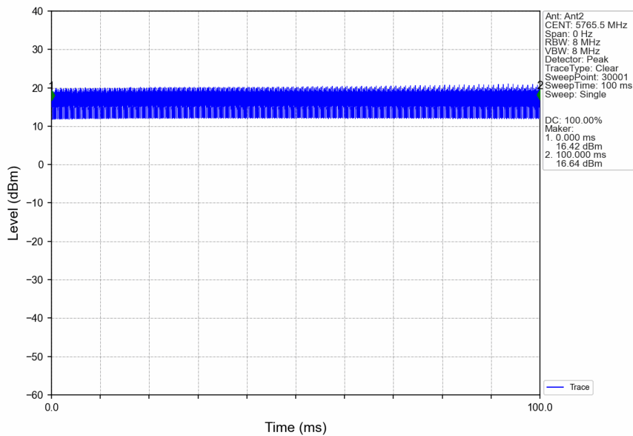
80M_LCH_5765.5MHz_Ant2_NTNV
