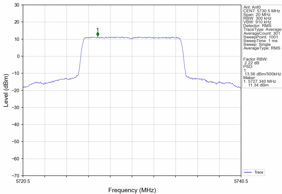
10M_LCH_5730.5MHz_Ant0_NTNV
