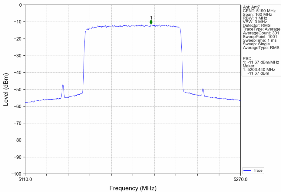
80M_LCH_5190MHz_Ant7_NTNV
