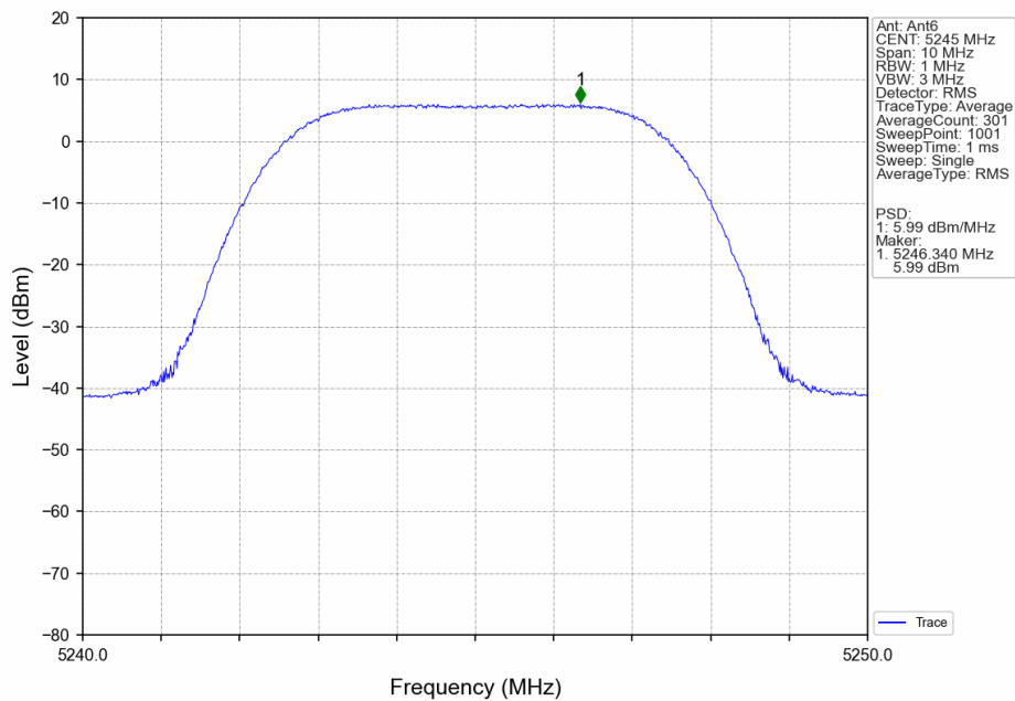
5M_HCH_5245MHz_Ant6_NTNV
