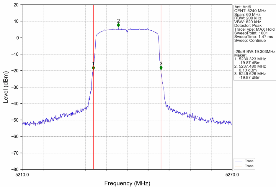
20M_HCH_5240MHz_Ant6_NTNV
