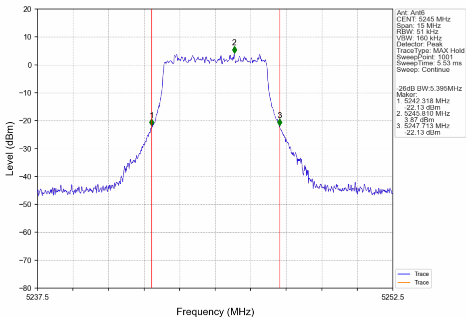
5M_HCH_5245MHz_Ant6_NTNV
