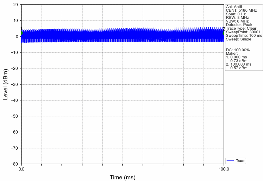
60M_LCH_5180MHz_Ant6_NTNV
