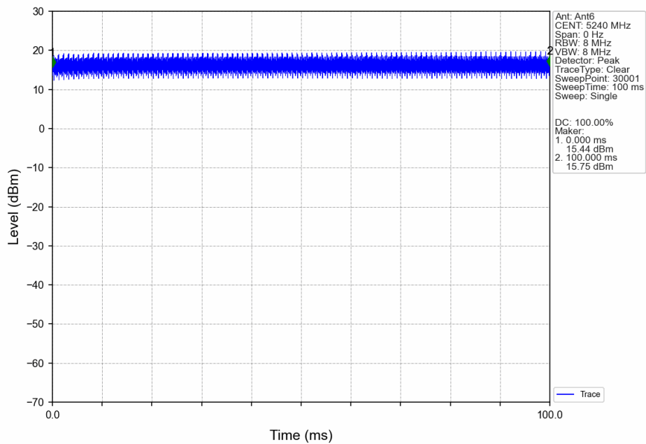
20M_HCH_5240MHz_Ant6_NTNV
