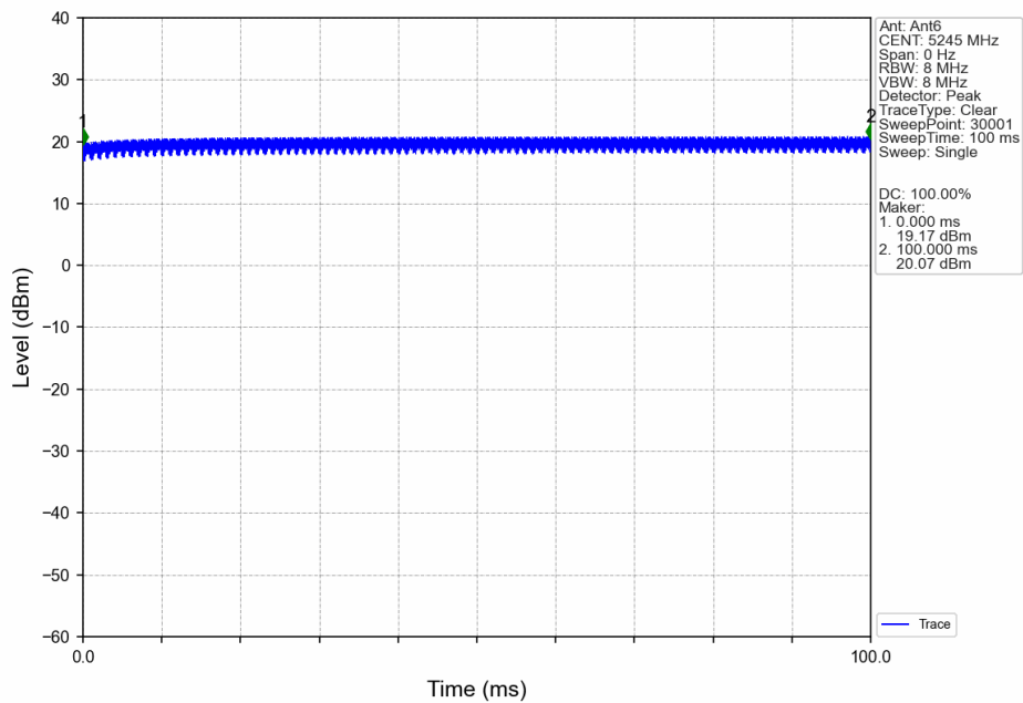
5M_HCH_5245MHz_Ant6_NTNV
