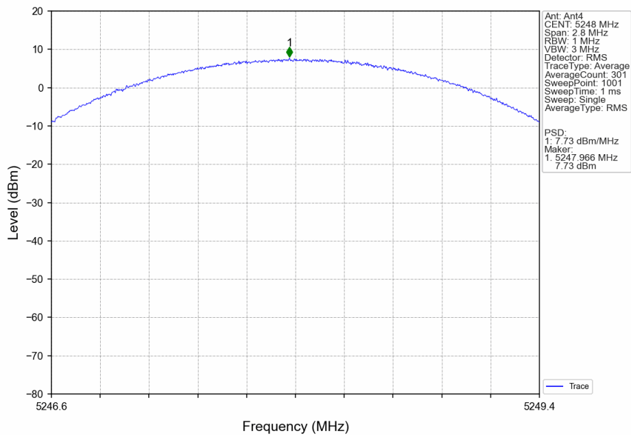
1.4M_HCH_5248MHz_Ant4_NTNV
