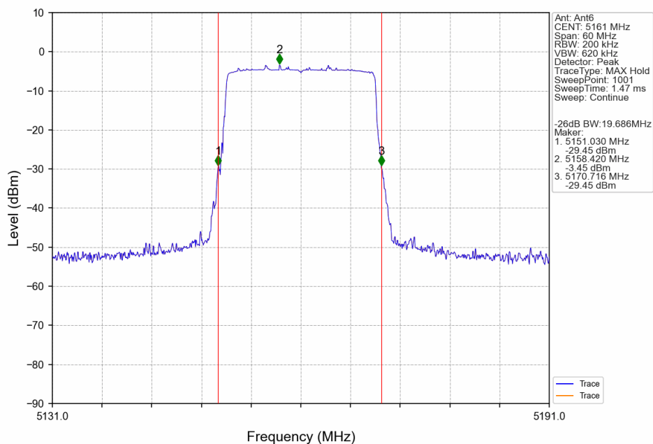
20M_LCH_5161MHz_Ant6_NTNV
